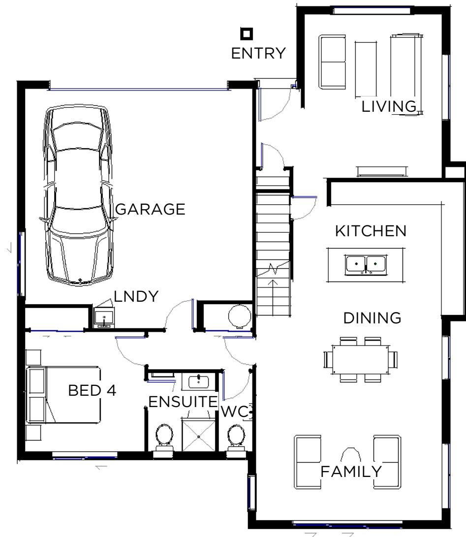
① Lower - Floor Plan - ART 1 : 100
