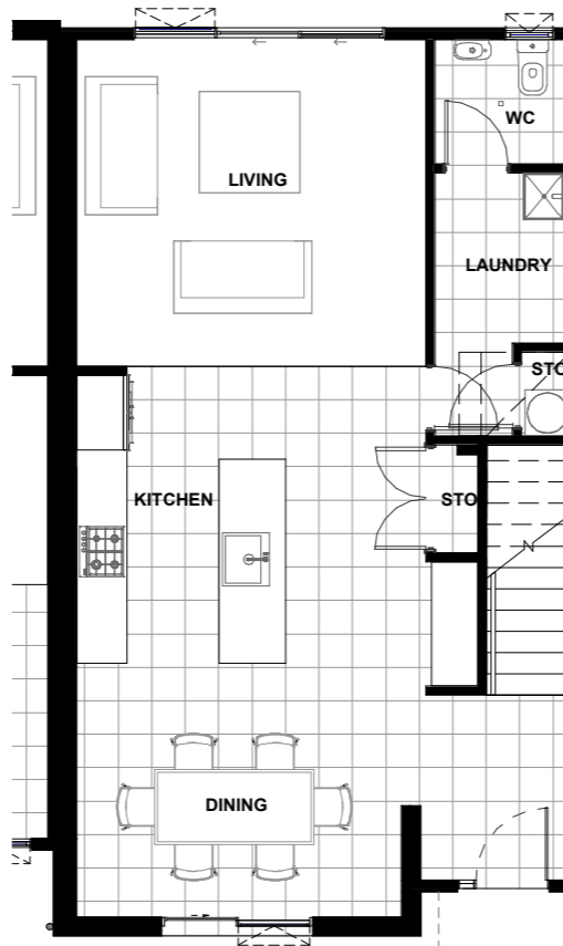
LOT 3044 GROUND FLOOR PLAN
