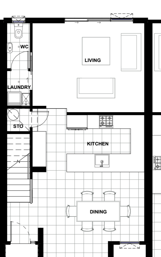
LOT 3043 GROUND FLOOR PLAN
