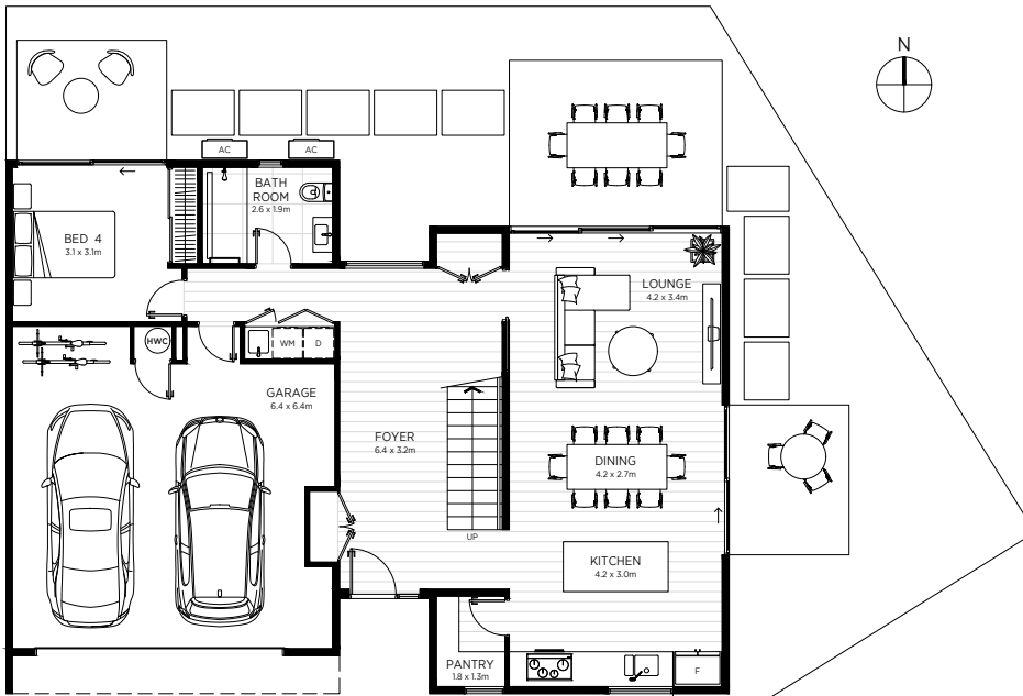
PU20 GROUND FLOOR
