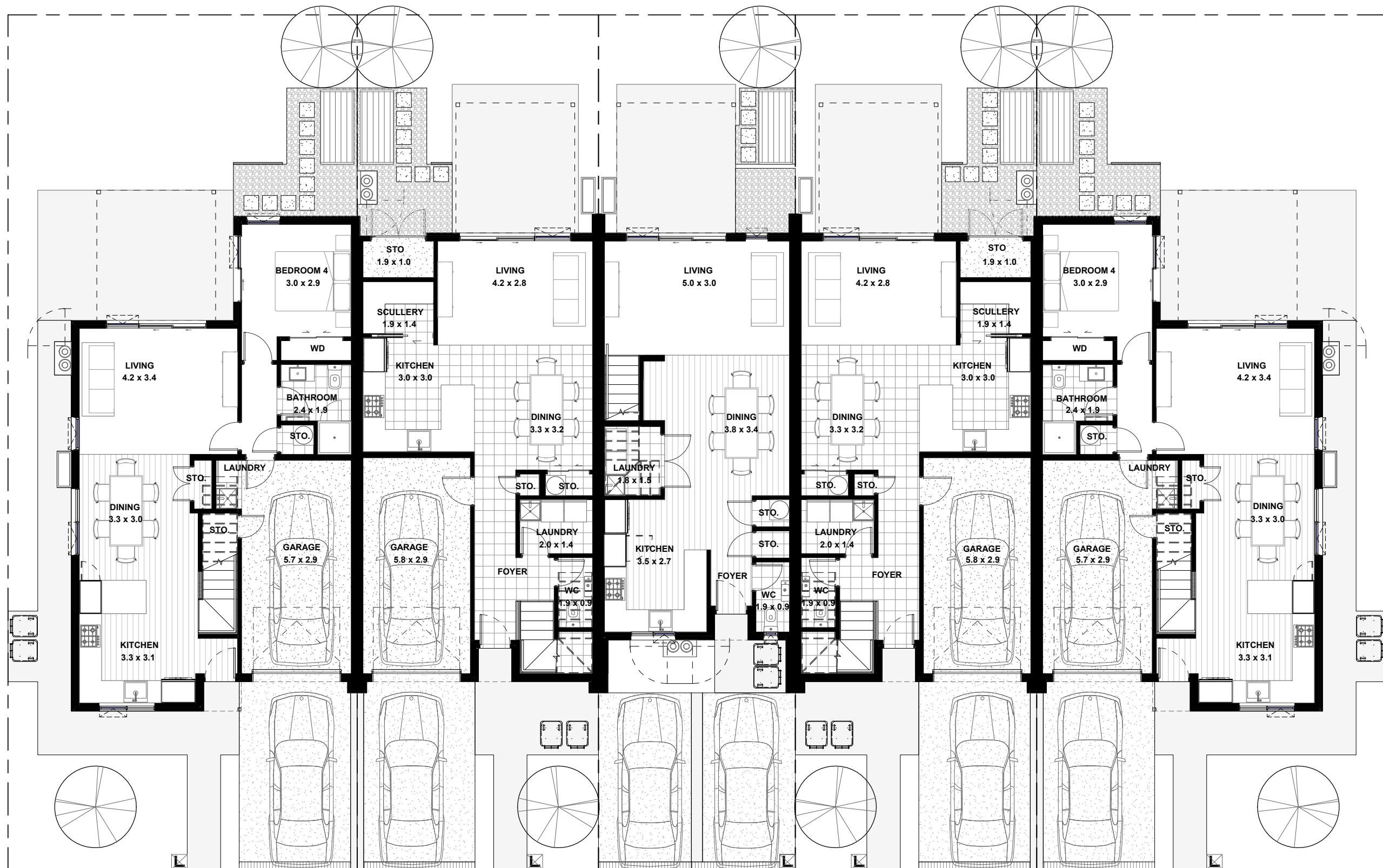
LOT 3065 GROUND FLOOR PLAN
