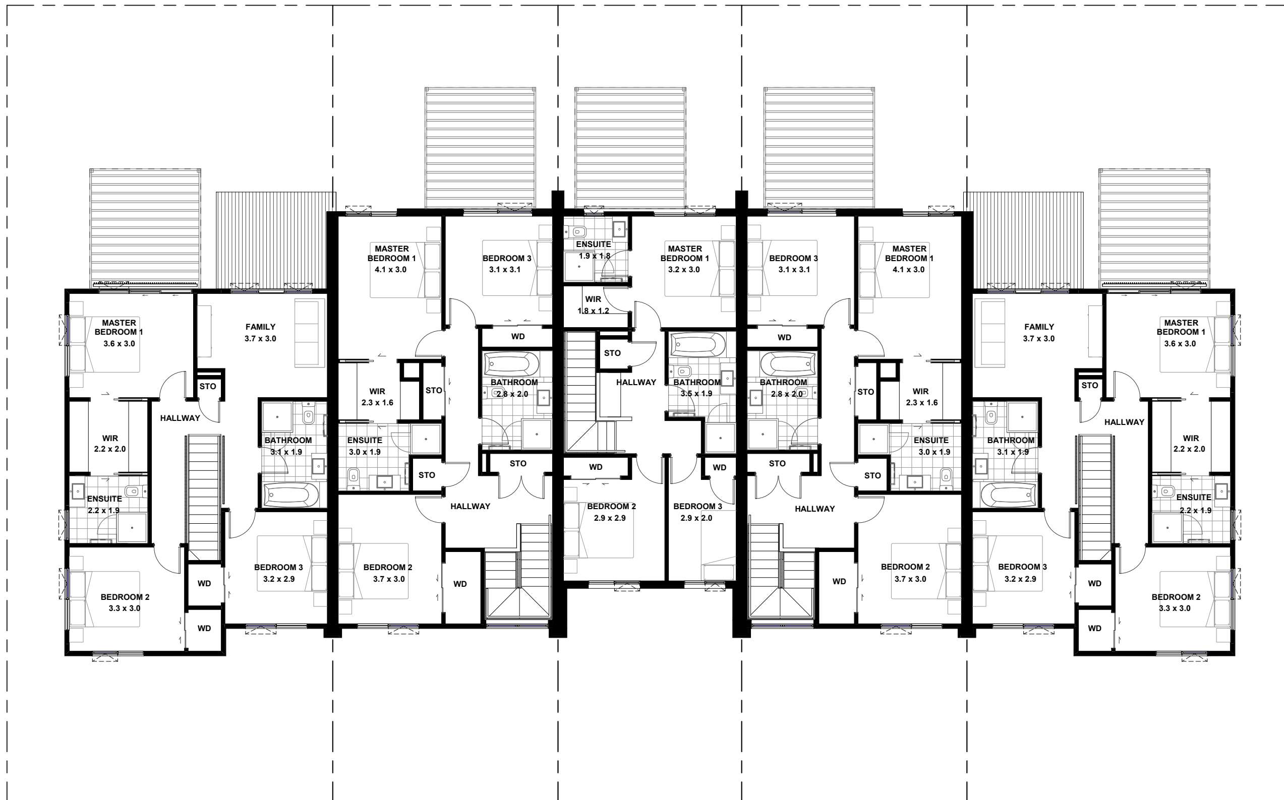
LOT 3065 FIRST FLOOR PLAN 17 Lady McKenzie Mews Floor Area - 162m 2 Site Area - 216m 2
