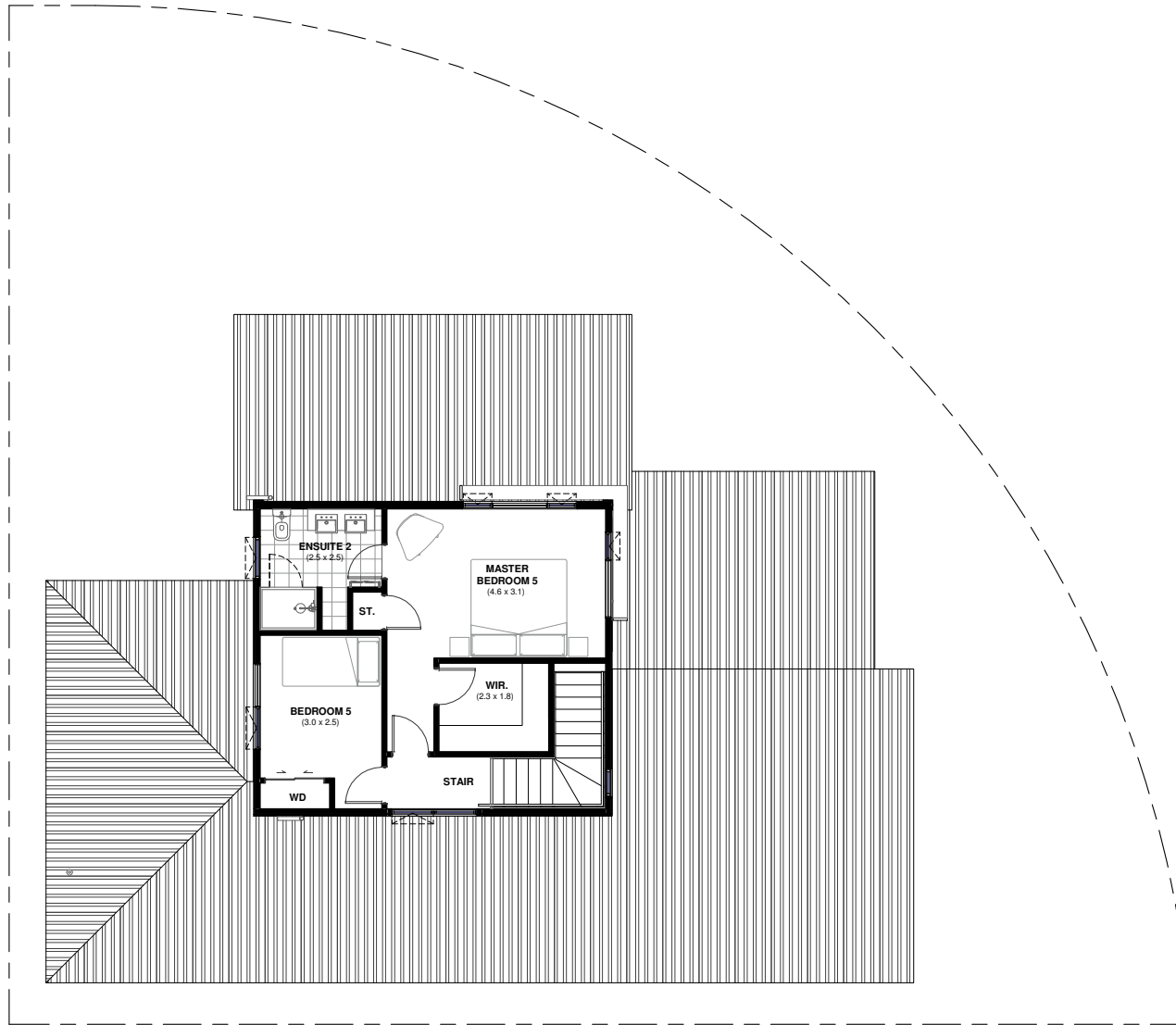
LOT 360 - FIRST FLOOR PLAN
