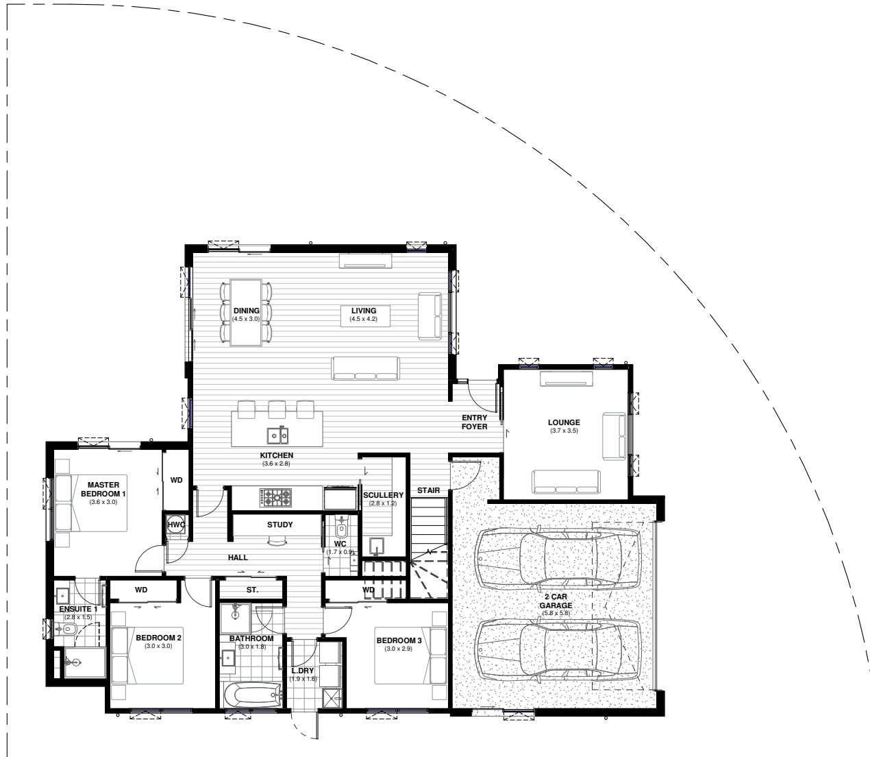
LOT 360 - GROUND FLOOR PLAN
