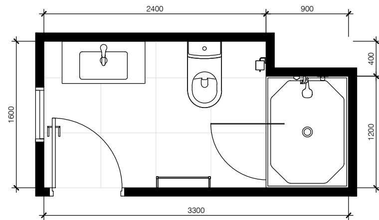
ENSUITE - GROUND FLOOR
