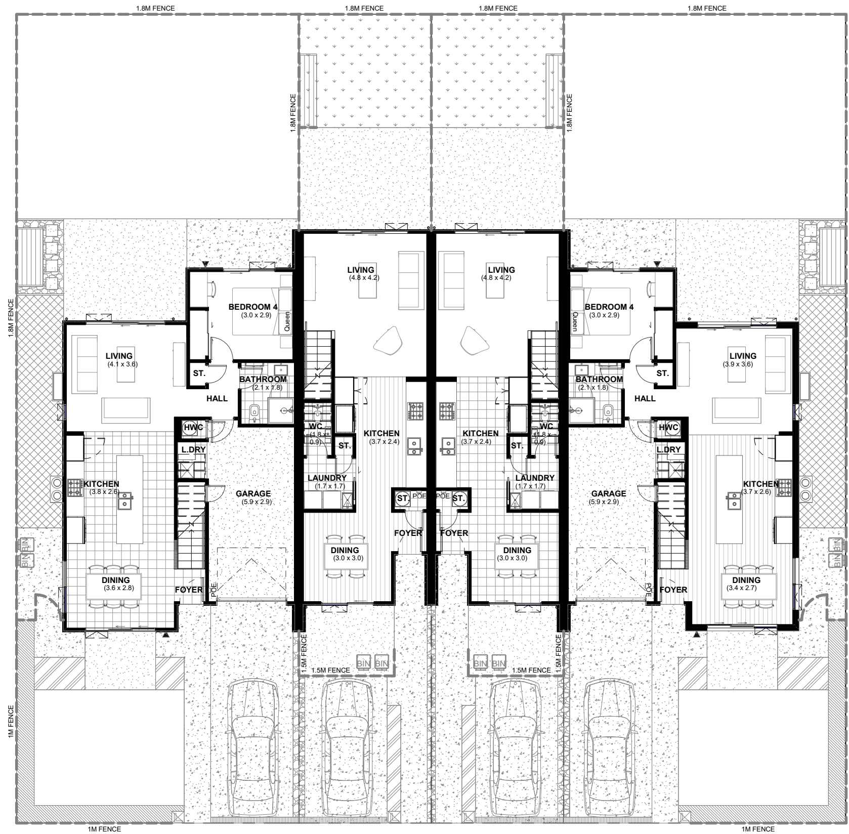
LOT 42 GROUND FLOOR PLAN
