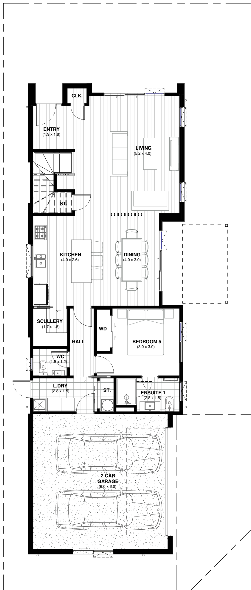
LOT 3053 - GROUND FLOOR PLAN
