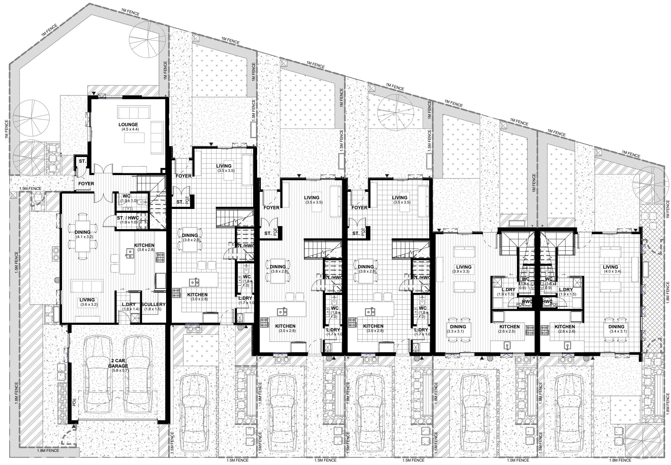
LOT 46 GROUND FLOOR PLAN 35 ADLAM LANE, CONIFER GROVE Floor Area - 200m 2 Site Area - 251m 2 Ground Floor - 117m 2 First Floor - 83m 2 LOT 47 GROUND FLOOR PLAN 37 ADLAM LANE, CONIFER GROVE Floor Area - 112m 2 Site Area - 134m 2 Ground Floor - 56m 2 First Floor - 56m 2 LOT 48 GROUND FLOOR PLAN 39 ADLAM LANE, CONIFER GROVE Floor Area - 112m 2 Site Area - 126m 2 Ground Floor - 56m 2 First Floor - 56m 2 LOT 49 GROUND FLOOR PLAN 41 ADLAM LANE, CONIFER GROVE Floor Area - 112m 2 Site Area - 118m 2 Ground Floor - 56m 2 First Floor - 56m 2 LOT 50 GROUND FLOOR PLAN 43 ADLAM LANE, CONIFER GROVE Floor Area - 94m 2 Site Area - 130m 2 Ground Floor - 47m 2 First Floor - 47m 2 LOT 51 GROUND FLOOR PLAN 45 ADLAM LANE, CONIFER GROVE Floor Area - 94m 2 Site Area - 142m 2 Ground Floor - 47m 2 First Floor - 47m 2
