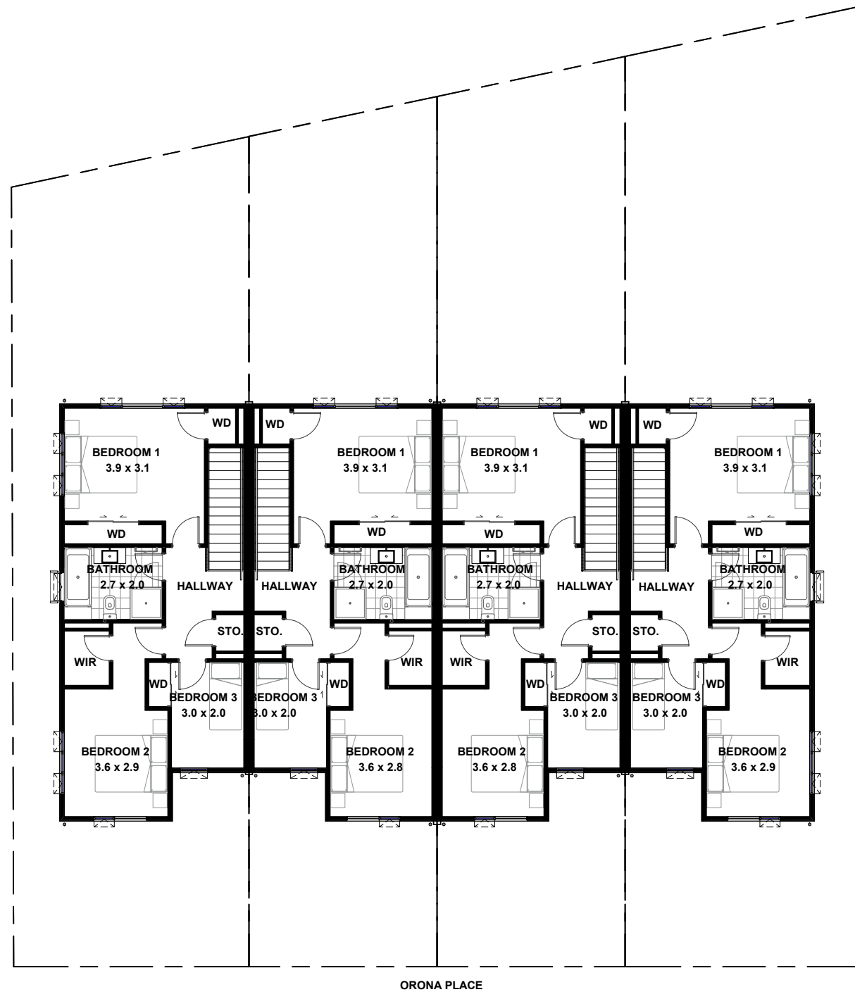
LOT 37 FIRST FLOOR PLAN
