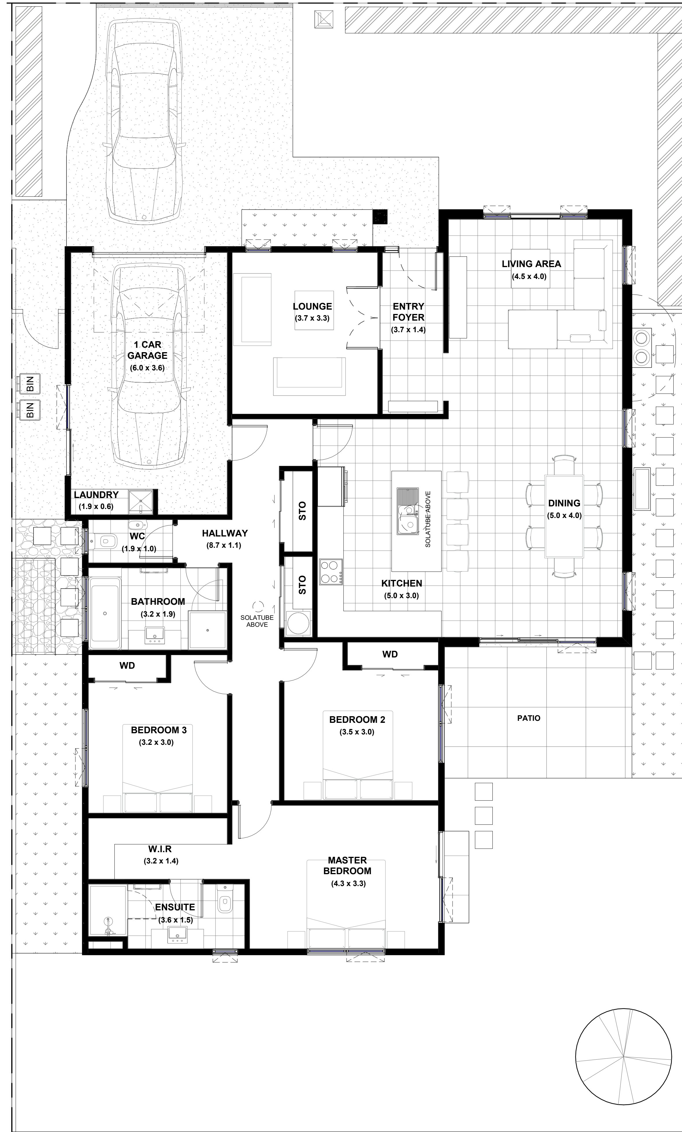
LOT 486 - FLOOR PLAN
