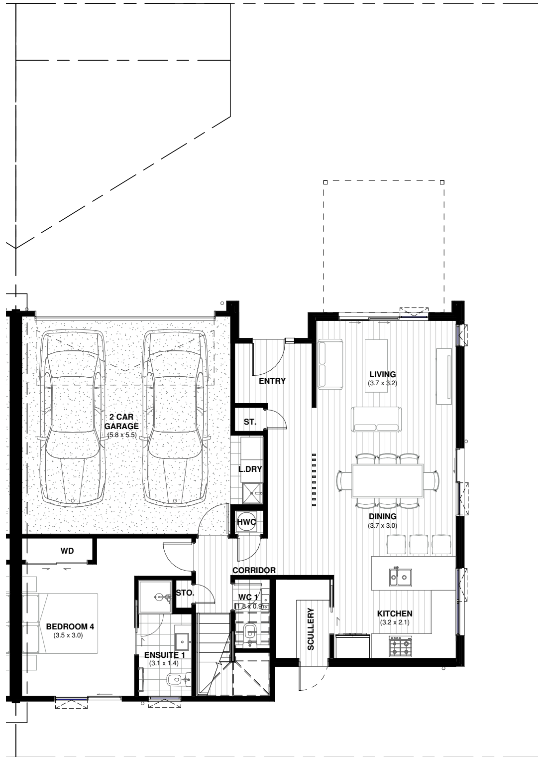
LOT 3083 - GROUND FLOOR PLAN
