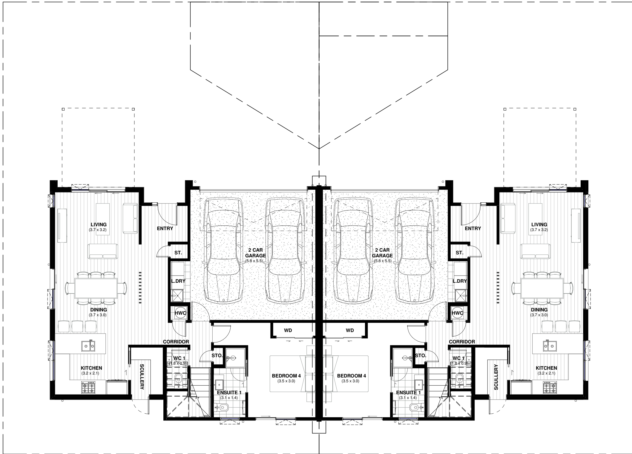
OVERALL GROUND FLOOR PLAN
