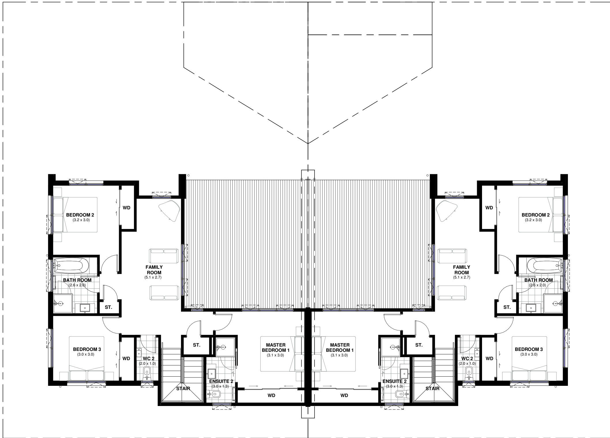
OVERALL FIRST FLOOR PLAN
