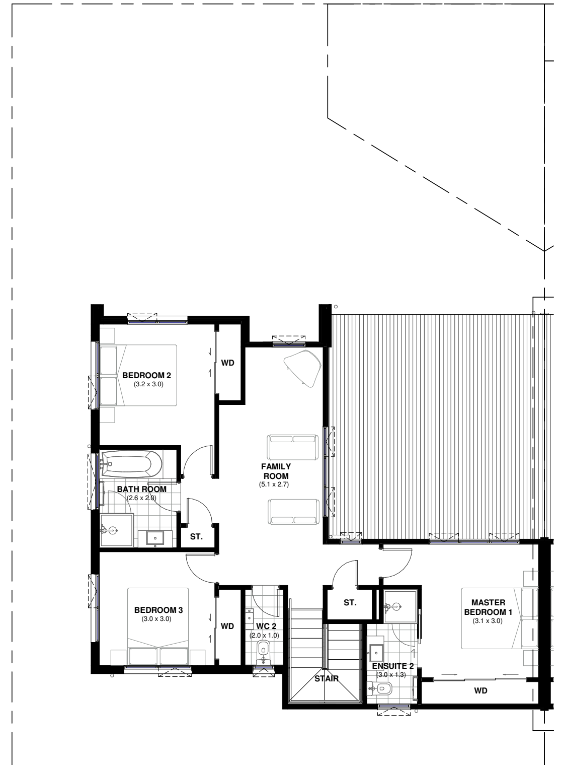
LOT 3082 - FIRST FLOOR PLAN
