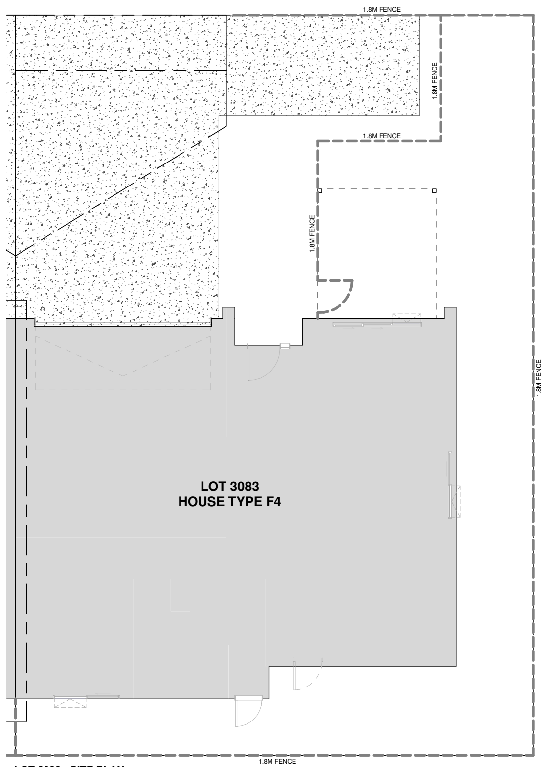
LOT 3083 - SITE PLAN
