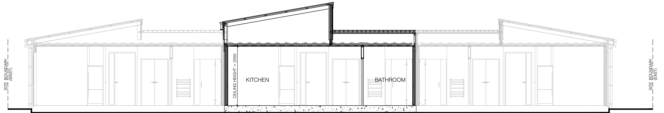
CROSS SECTION
