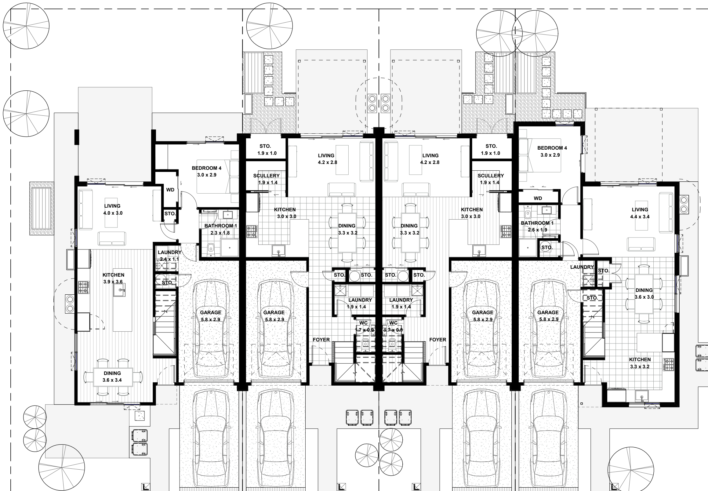
LOT 3061 GROUND FLOOR PLAN
