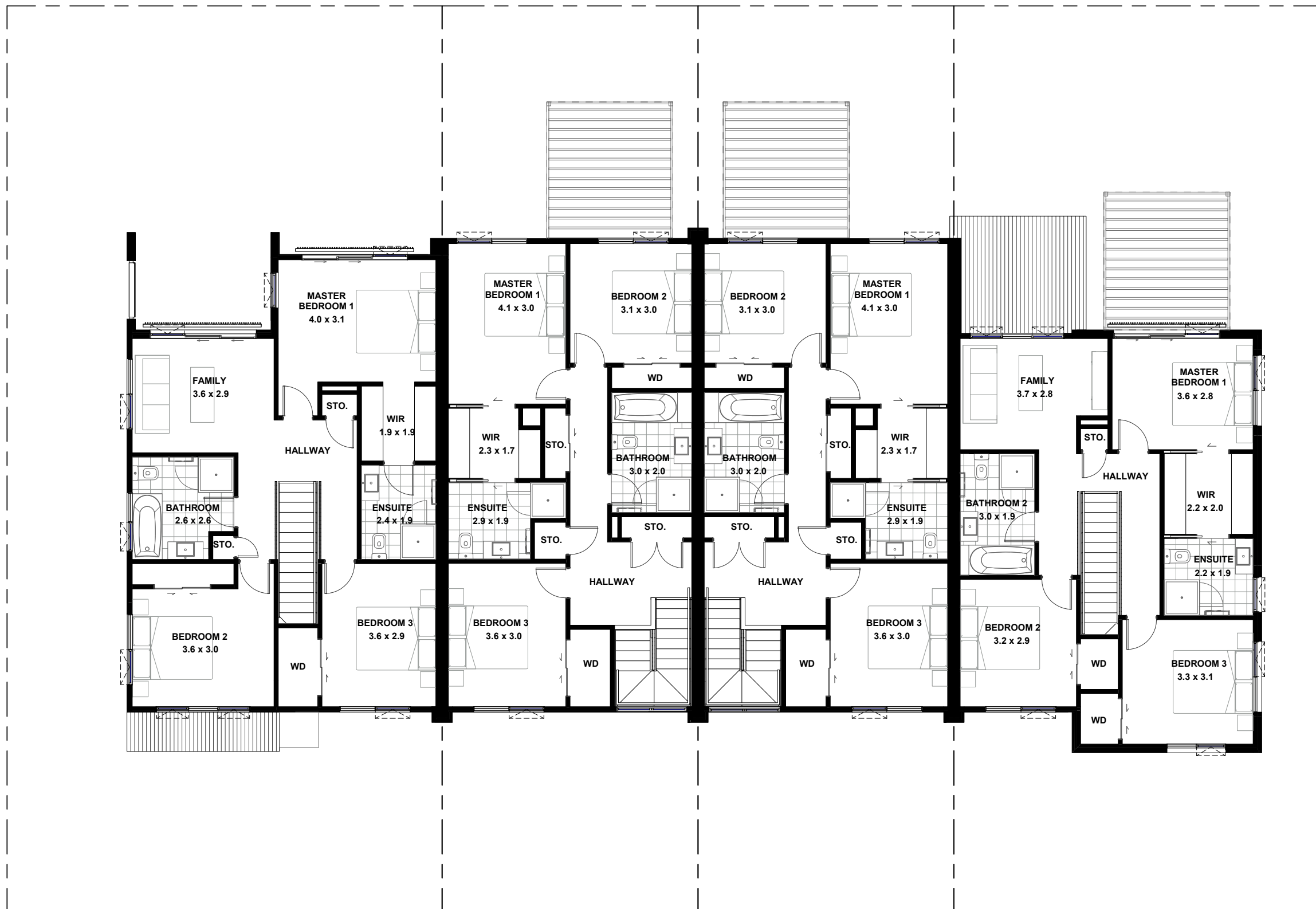
LOT 3061 FIRST FLOOR PLAN
