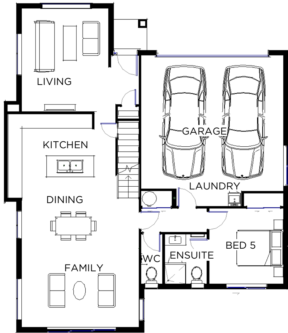
① Lower - Floor Plan - ART 1 : 100
