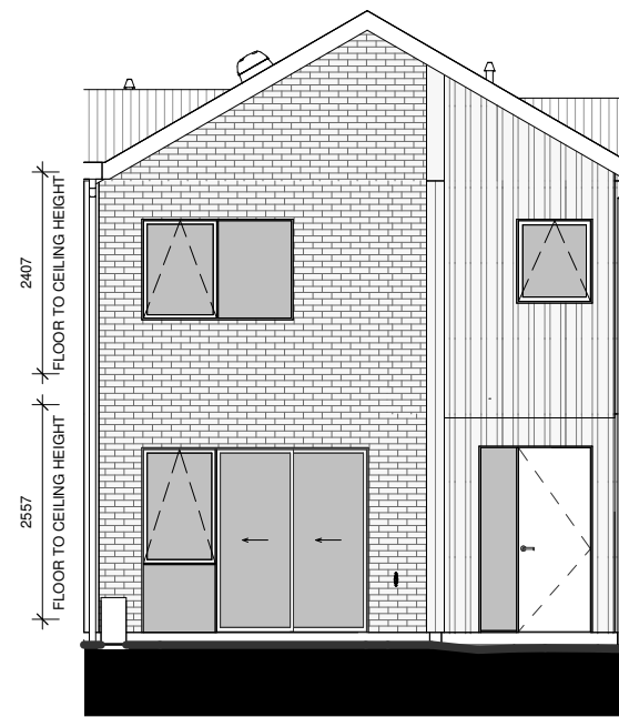
LOT 79 - EAST ELEVATION
