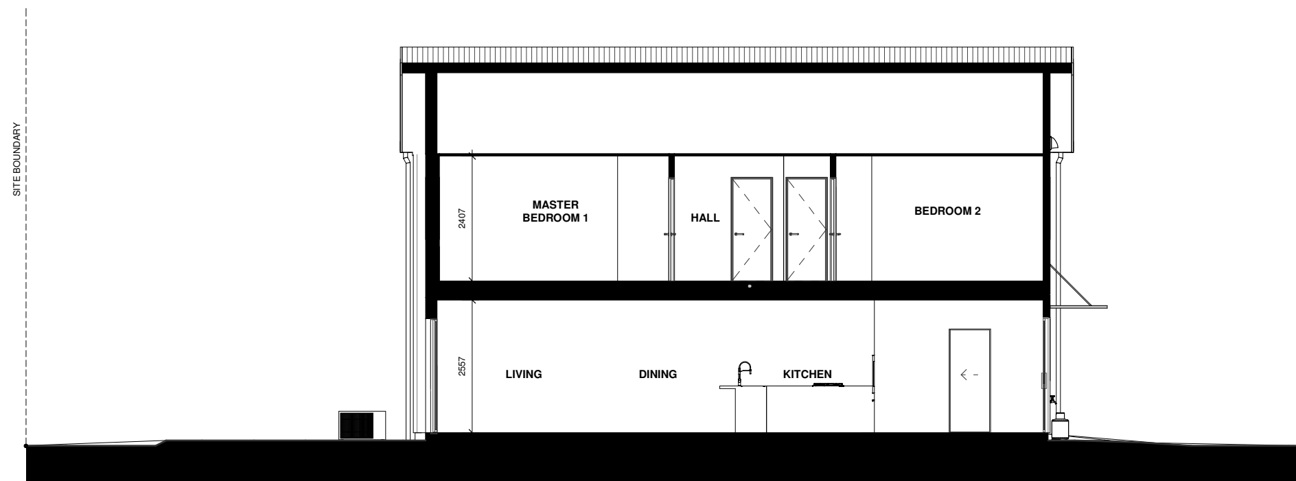
LOT 79 - SECTION A-A
