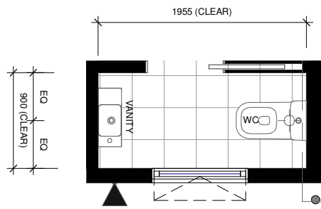
LOT 80 - GROUND FLOOR WC LAYOUT
