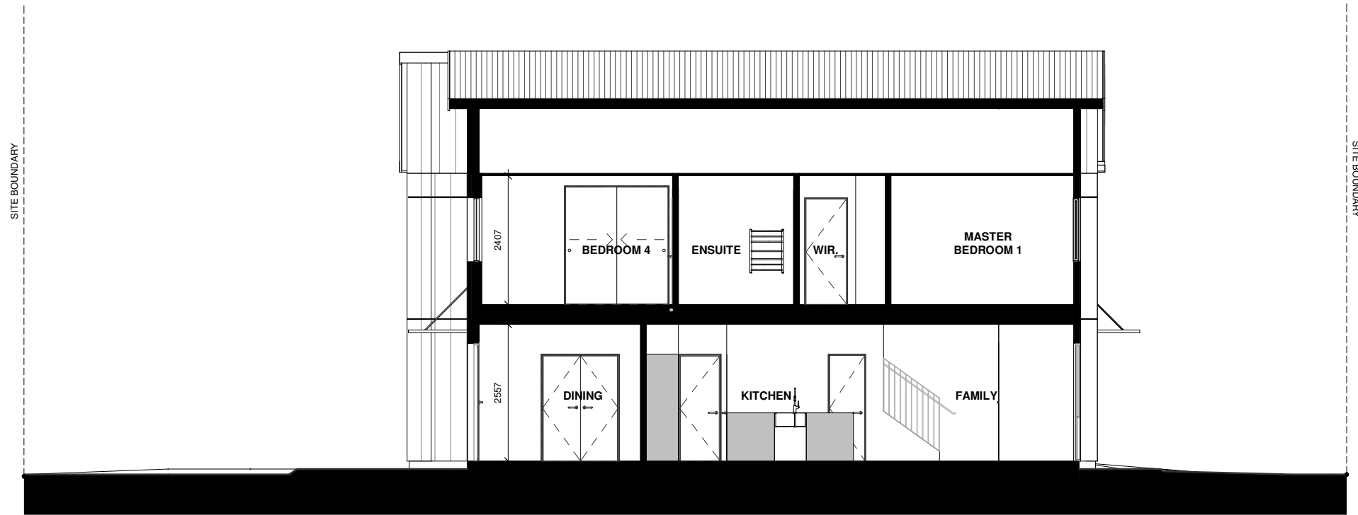
LOT 78 - SECTION A-A
