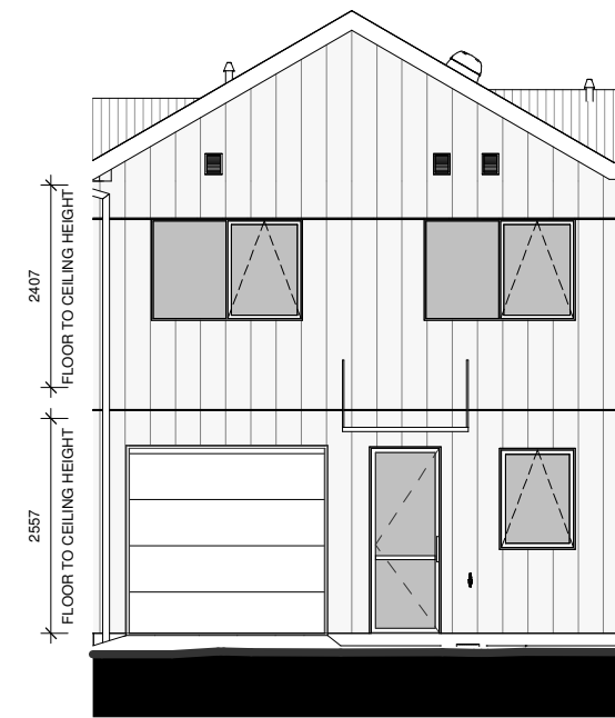
LOT 79 - WEST ELEVATION
