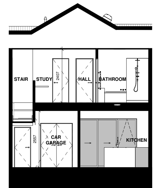
LOT 79 - SECTION B-B
