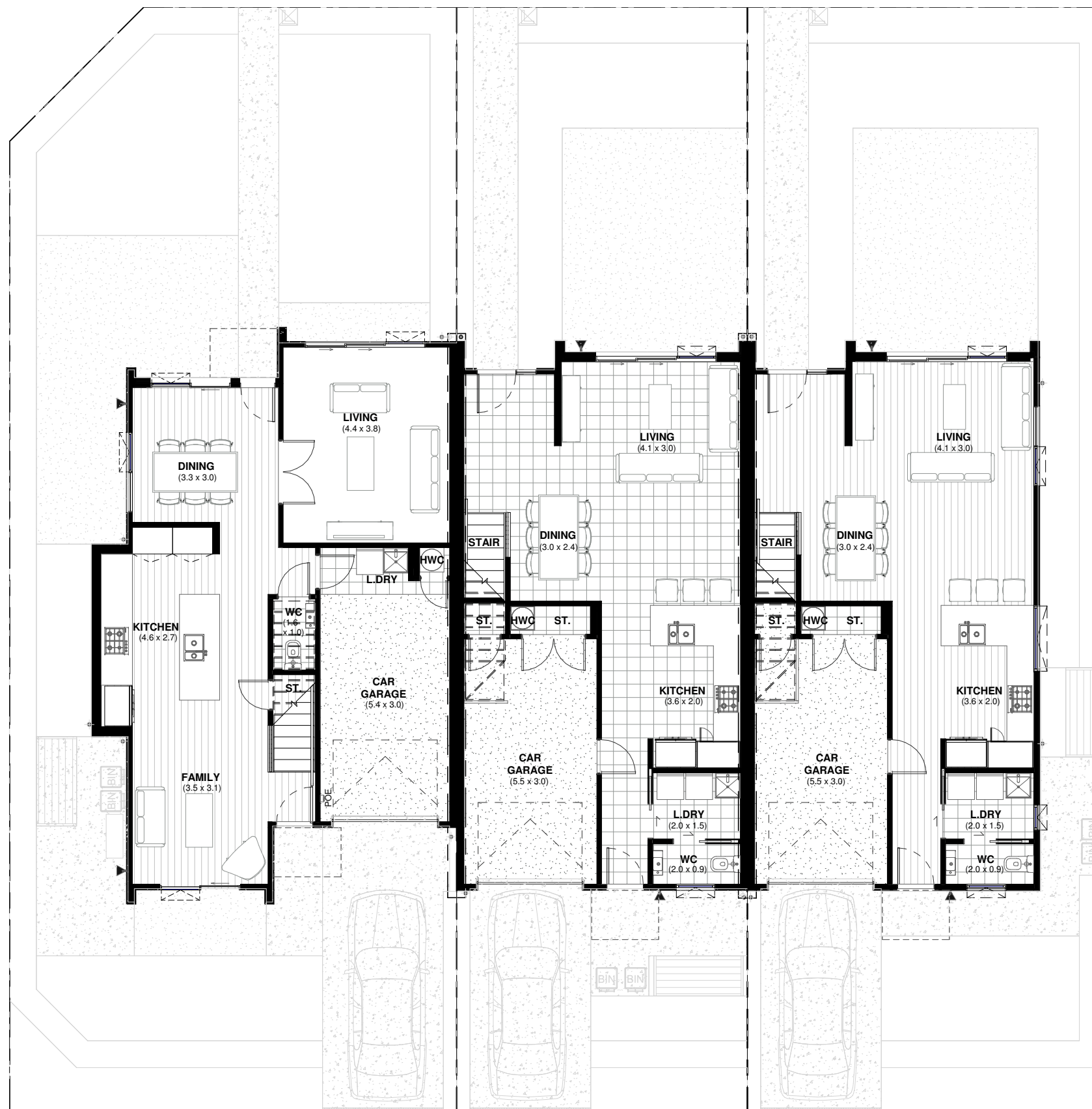
LOT 78 GROUND FLOOR PLAN 2 AQUAMARINE ROAD, HINGAIA Floor Area - 170m 2 Site Area - 243m 2 Ground Floor - 85m 2 First Floor - 85m 2
