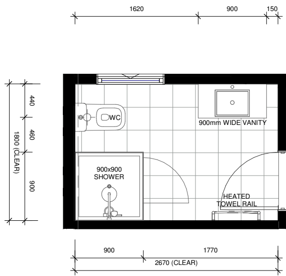
LOT 79 - FIRST FLOOR ENSUITE LAYOUT
