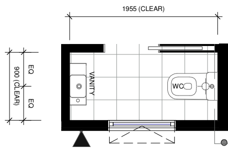
LOT 79 - GROUND FLOOR WC LAYOUT
