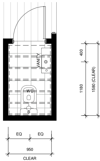
LOT 78 - GROUND FLOOR WC LAYOUT
