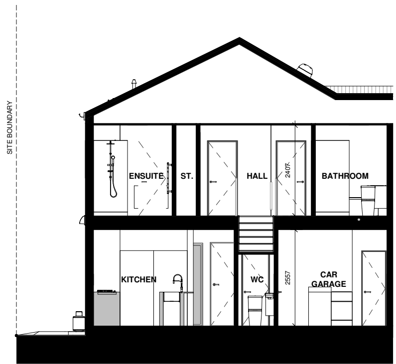
LOT 78 - SECTION B-B
