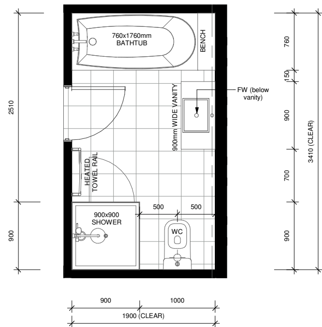
LOT 78 - FIRST FLOOR BATHROOM LAYOUT
