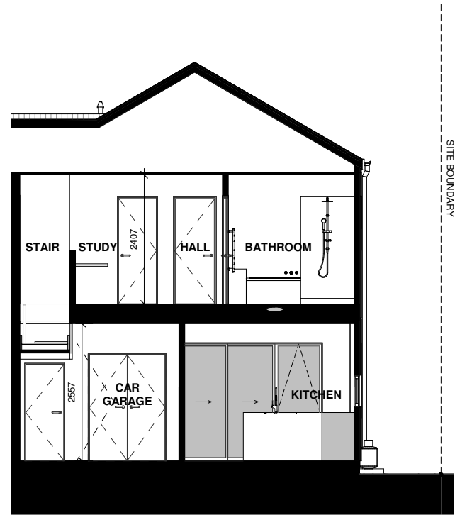
LOT 80 - SECTION B-B
