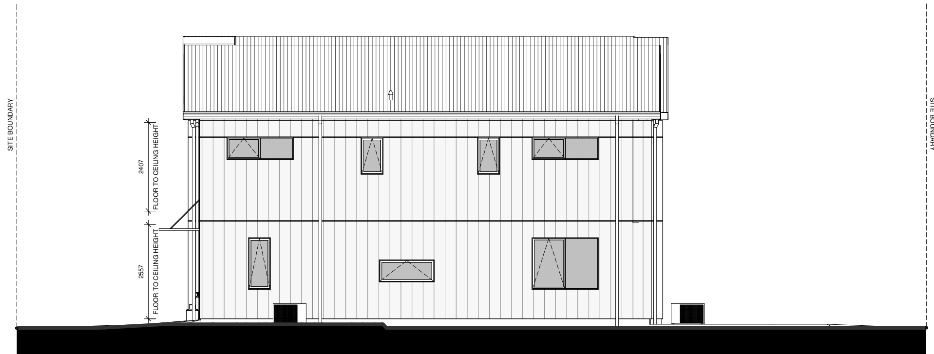
LOT 80 - NORTH ELEVATION
