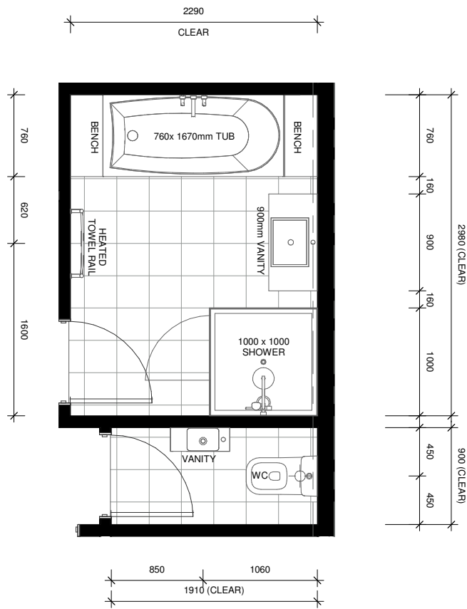
LOT 79 - FIRST FLOOR BATHROOM & WC LAYOUT
