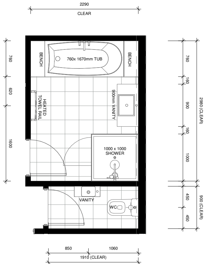
LOT 80 - FIRST FLOOR BATHROOM & WC LAYOUT
