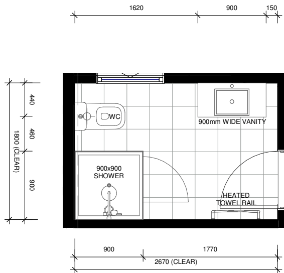
LOT 80 - FIRST FLOOR ENSUITE LAYOUT
