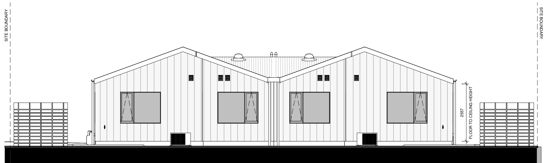
OVERALL WEST ELEVATION
