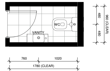
LOT 68 - WC LAYOUT
