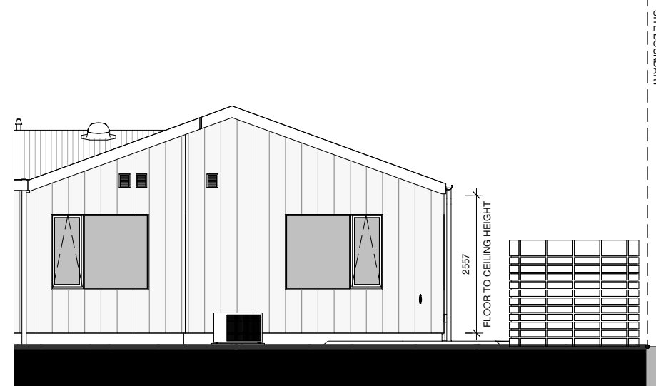
LOT 68 - WEST ELEVATION
