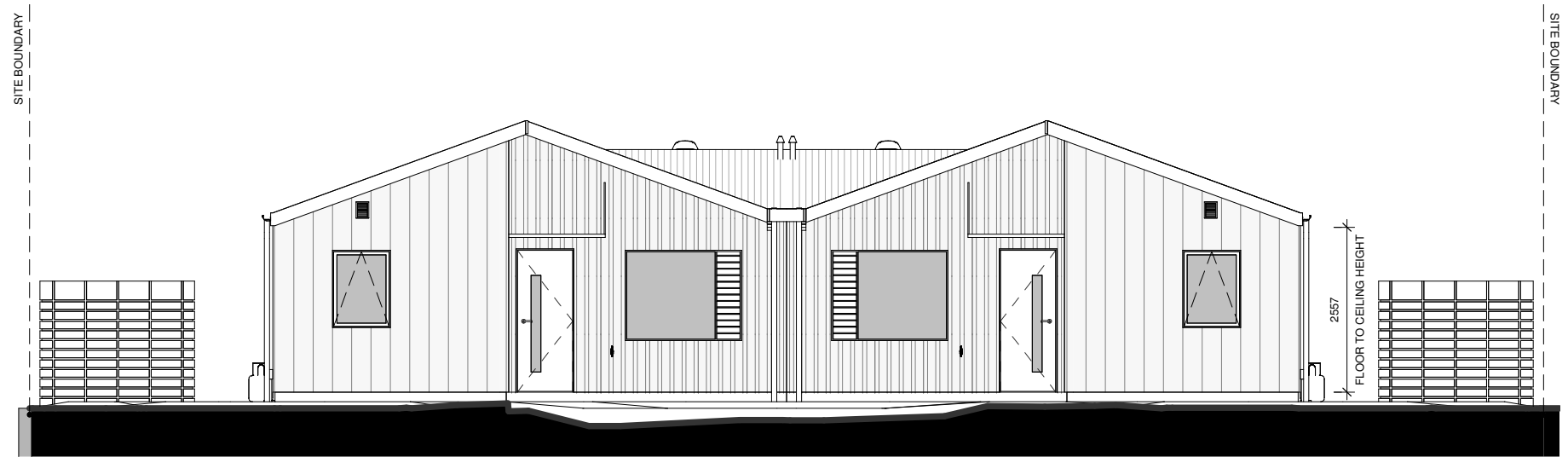
OVERALL EAST ELEVATION
