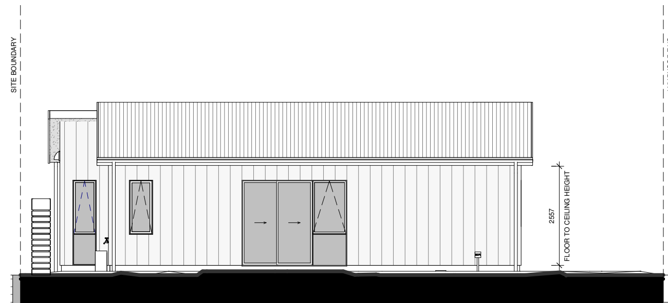
LOT 68 - SOUTH ELEVATION
