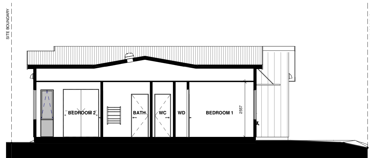
LOT 67 - SECTION C
