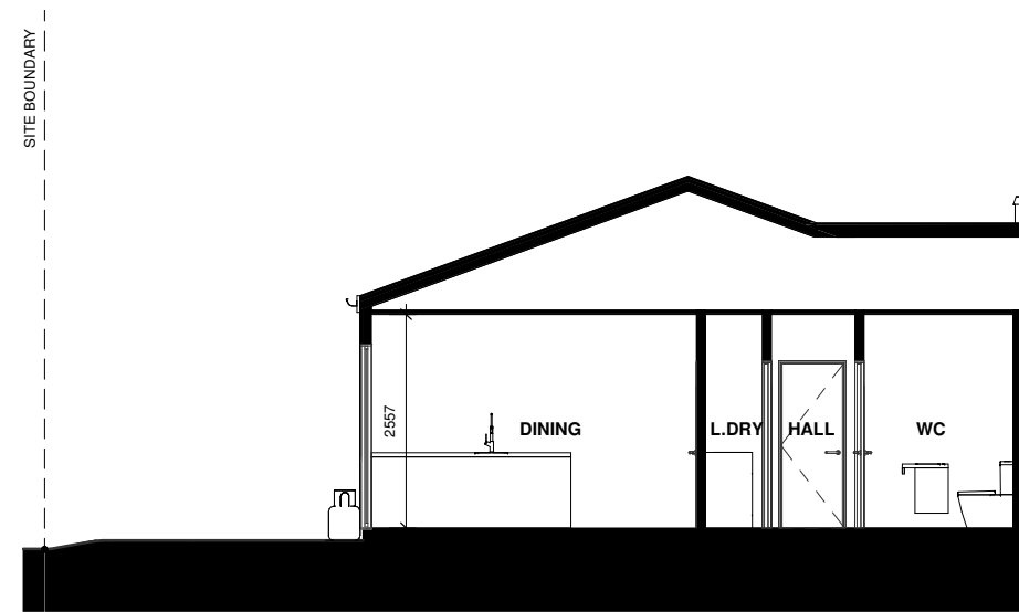
LOT 67 - SECTION B
