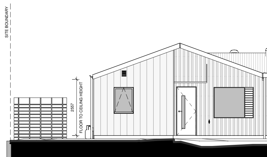
LOT 68 - EAST ELEVATION
