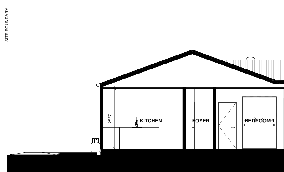
LOT 68 - SECTION A
