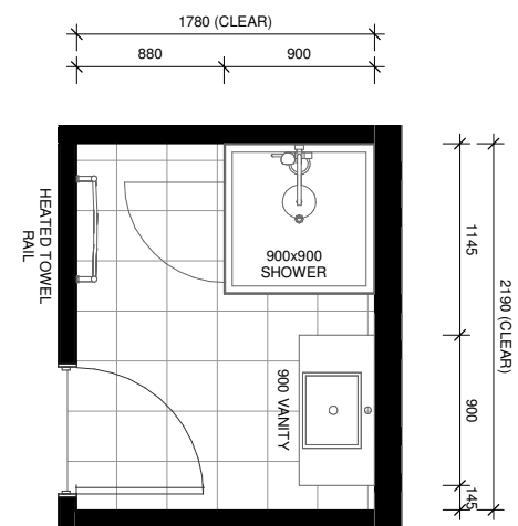
LOT 68 - BATHROOM LAYOUT
