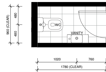
LOT 67 - WC LAYOUT
