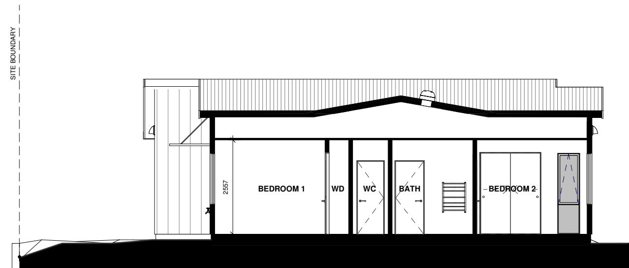
LOT 68 - SECTION C
