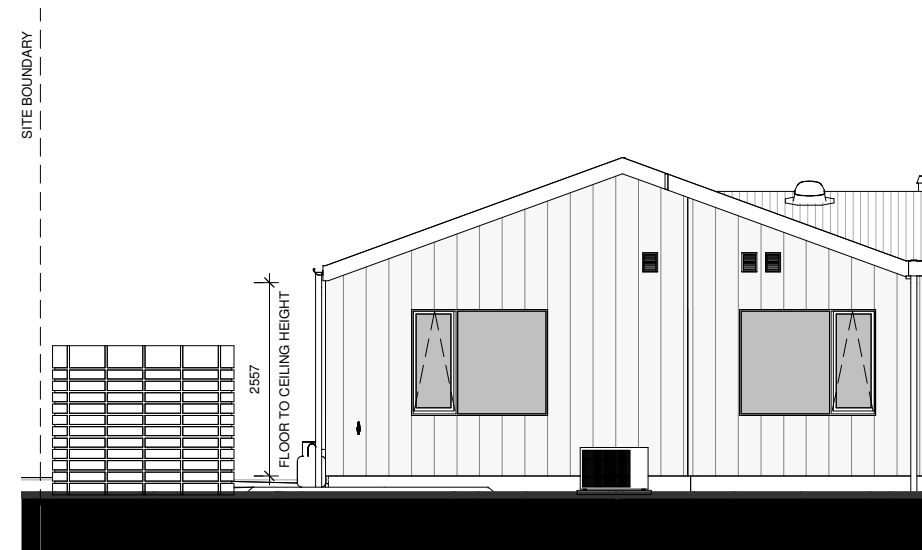
LOT 67 - WEST ELEVATION
