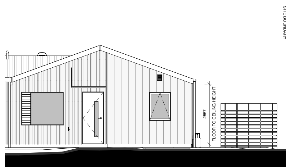
LOT 67 - EAST ELEVATION
