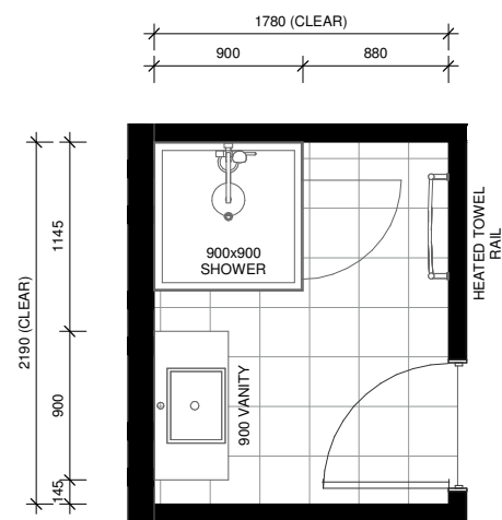
LOT 67 - BATHROOM LAYOUT
