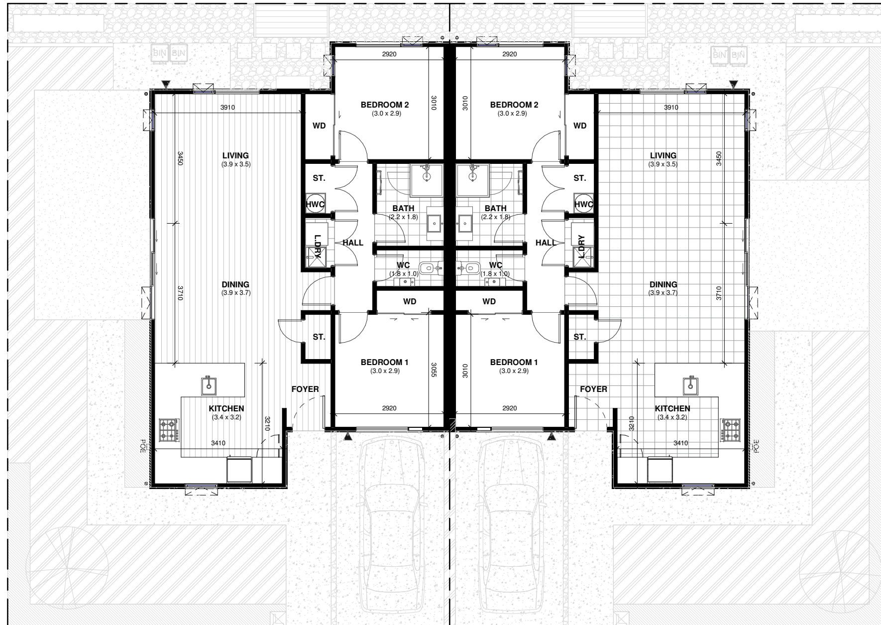
LOT 68 GROUND FLOOR PLAN 3 SEAFOAM ROAD, HINGAIA
