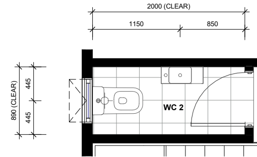
LOT 64 - FIRST FLOOR WC2 LAYOUT
