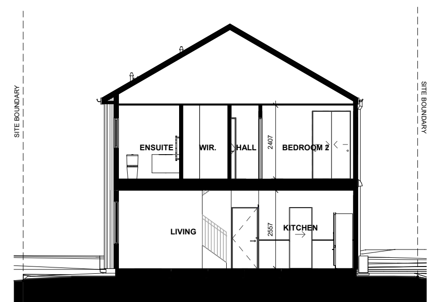
LOT 64 - SECTION C-C
