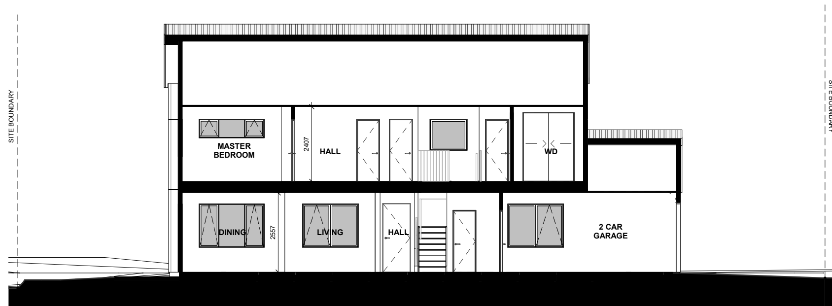
LOT 64 - SECTION A-A
