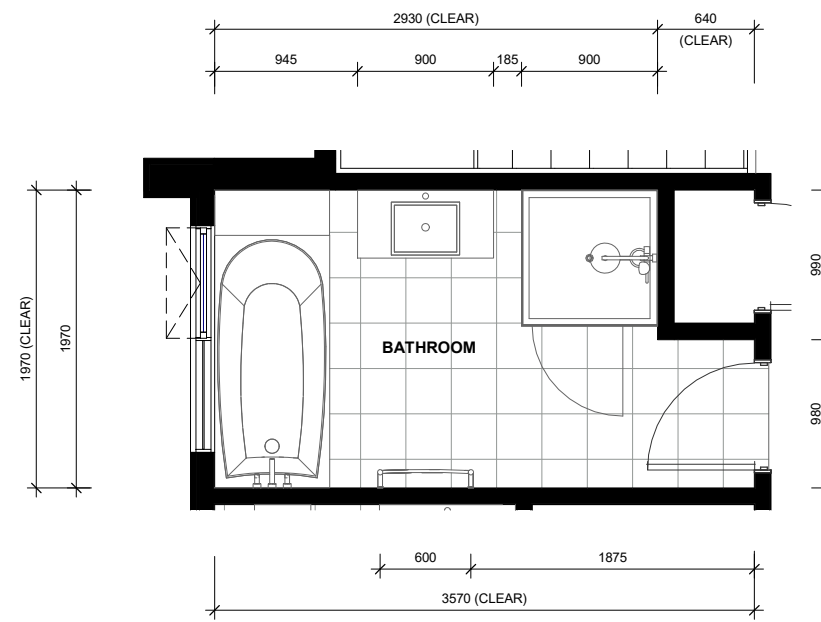
LOT 64 - FIRST FLOOR BATHROOM LAYOUT
