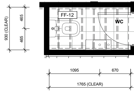
LOT 64 - GROUND FLOOR WC LAYOUT
