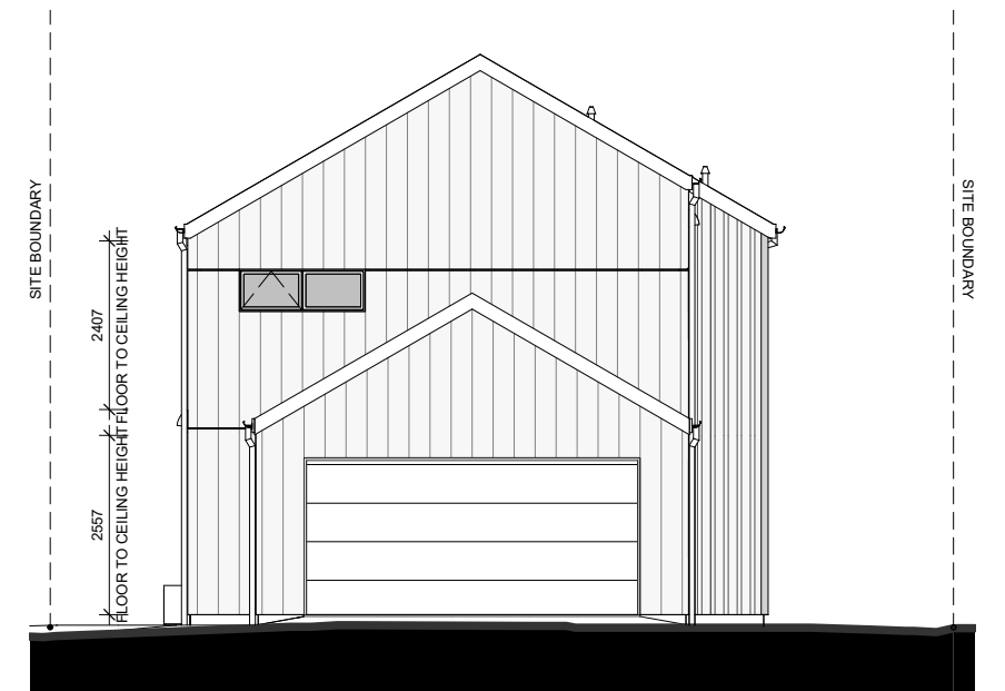
LOT 64 - SOUTH ELEVATION
