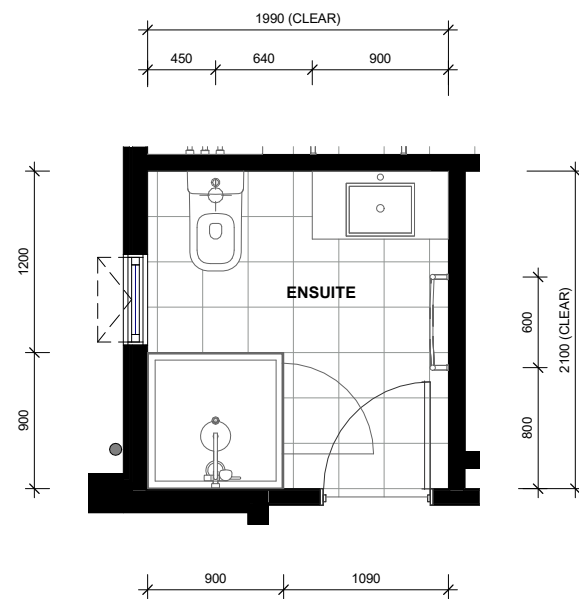
LOT 64 - FIRST FLOOR ENSUITE LAYOUT
