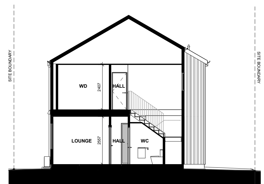
LOT 64 - SECTION D-D
