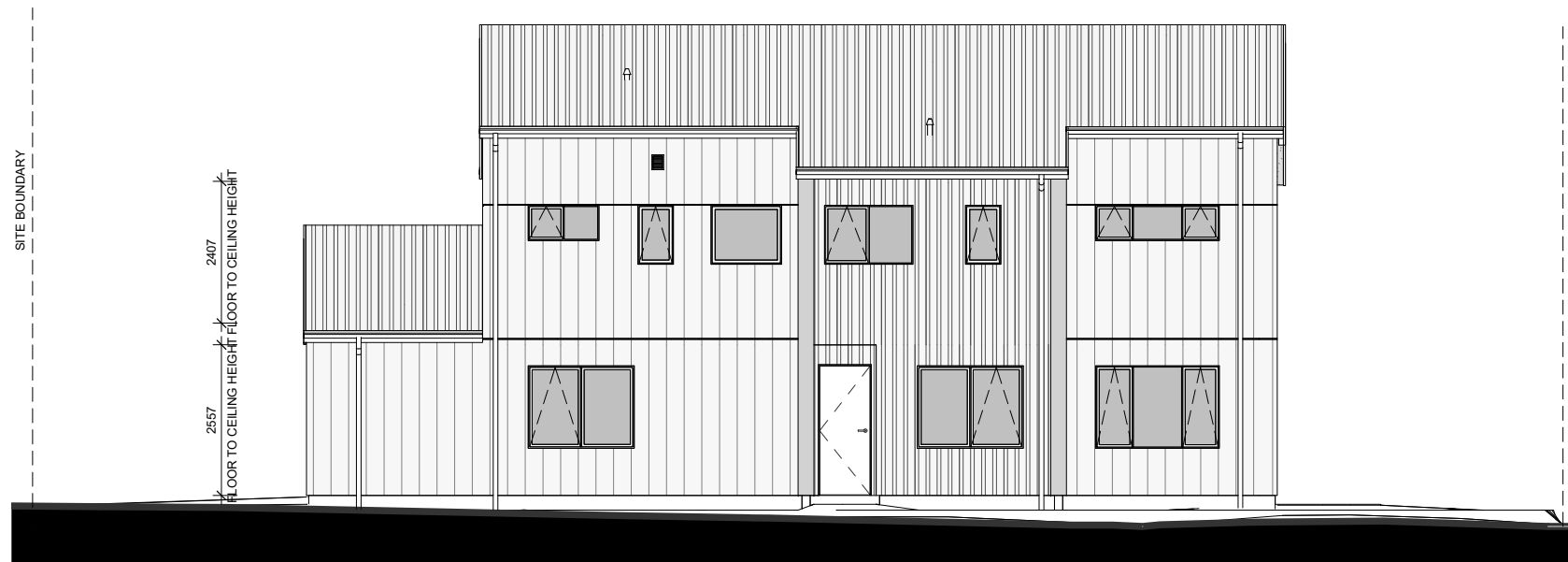
LOT 64 - EAST ELEVATION
