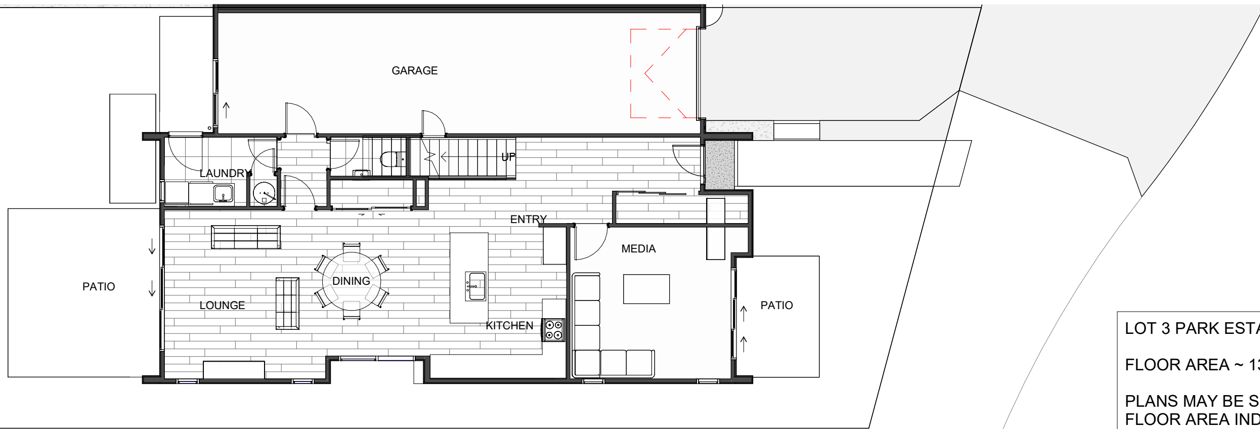
1 A03 - lot 3 Ground Floor Plan - ART A250 1 : 100
