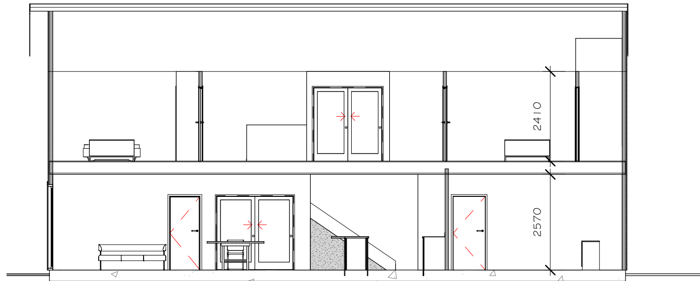
1 Long Section Lot 3 Art A201 1 : 100
