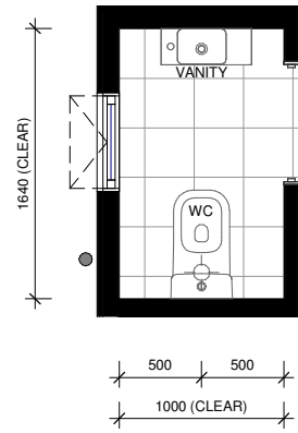
LOT 4 - GROUND FLOOR WC LAYOUT
