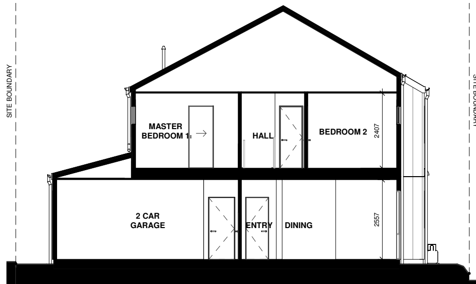
LOT 4 - SECTION F-F
