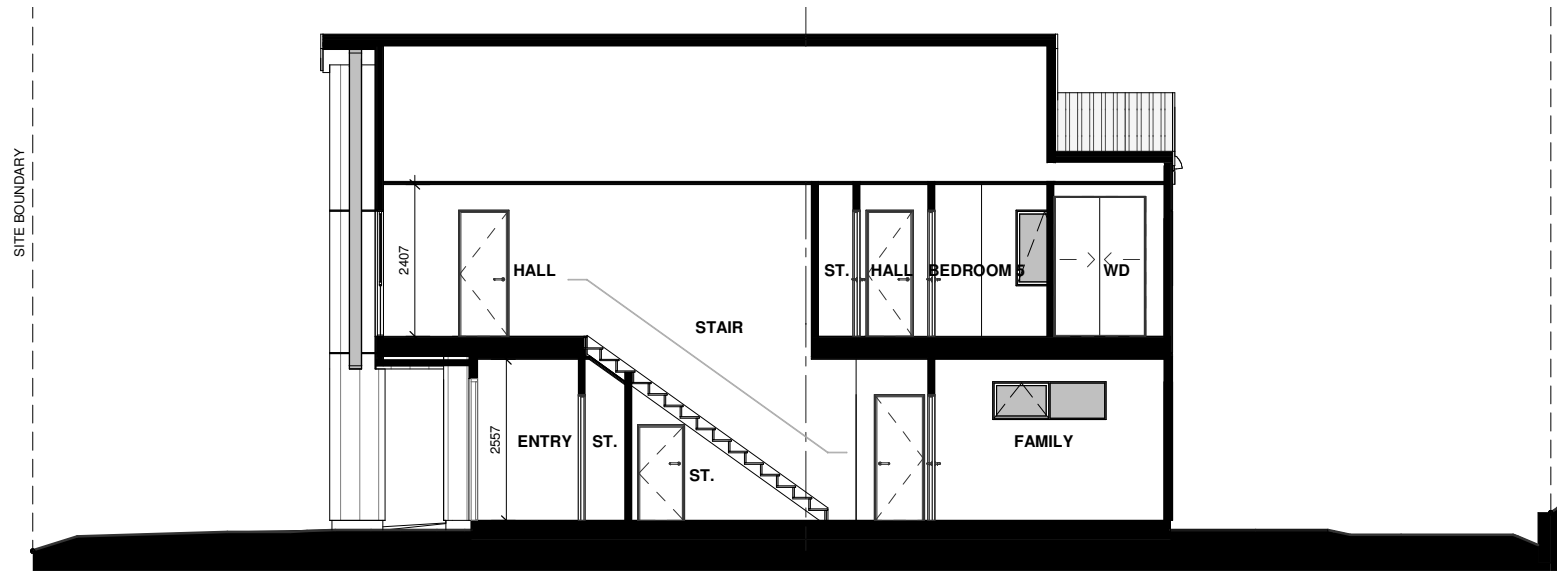
LOT 4 - SECTION A-A
