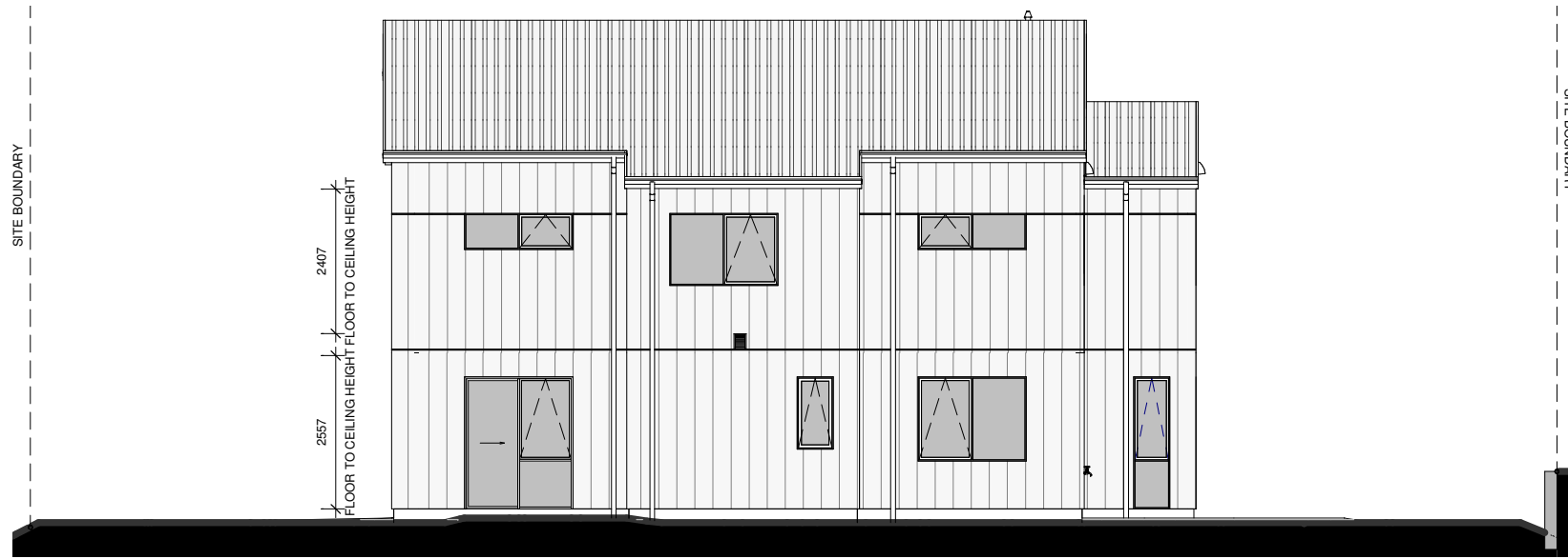
LOT 4 - EAST ELEVATION
