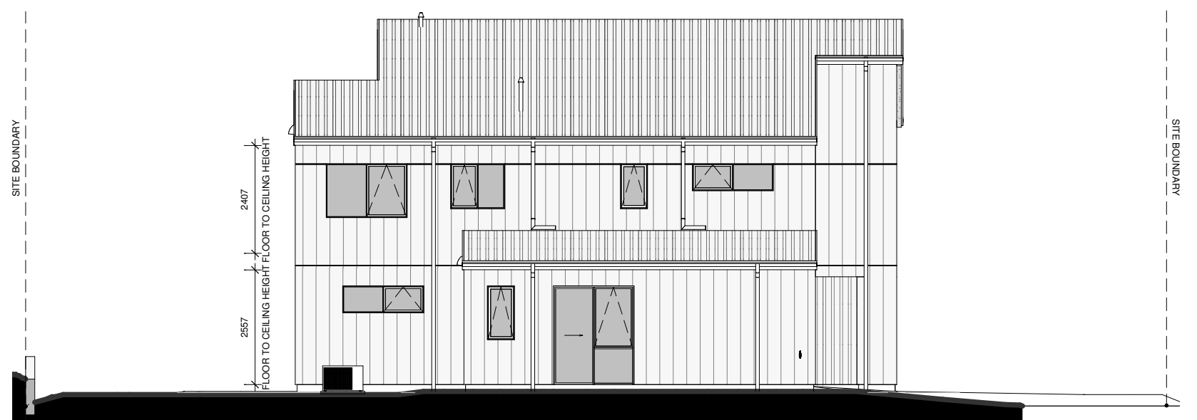
LOT 4 - WEST ELEVATION
