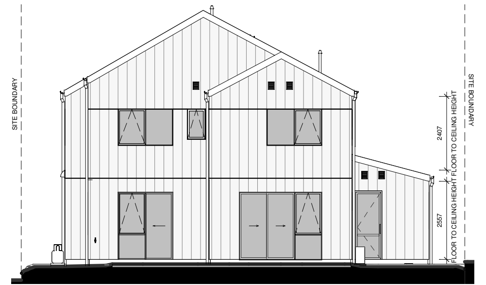
LOT 4 - NORTH ELEVATION
