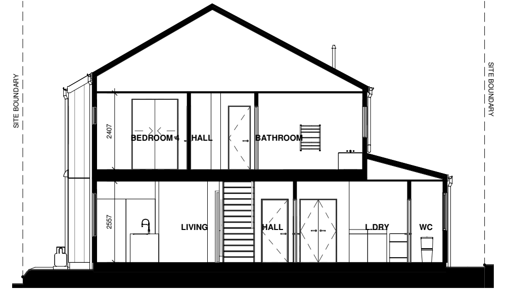
LOT 4 - SECTION E-E
