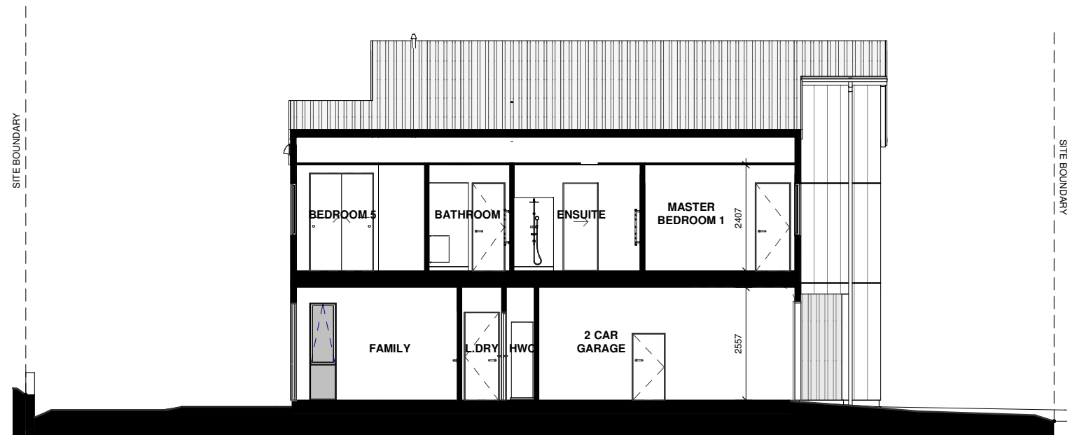
LOT 4 - SECTION C-C
