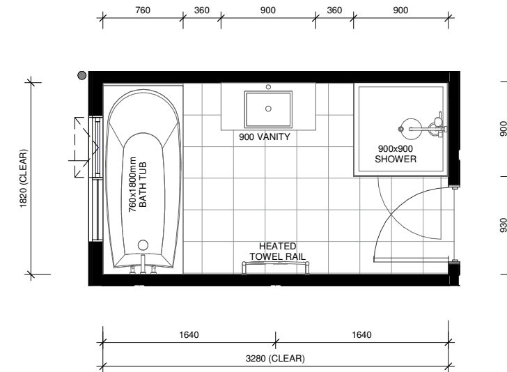
LOT 4 - FIRST FLOOR BATH ROOM LAYOUT
