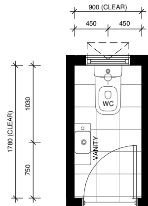
LOT 4 - FIRST FLOOR WC ROOM LAYOUT
