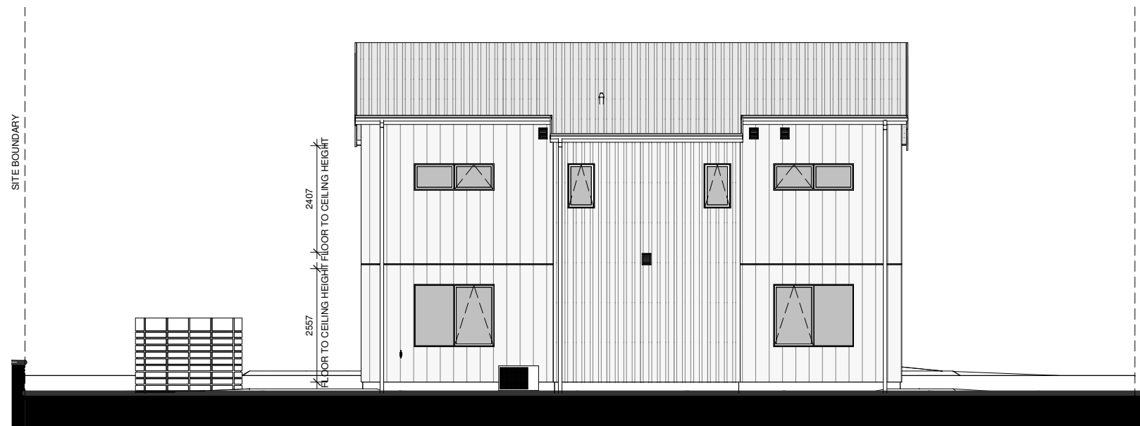
LOT 11 - WEST ELEVATION
