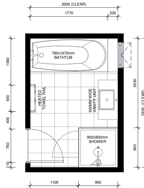
LOT 11 - FIRST FLOOR BATHROOM 1 LAYOUT
