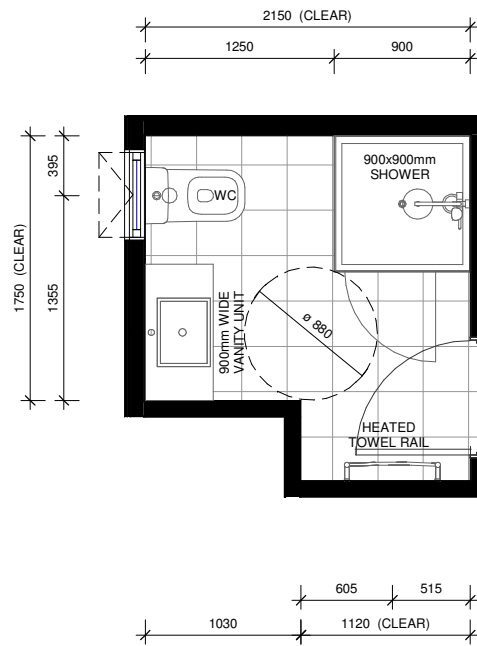
LOT 11 - FIRST FLOOR ENSUITE LAYOUT
