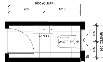
LOT 11 - FIRST FLOOR WC LAYOUT
