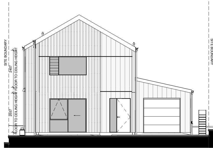
LOT 11 - SOUTH ELEVATION
