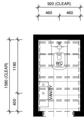
LOT 11 - GROUND FLOOR WC LAYOUT
