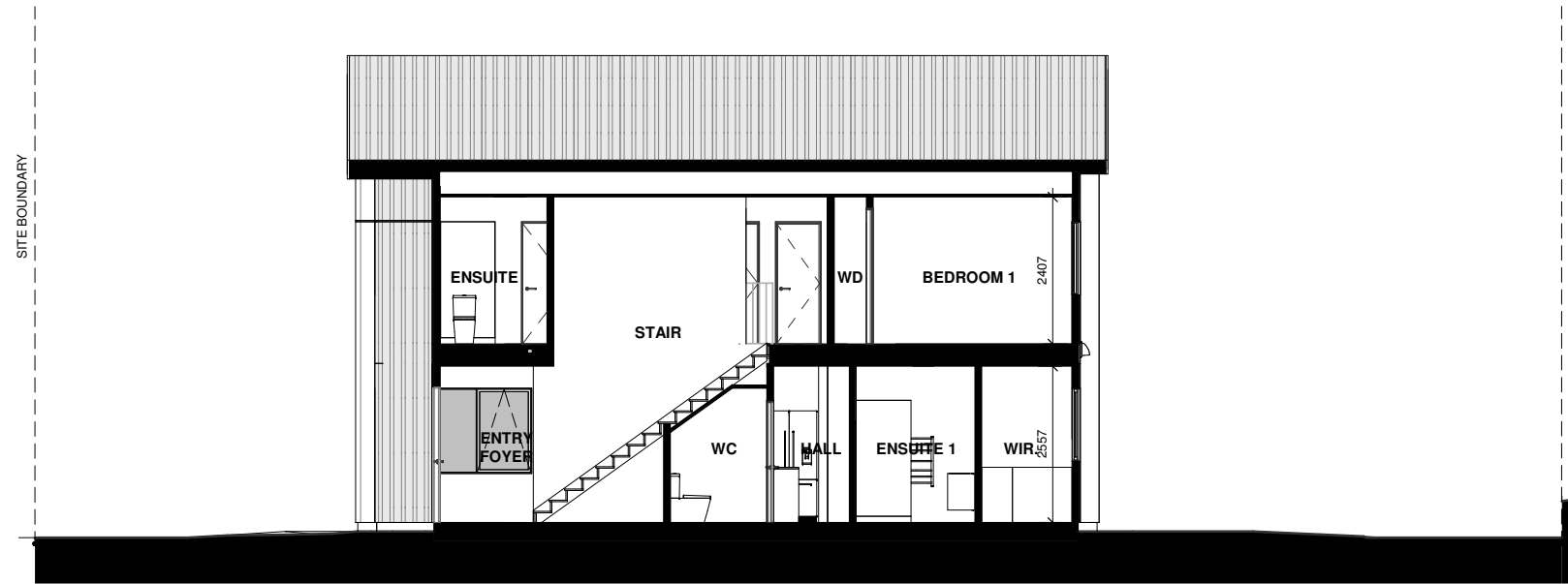
LOT 11 - SECTION A-A
