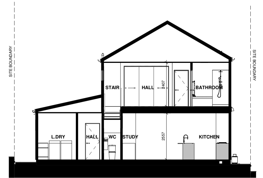
LOT 11 - SECTION C-C
