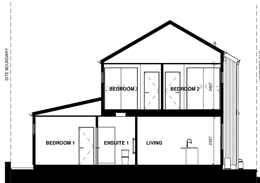
LOT 11 - SECTION D-D
