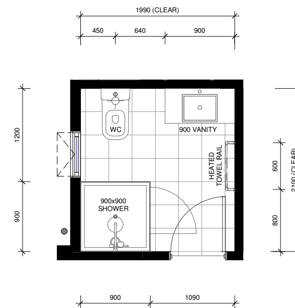
LOT 69 - FIRST FLOOR ENSUITE LAYOUT
