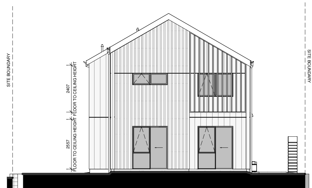
LOT 69 - WEST ELEVATION
