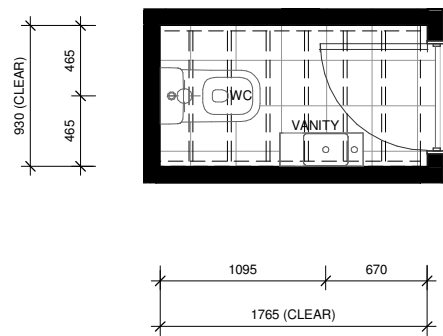
LOT 69 - GROUND FLOOR WC LAYOUT
