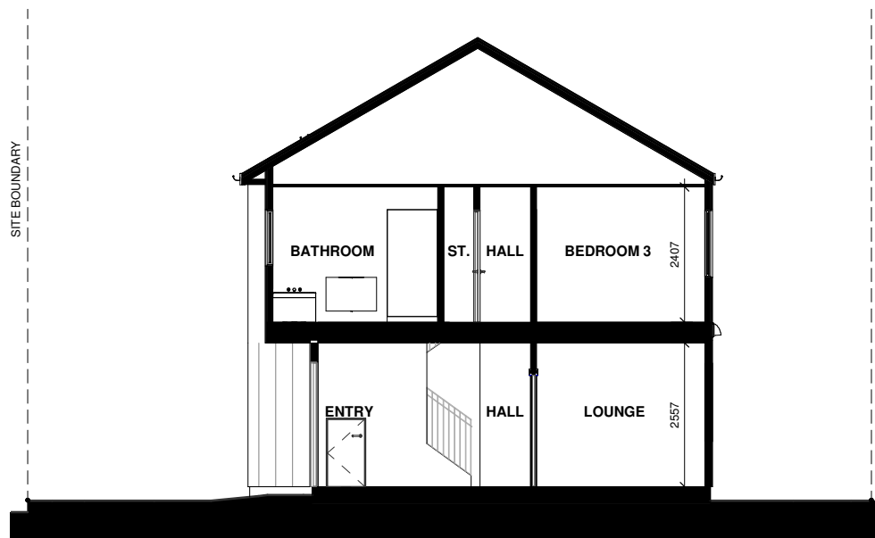
LOT 69 - SECTION D
