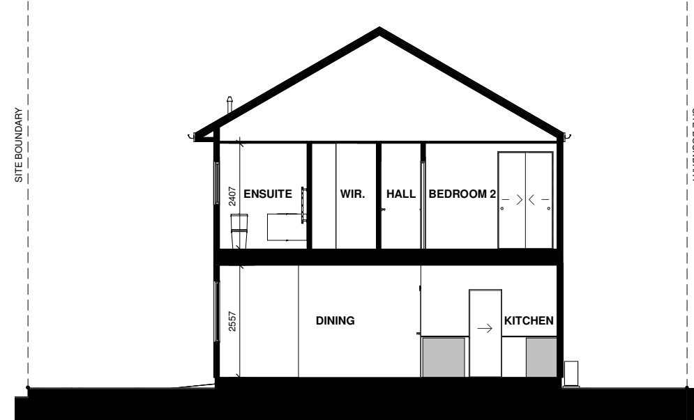
LOT 69 - SECTION C
