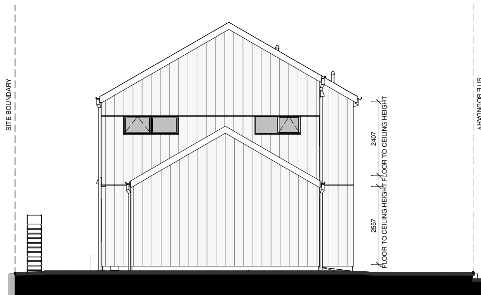
LOT 69 - EAST ELEVATION
