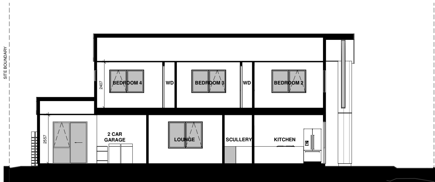
LOT 69 - SECTION A
