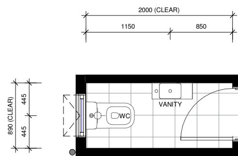
LOT 69 - FIRST FLOOR WC2 LAYOUT
