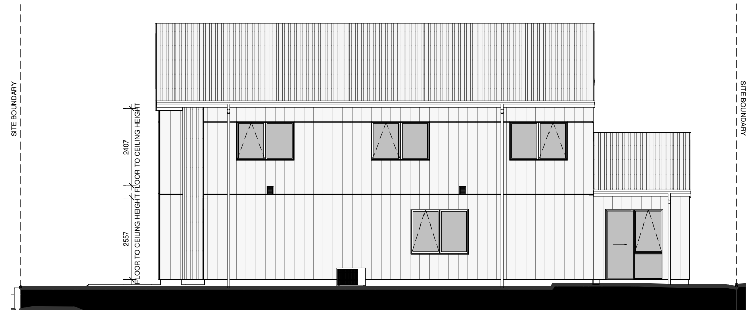
LOT 69 - SOUTH ELEVATION
