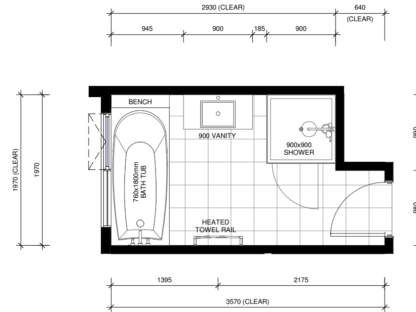
LOT 69 - FIRST FLOOR BATHROOM LAYOUT
