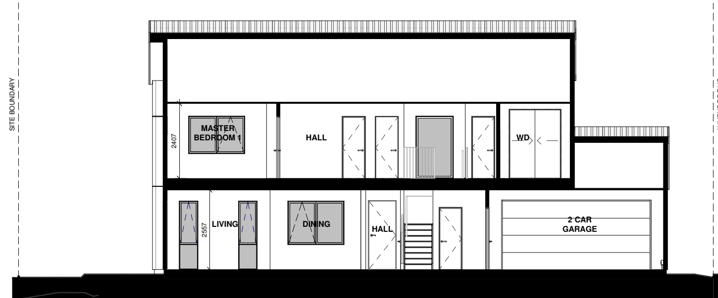
LOT 69 - SECTION B
