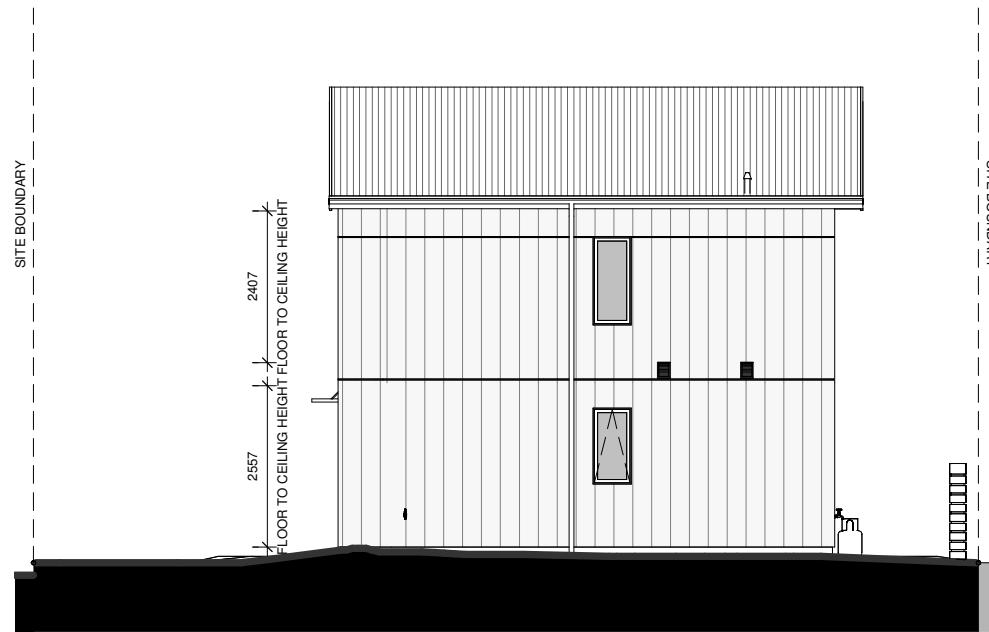
LOT 70 - WEST ELEVATION
