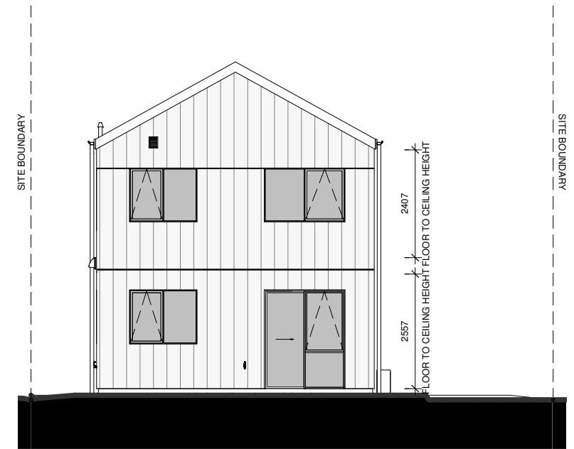
LOT 70 - SOUTH ELEVATION
