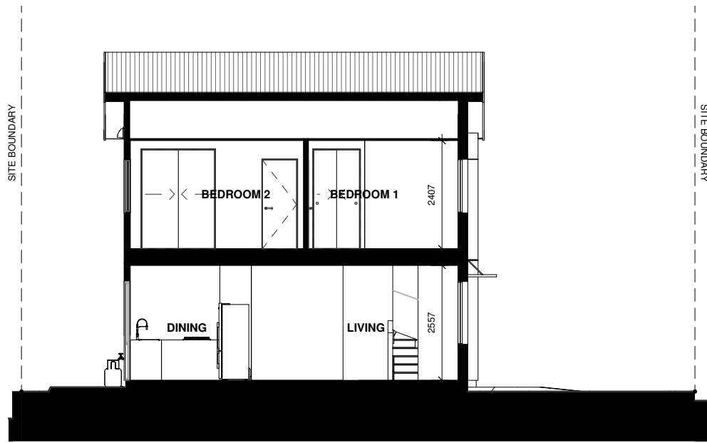
LOT 70 - SECTION A
