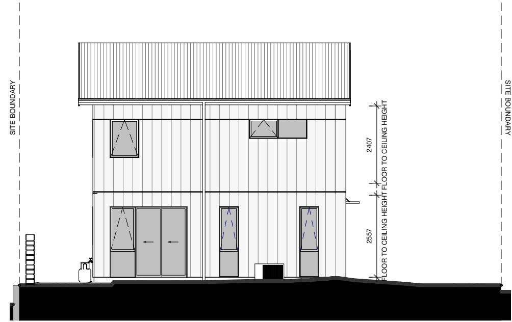
LOT 70 - EAST ELEVATION
