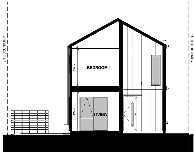
LOT 70 - SECTION D
