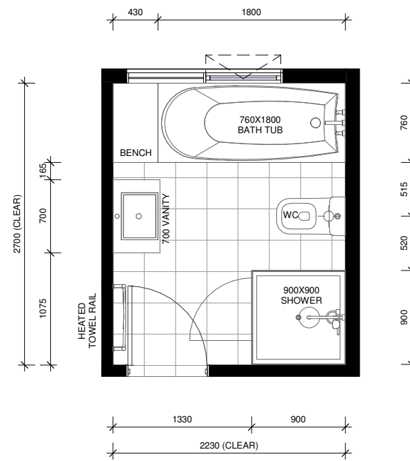
LOT 70 - FIRST FLOOR BATHROOM LAYOUT
