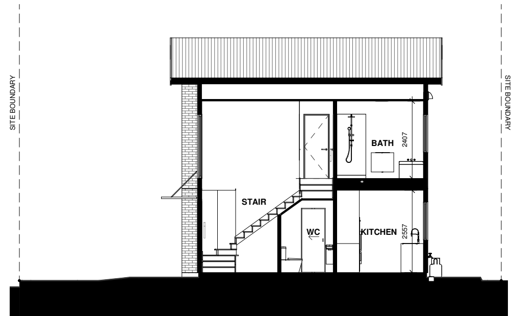
LOT 70 - SECTION B
