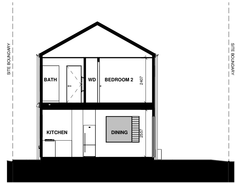
LOT 70 - SECTION C
