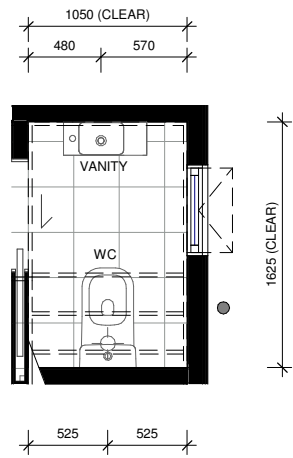
LOT 70 - GROUND FLOOR WC LAYOUT
