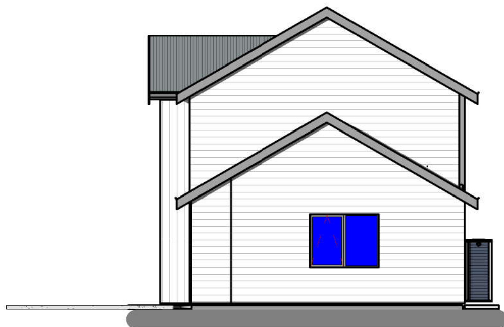
4 01-South A201 1 : 100
