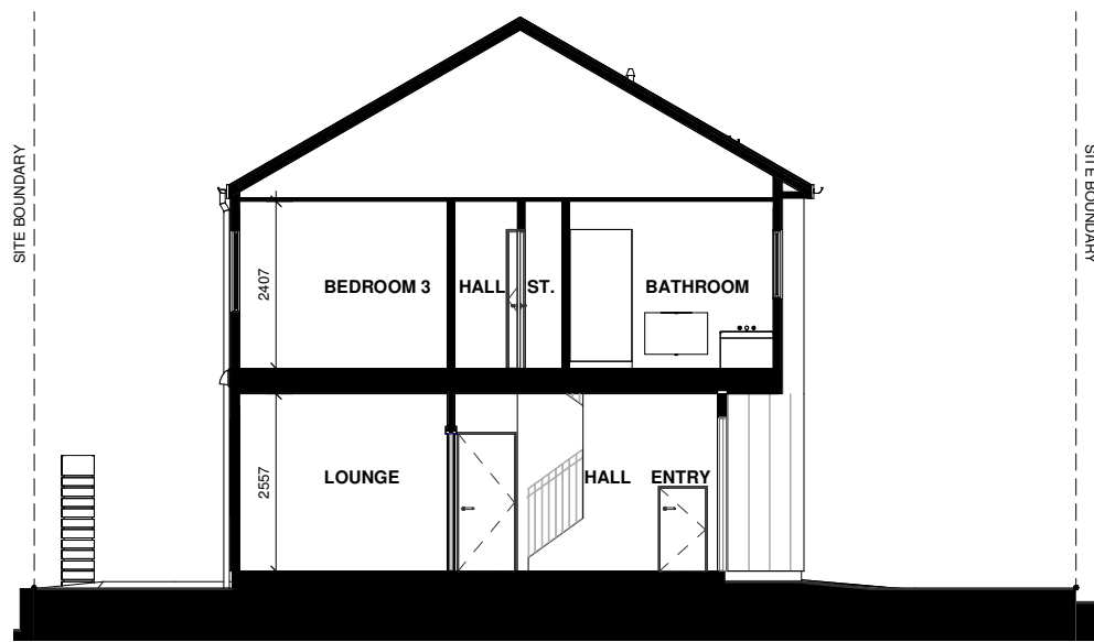
LOT 71 - SECTION D
