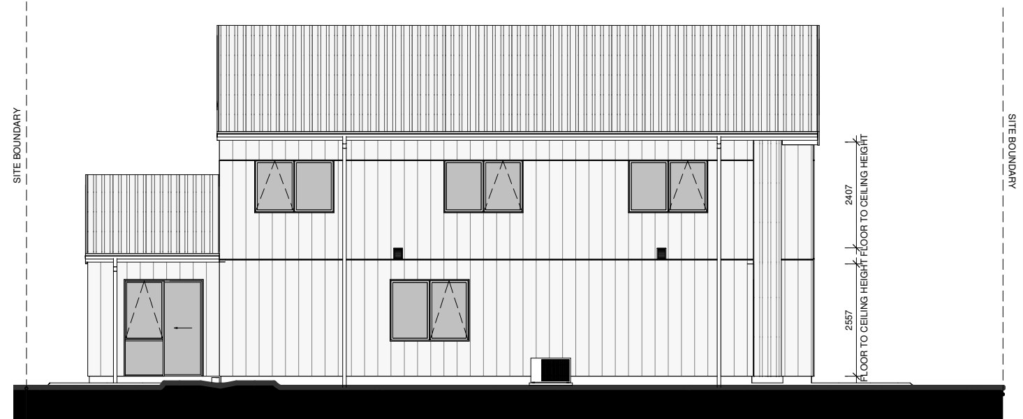
LOT 71 - SOUTH ELEVATION
