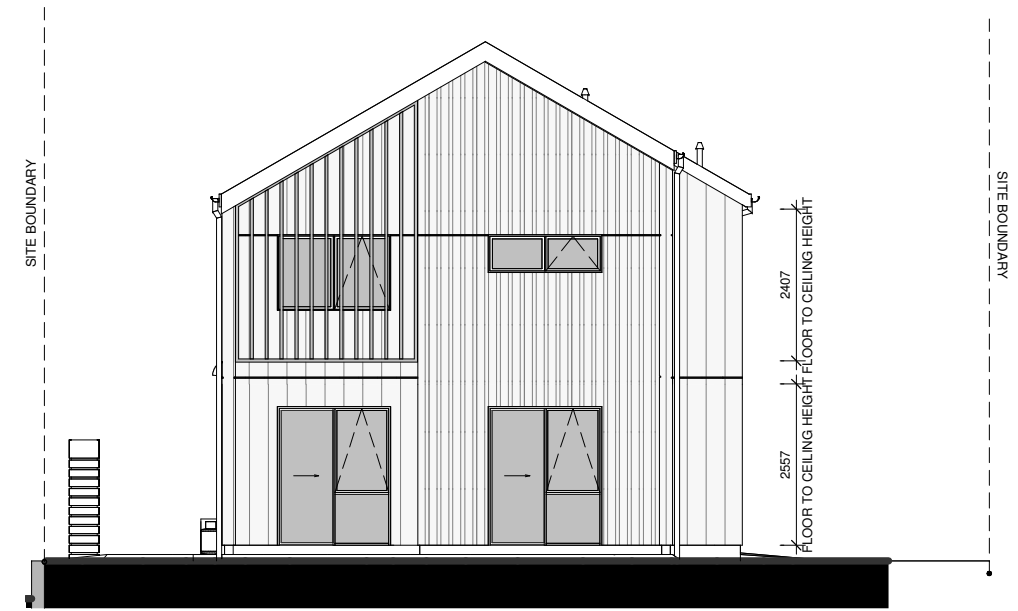
LOT 71 - EAST ELEVATION
