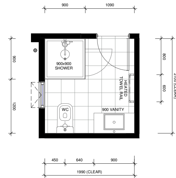
LOT 71 - FIRST FLOOR ENSUITE LAYOUT
