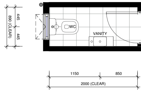
LOT 71 - FIRST FLOOR WC2 LAYOUT
