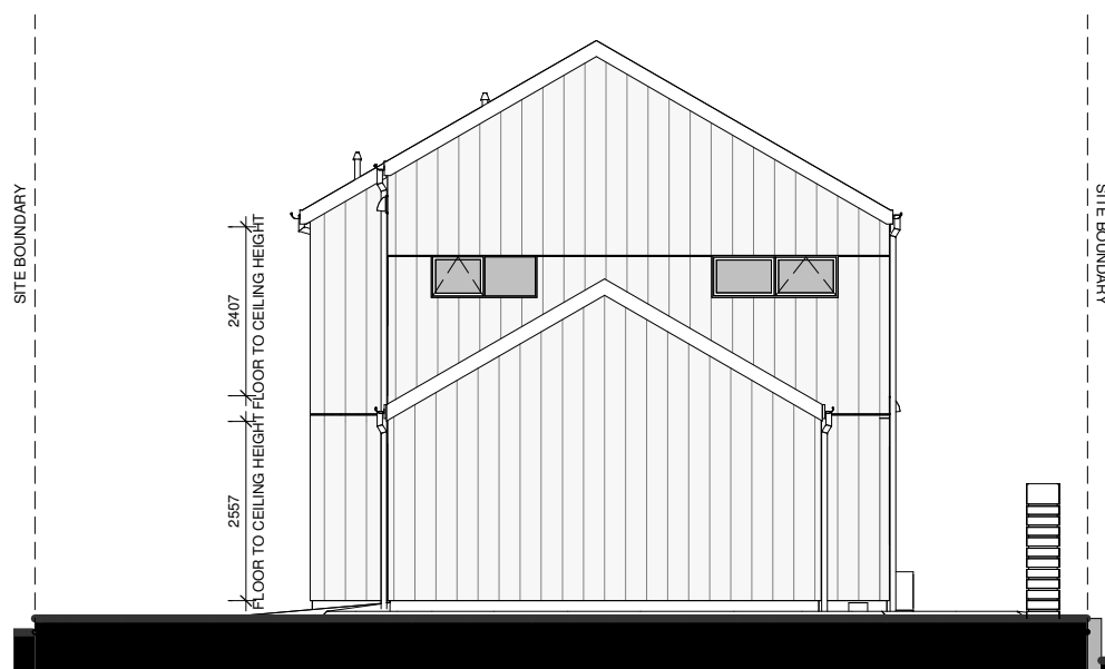
LOT 71 - WEST ELEVATION
