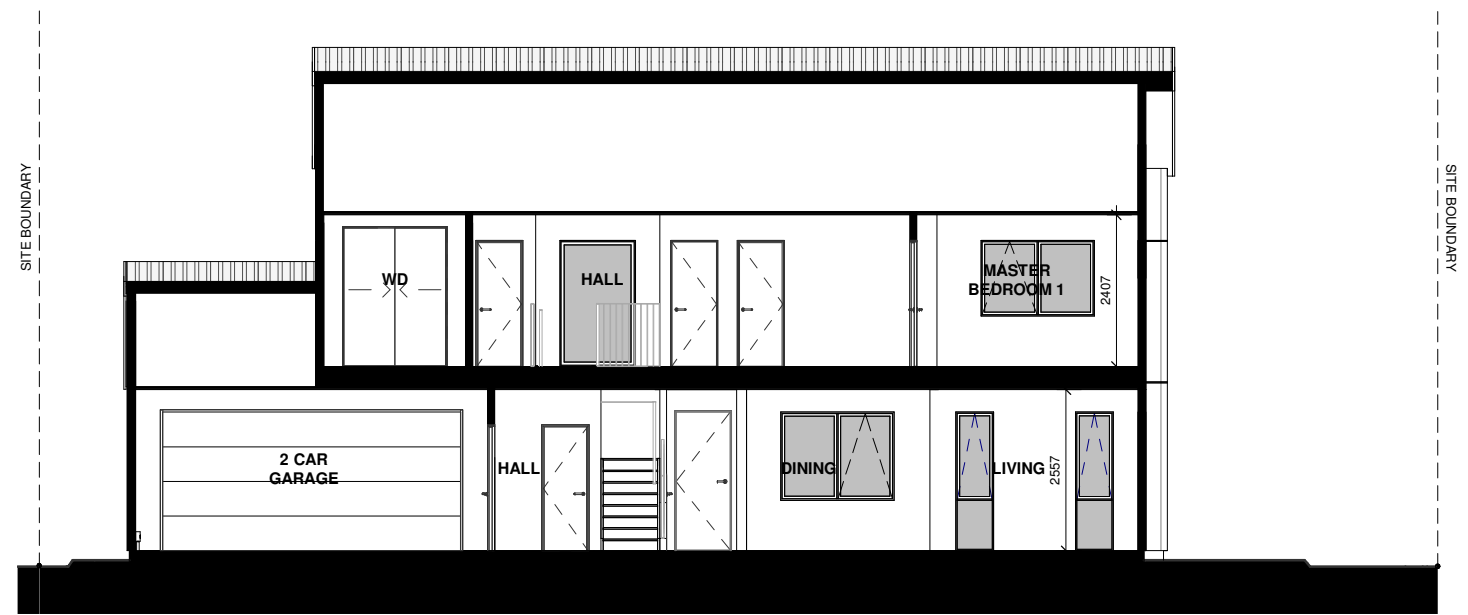
LOT 71 - SECTION B
