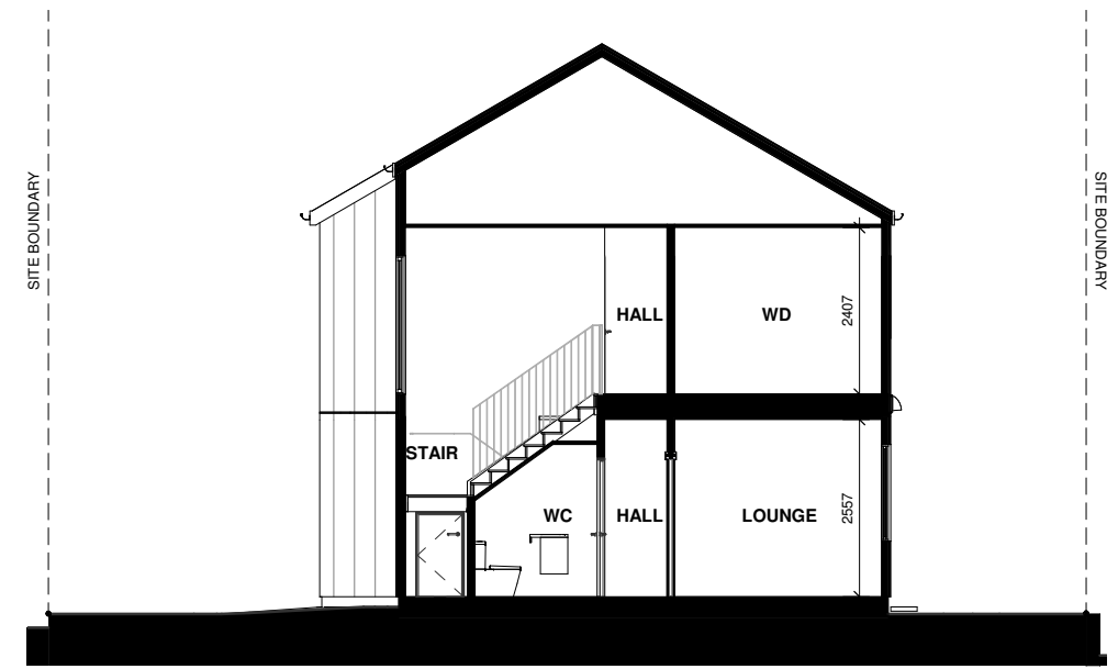
LOT 71 - SECTION C
