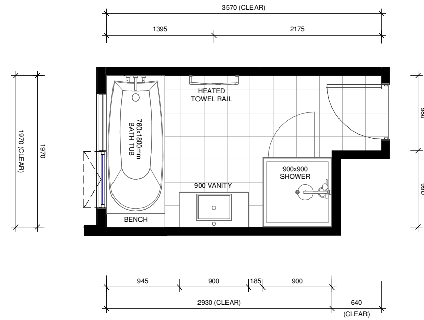
LOT 71 - FIRST FLOOR BATHROOM LAYOUT
