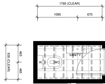
LOT 71 - GROUND FLOOR WC LAYOUT
