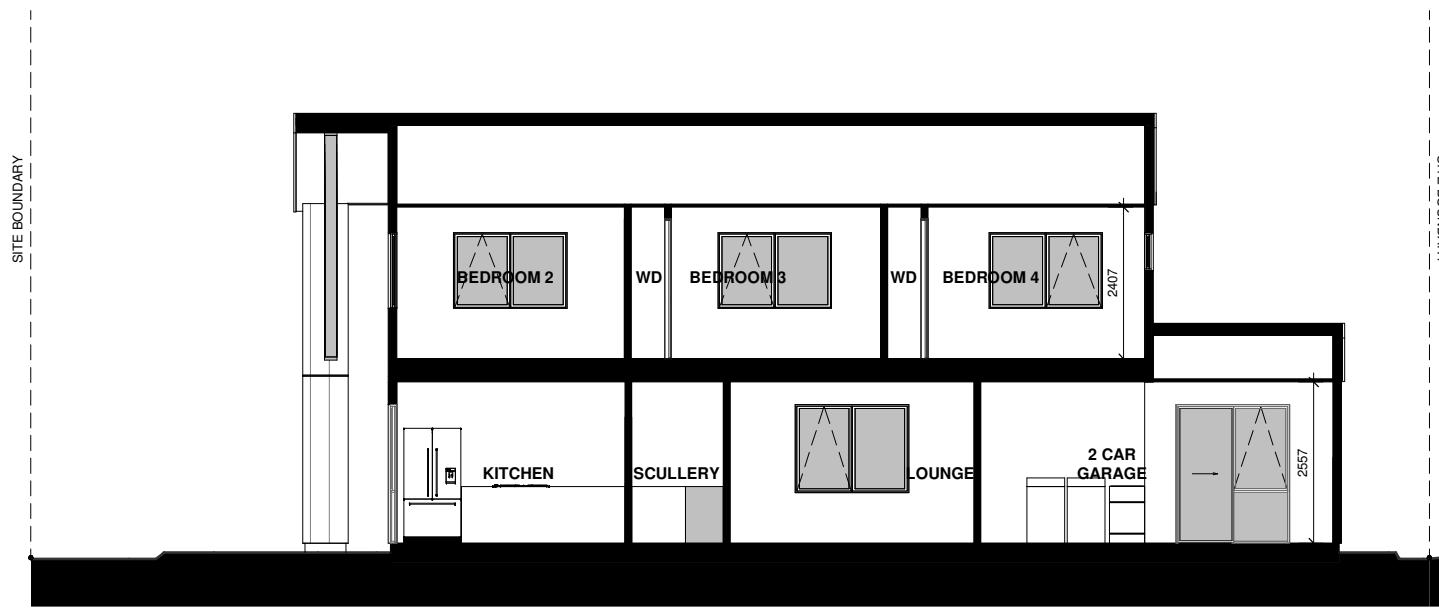
LOT 71 - SECTION A
