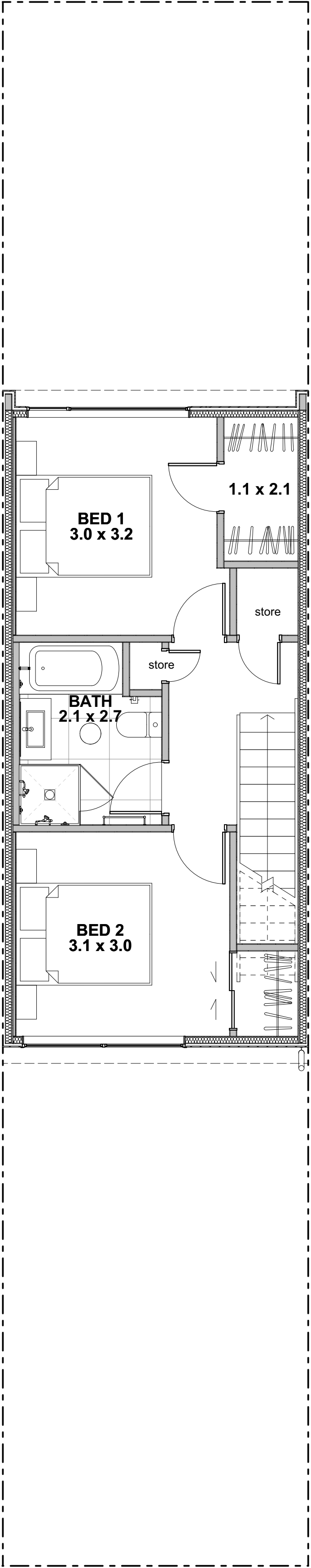
FIRST FLOOR PLAN
