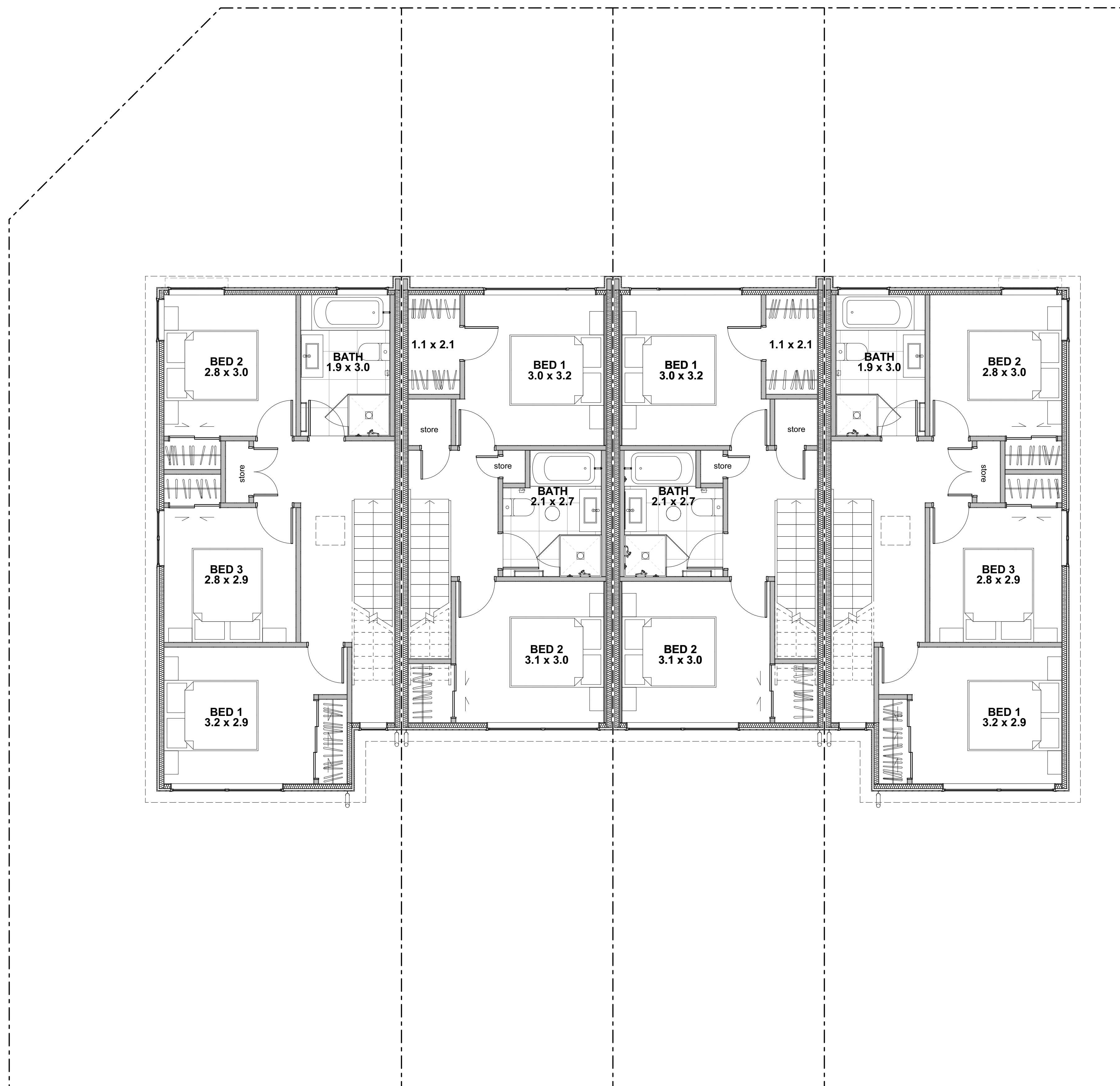
LOT 46 FIRST FLOOR PLAN
