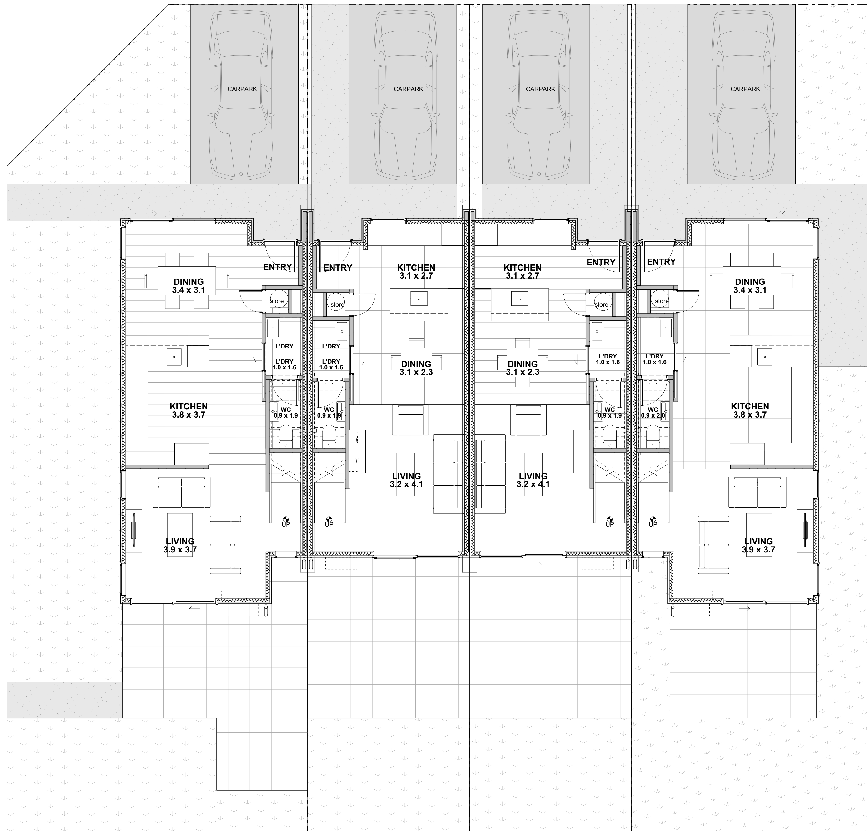
LOT 46 GROUND FLOOR PLAN
