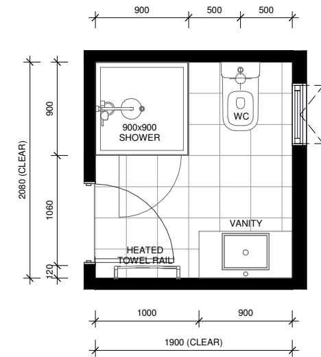
LOT 72 - FIRST FLOOR ENSUITE 2 LAYOUT
