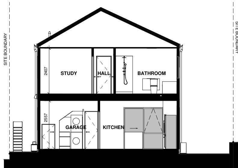
LOT 72 - SECTION D
