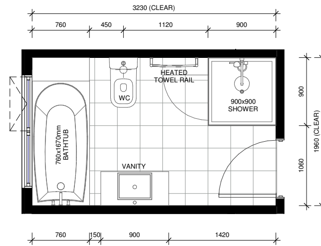
LOT 72 - FIRST FLOOR BATHROOM LAYOUT
