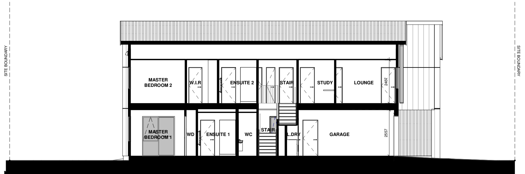
LOT 72 - SECTION B
