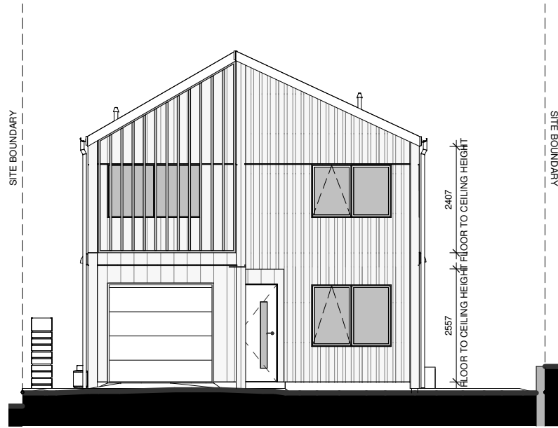
LOT 72 - EAST ELEVATION
