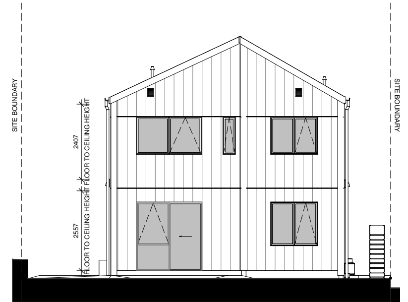
LOT 72 - WEST ELEVATION
