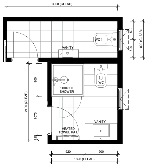
LOT 72 - GROUND FLOOR WC & ENSUITE 1 LAYOUT
