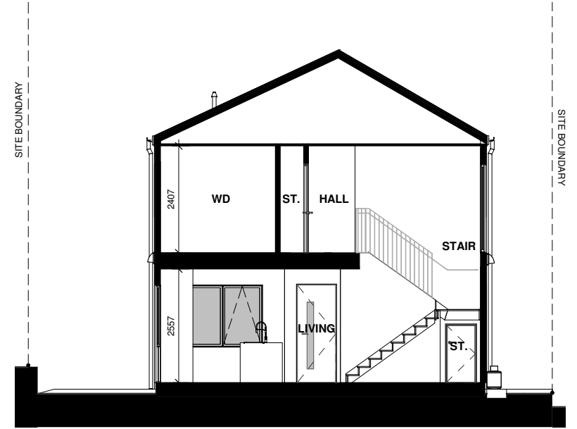
LOT 72 - SECTION C
