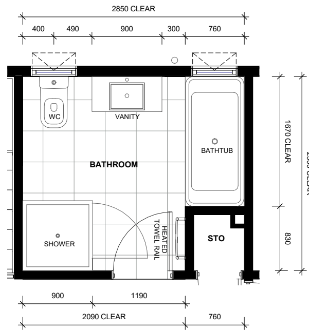
LOT 94 - FIRST FLOOR BATHROOM LAYOUT
