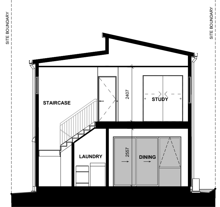
LOT 94 - SECTION C-C
