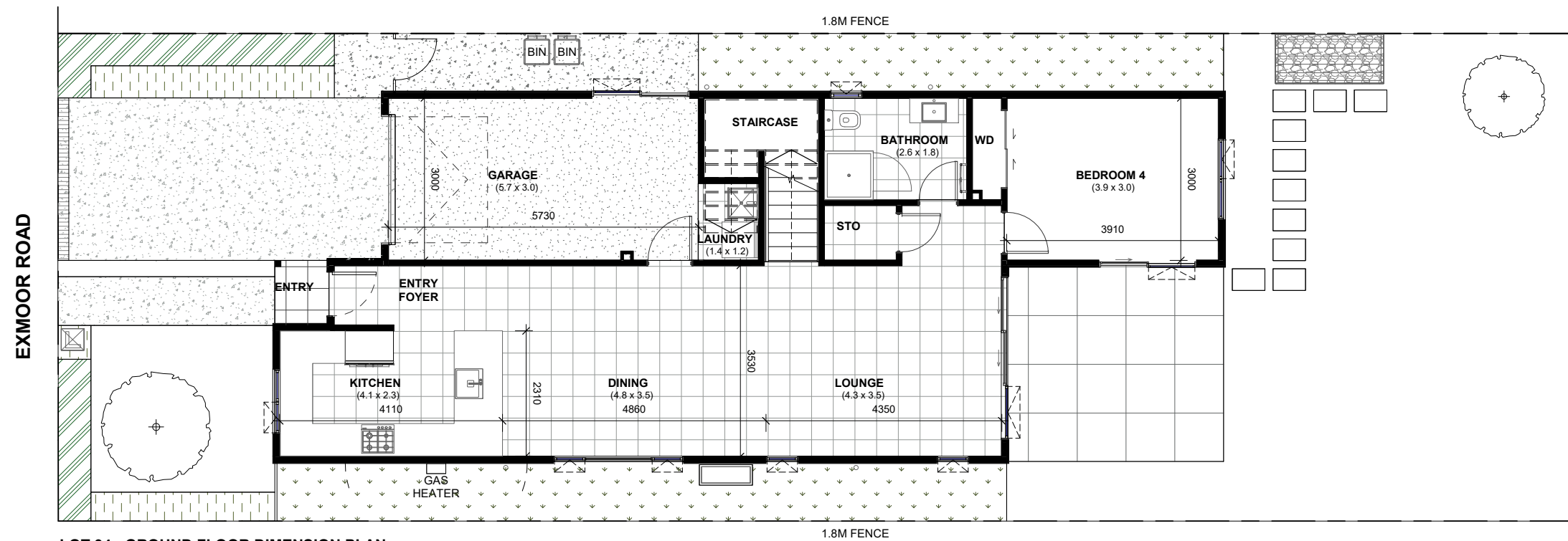
LOT 94 - GROUND FLOOR DIMENSION PLAN
