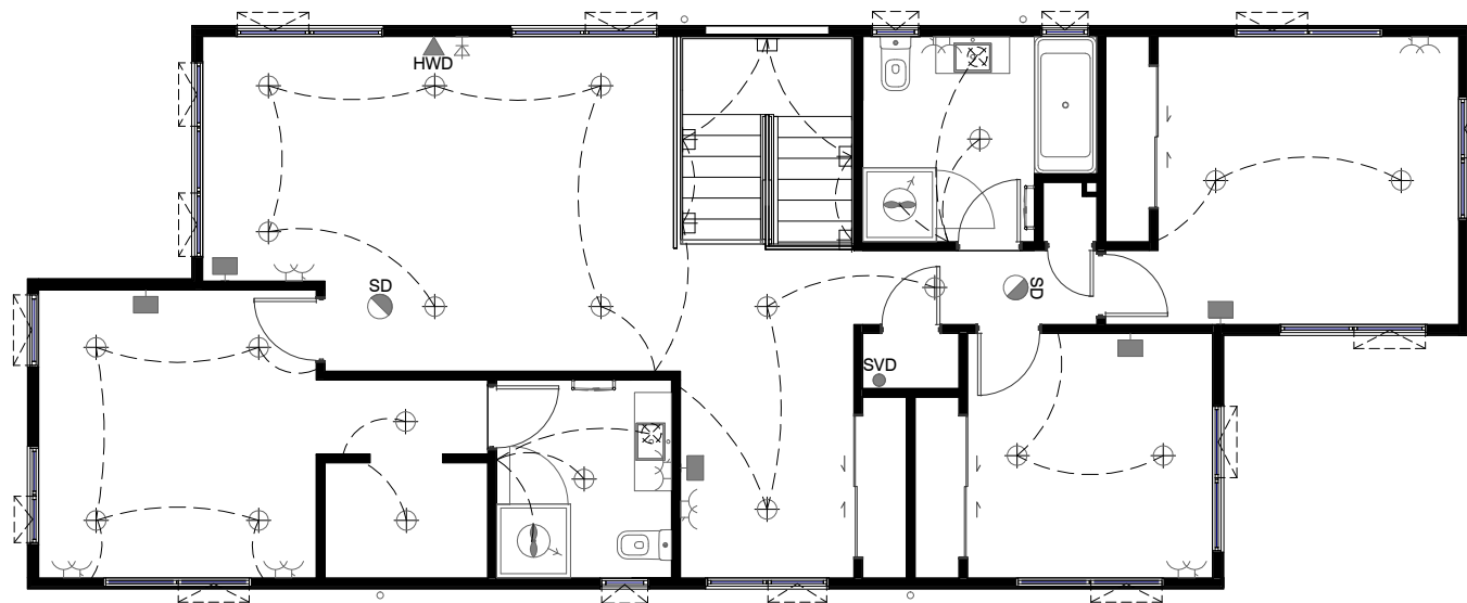
LOT 94 - FIRST FLOOR ELECTRICAL PLAN
