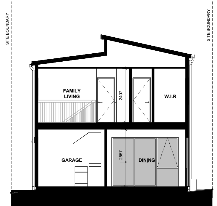
LOT 94 - SECTION D-D
