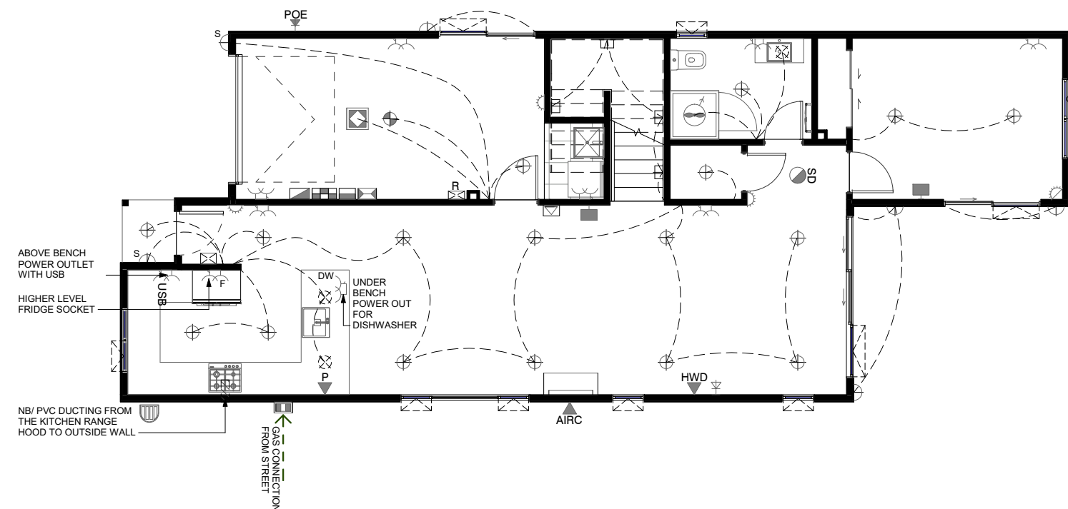
LOT 94 - GROUND FLOOR ELECTRICAL PLAN
