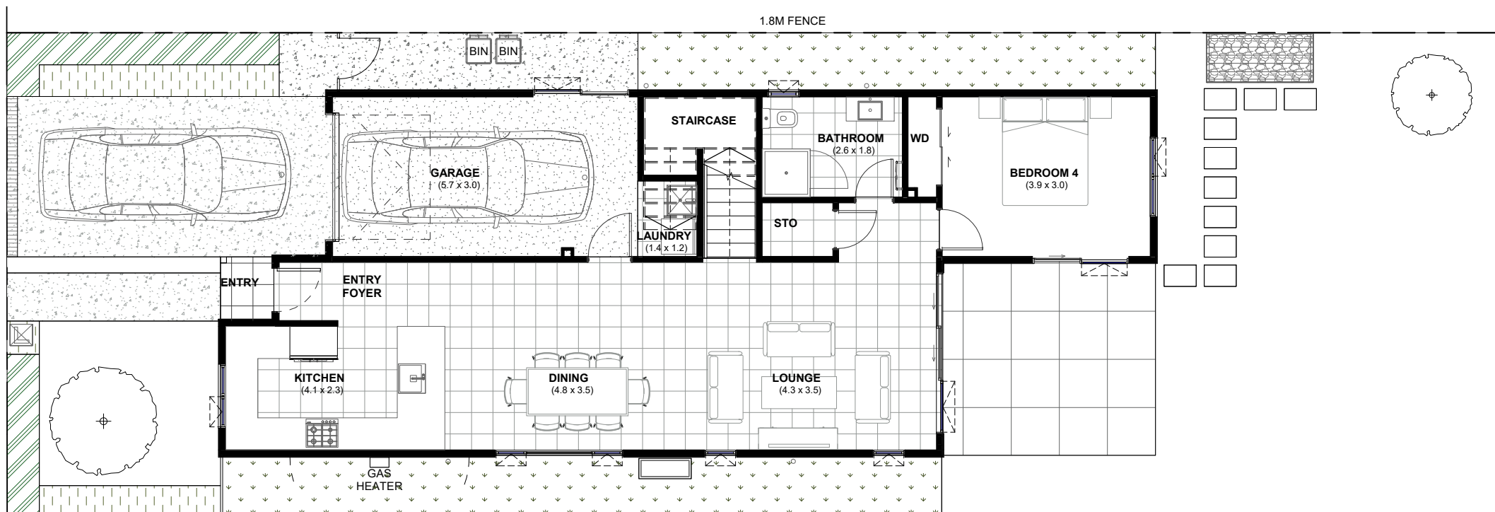
LOT 94 - GROUND FLOOR PLAN
