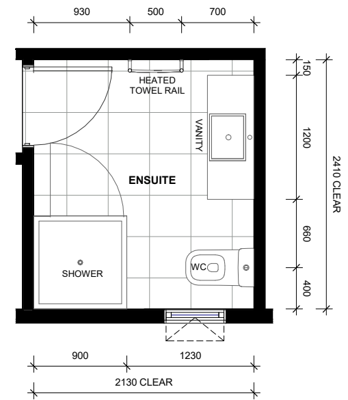
LOT 94 - FIRST FLOOR ENSUITE LAYOUT
