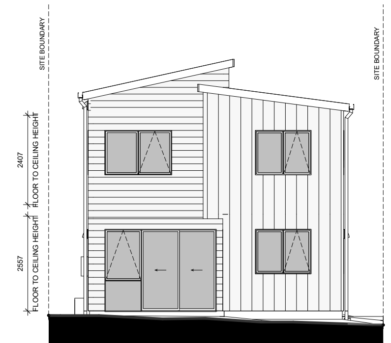
LOT 94 - SOUTH ELEVATION
