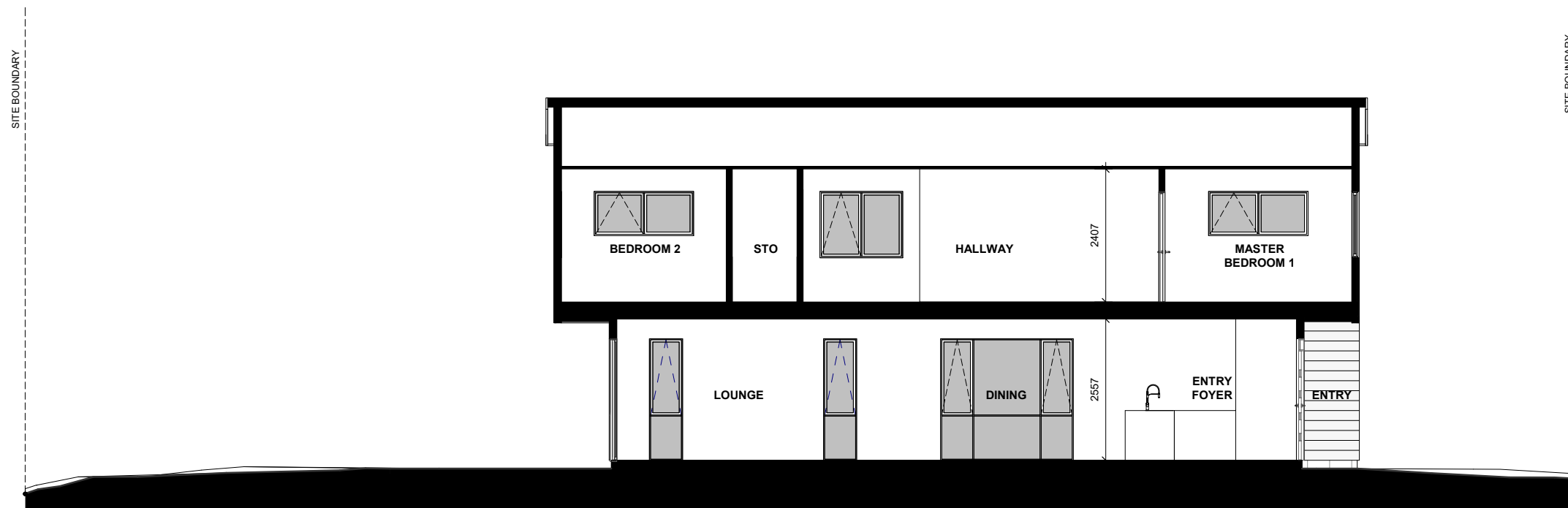
LOT 94 - SECTION B-B
