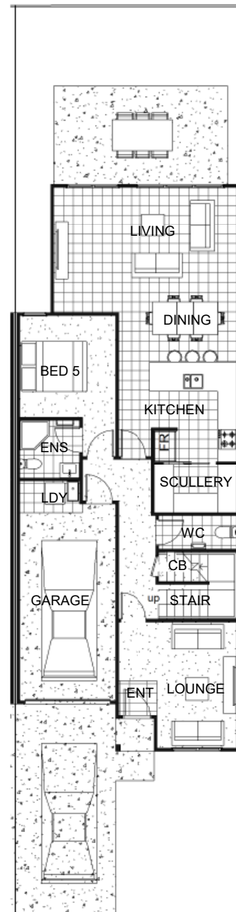
Ground floor
