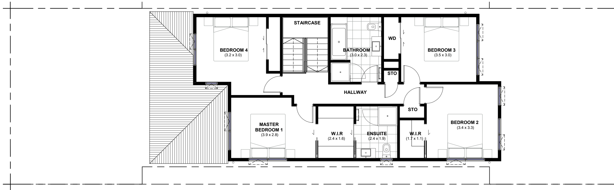
LOT 70 - FIRST FLOOR PLAN
