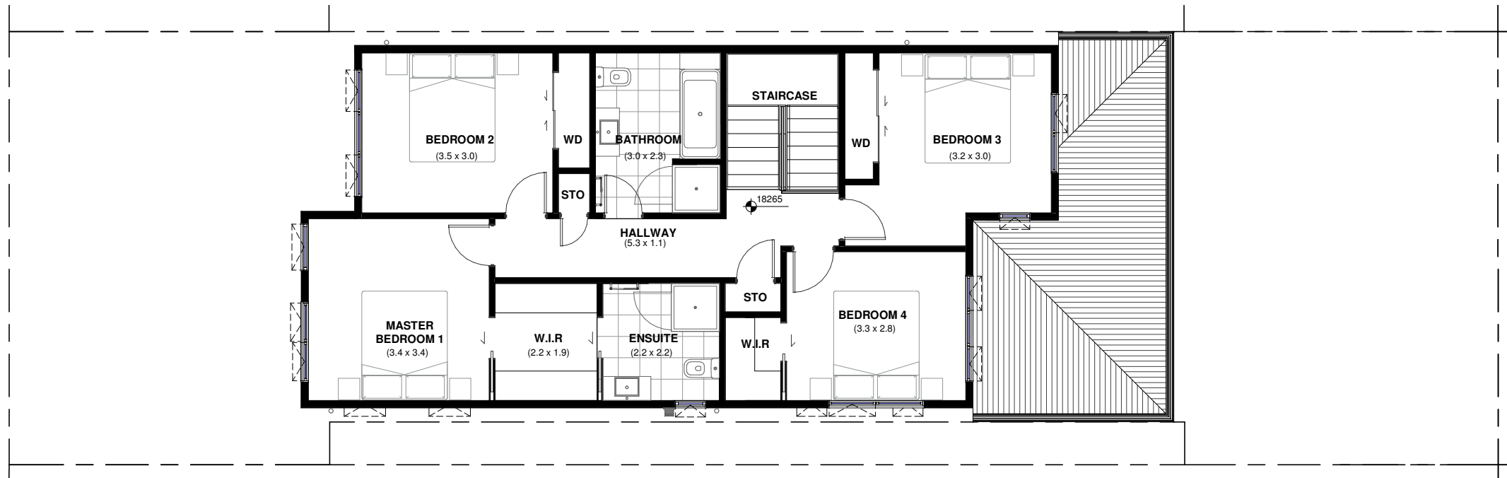
LOT 61_FIRST FLOOR LEVEL
