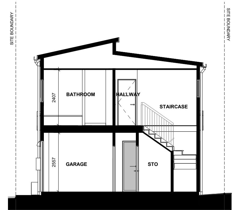
LOT 88 - SECTION C-C
