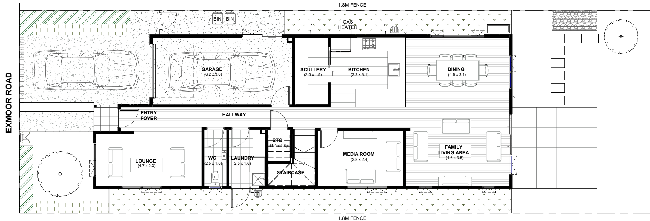
LOT 88 - GROUND FLOOR PLAN
