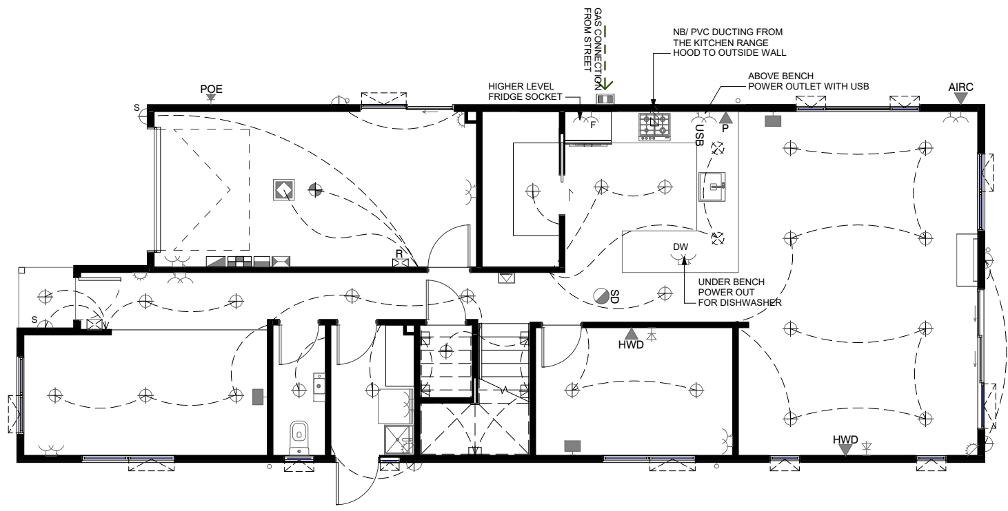
LOT 88 - GROUND FLOOR ELECTRICAL PLAN
