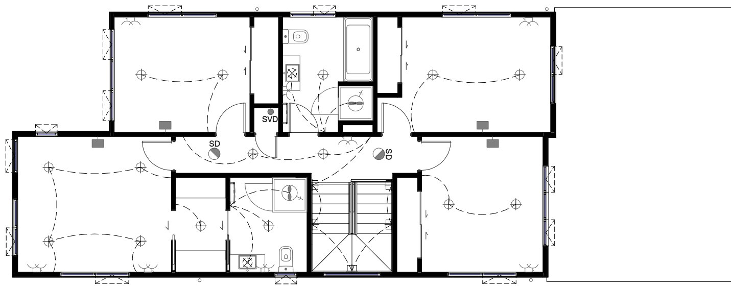
LOT 88 - FIRST FLOOR ELECTRICAL PLAN
