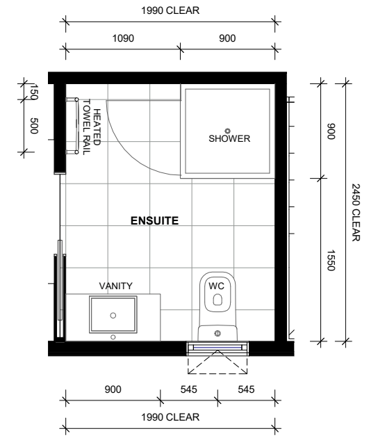
LOT 88 - FIRST FLOOR ENSUITE LAYOUT
