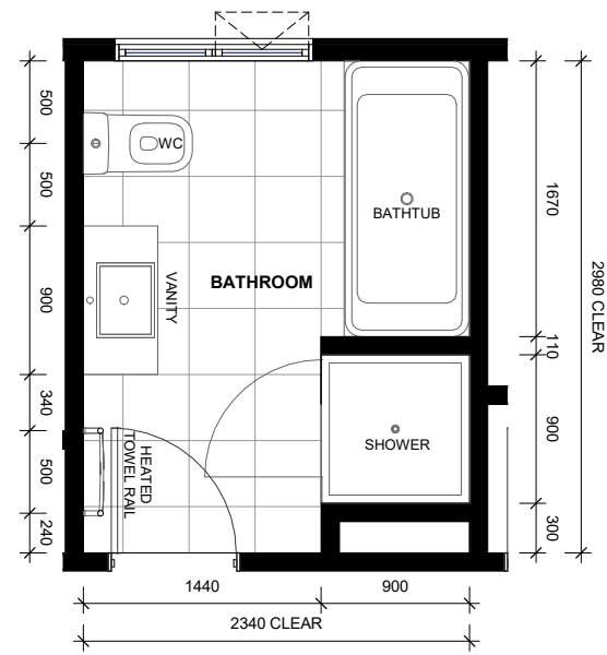
LOT 88 - FIRST FLOOR BATHROOM LAYOUT
