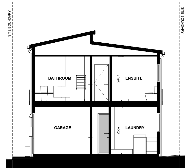
LOT 88 - SECTION D-D
