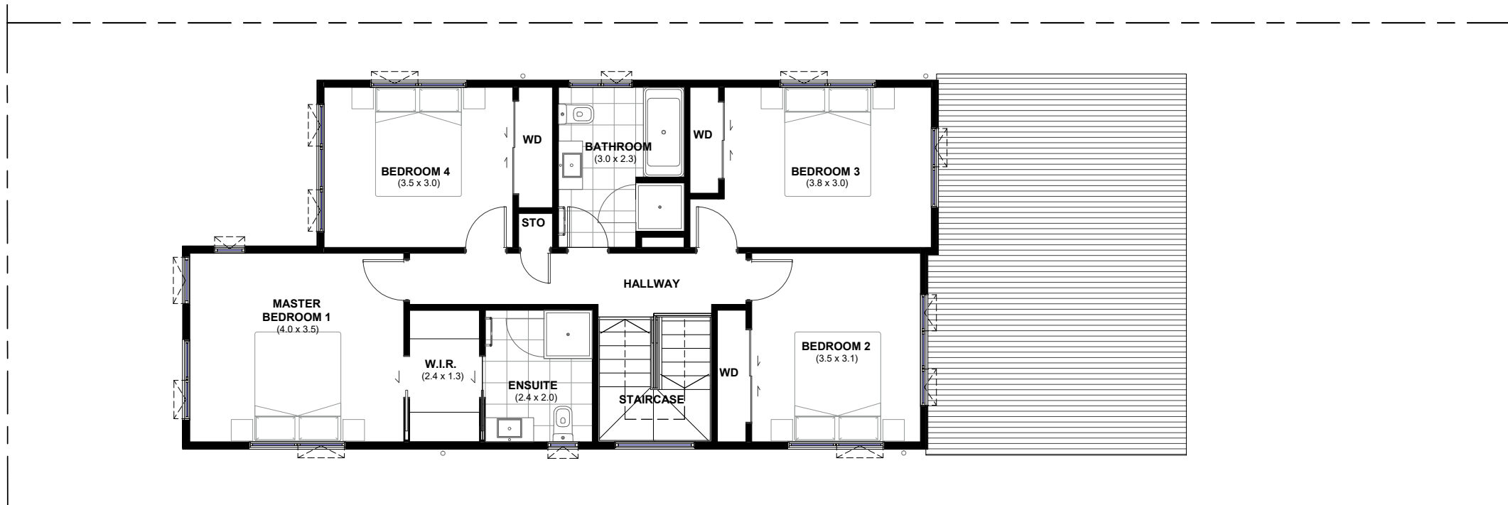
LOT 88 - FIRST FLOOR PLAN
