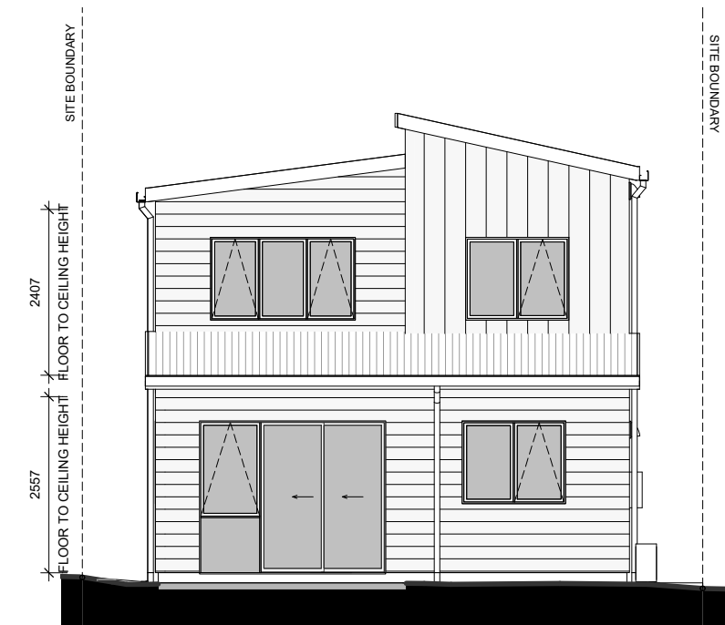
LOT 88 - SOUTH ELEVATION
