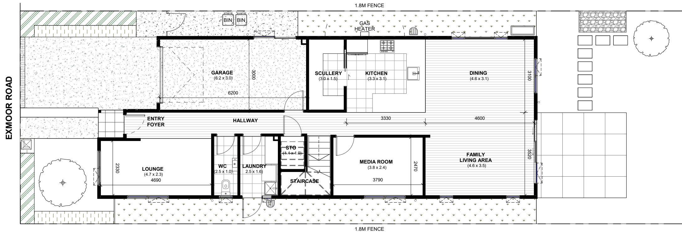
LOT 88 - GROUND FLOOR DIMENSION PLAN
