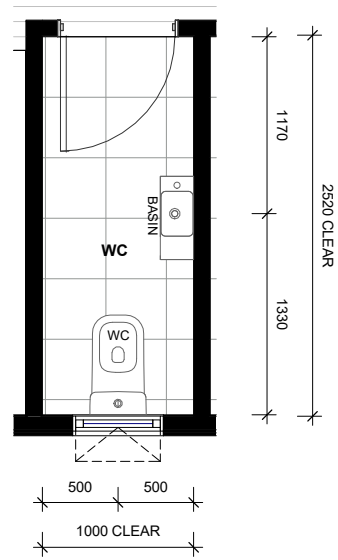
LOT 88 - GROUND FLOOR WC LAYOUT
