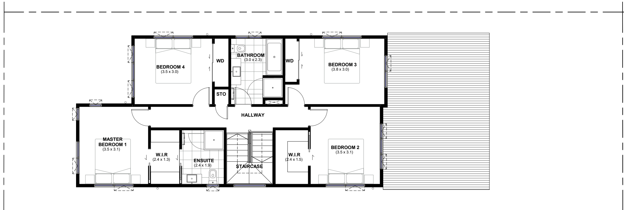
LOT 55 - FIRST FLOOR PLAN
