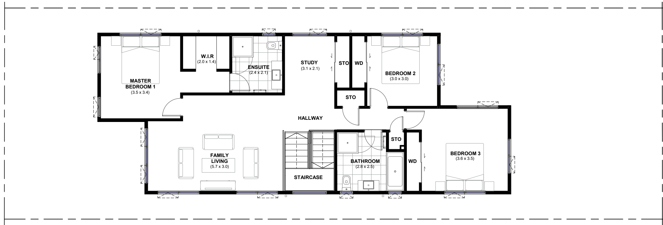
LOT 56 - FIRST FLOOR PLAN
