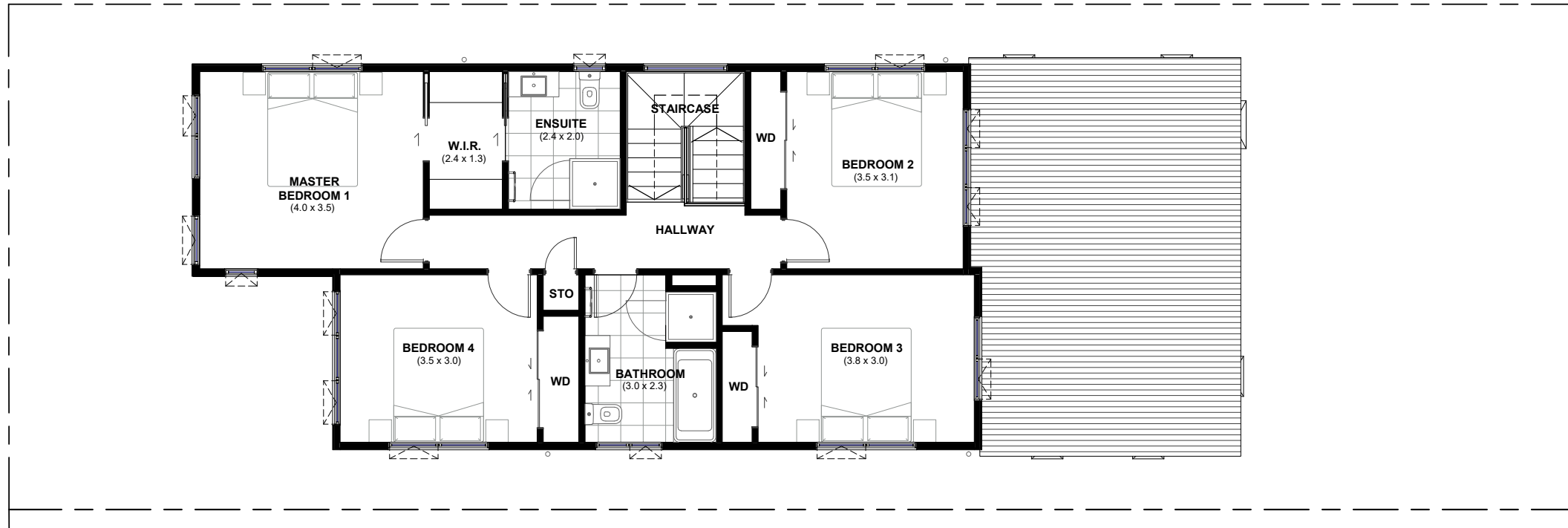
LOT 97 - FIRST FLOOR PLAN
