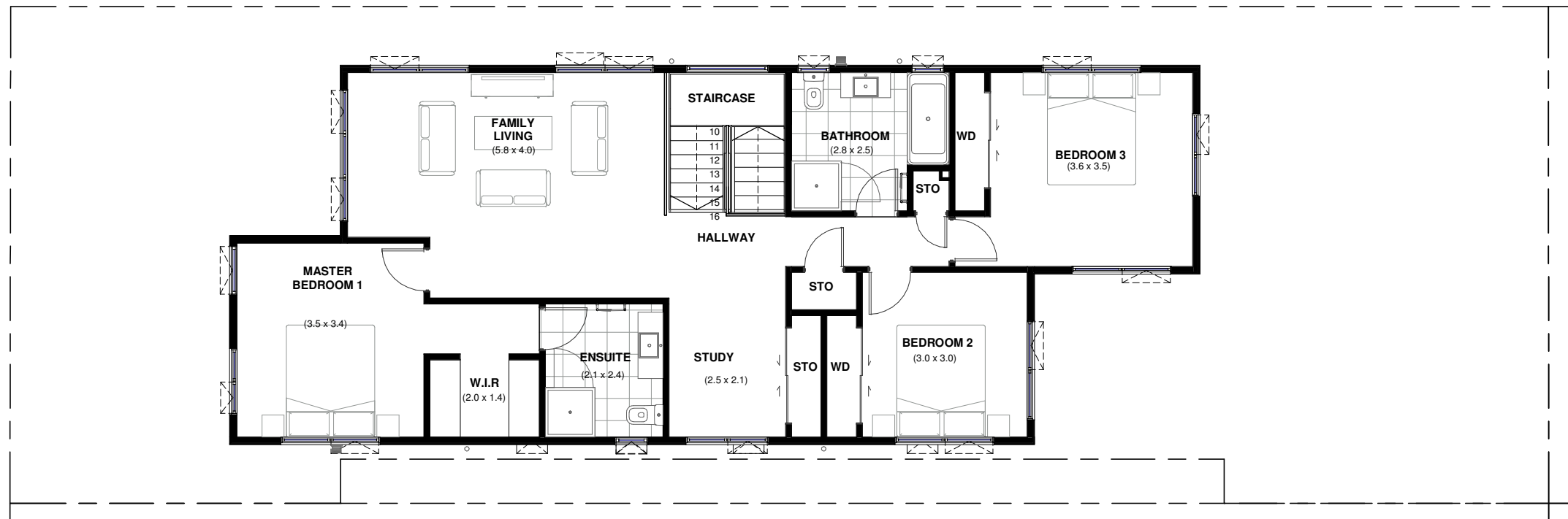
LOT 62_FIRST FLOOR LEVEL
