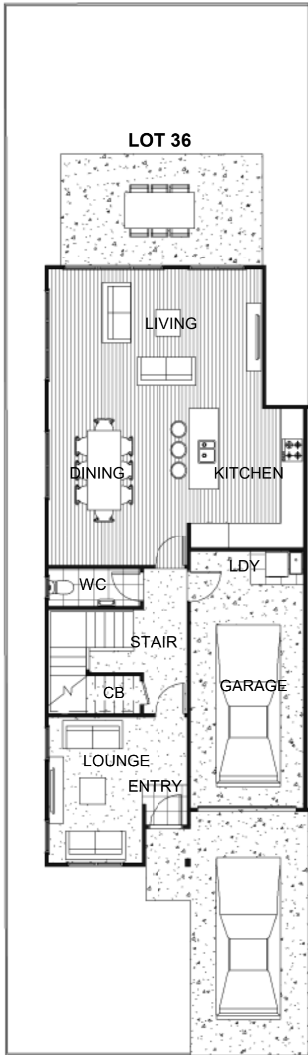
LOT 36 LOWER FLOOR PLAN 1 : 100
