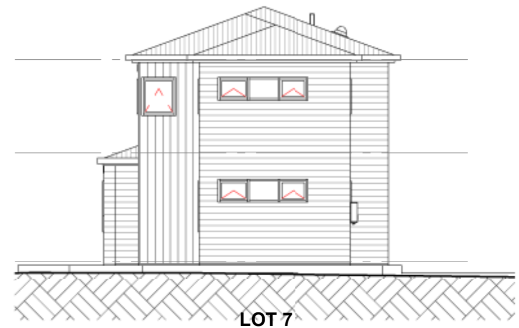
LOT 7 WEST ELEVATION 1 : 100
