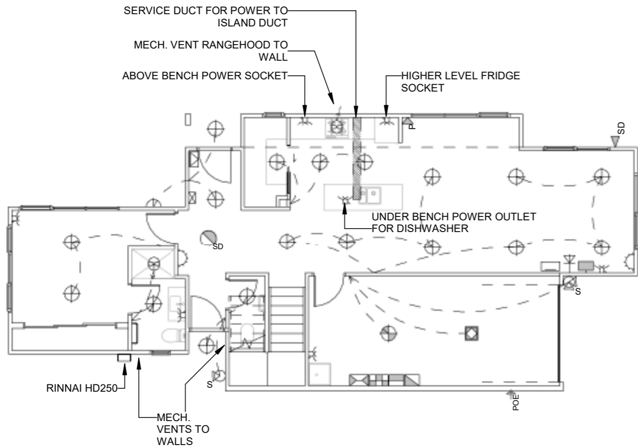
LOT 7 LOWER ELECTRICAL LAYOUT PLAN
