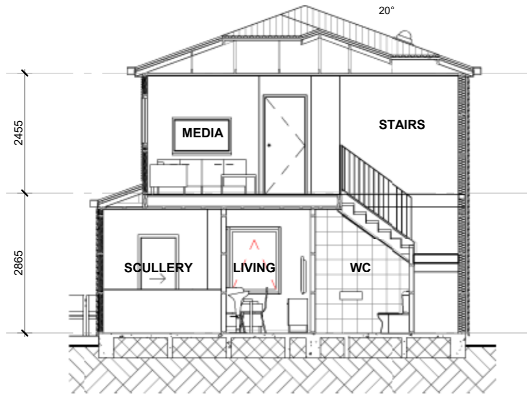
LOT 7 CROSS SECTION
