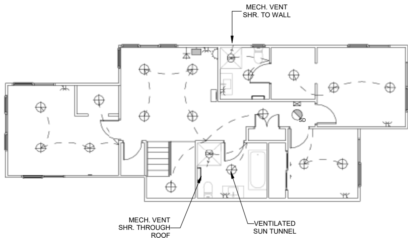
LOT 7 UPPER ELECTRICAL LAYOUT PLAN
