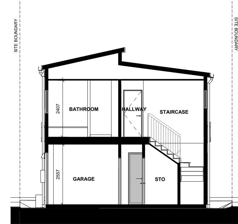
LOT 28 - SECTION C-C
