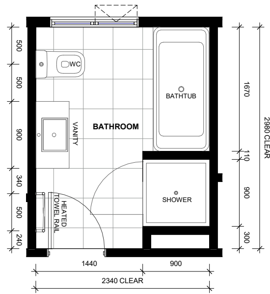
LOT 28 - FIRST FLOOR BATHROOM LAYOUT
