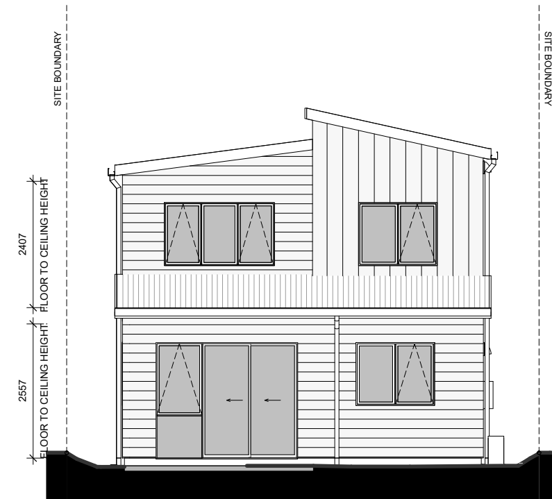
LOT 28 - SOUTH ELEVATION
