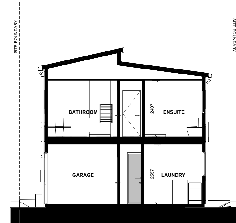
LOT 28 - SECTION D-D
