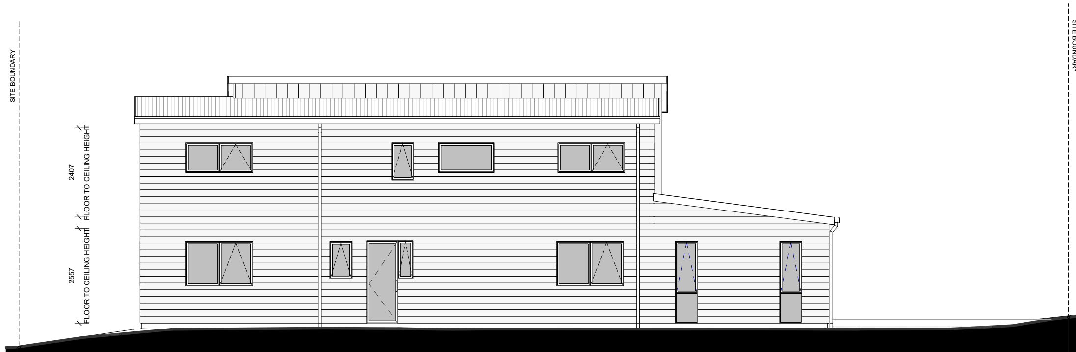
LOT 28 - WEST ELEVATION
