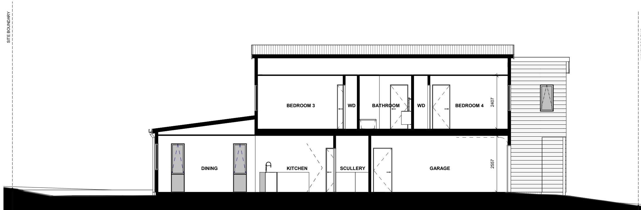
LOT 28 - SECTION B-B
