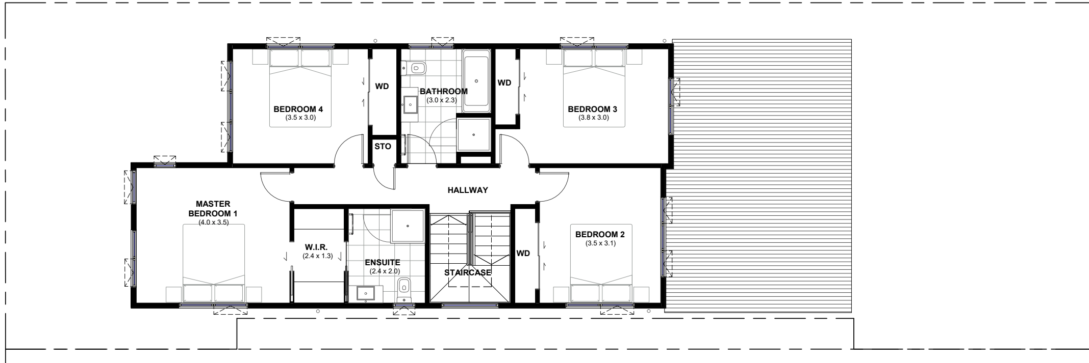
LOT 28 - FIRST FLOOR PLAN
