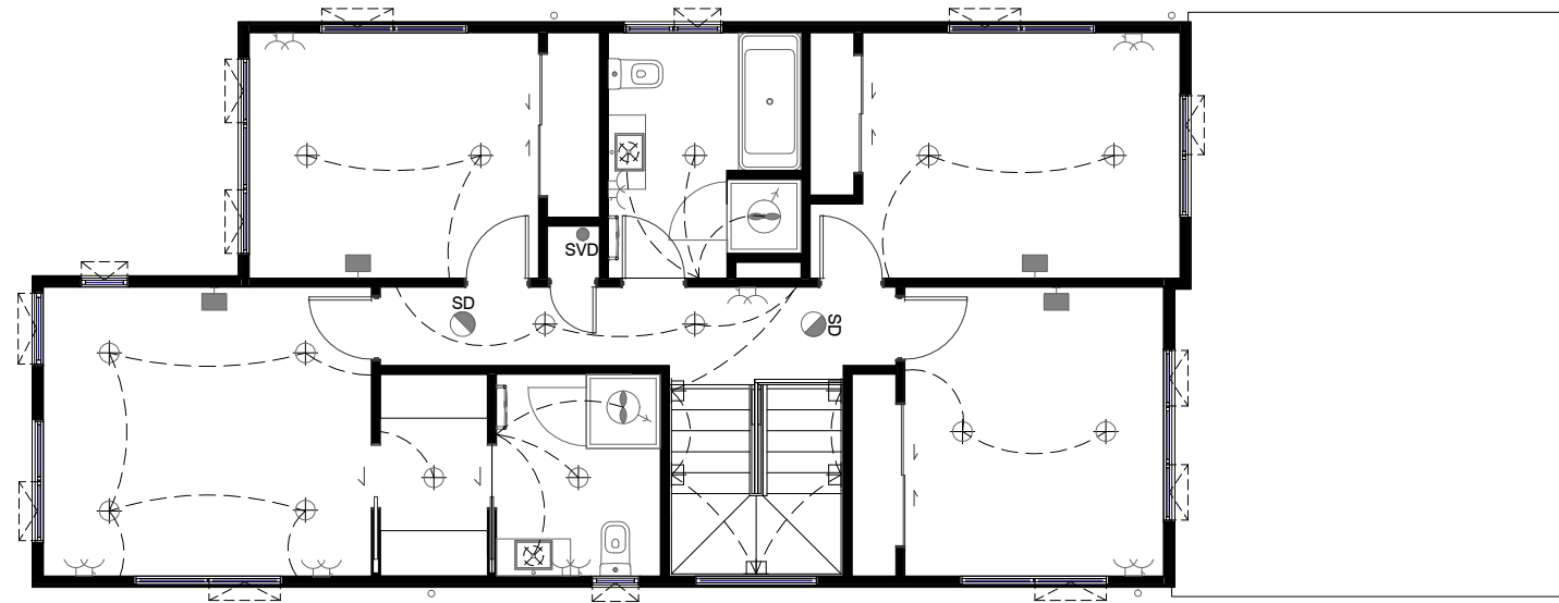
LOT 28 - FIRST FLOOR ELECTRICAL PLAN
