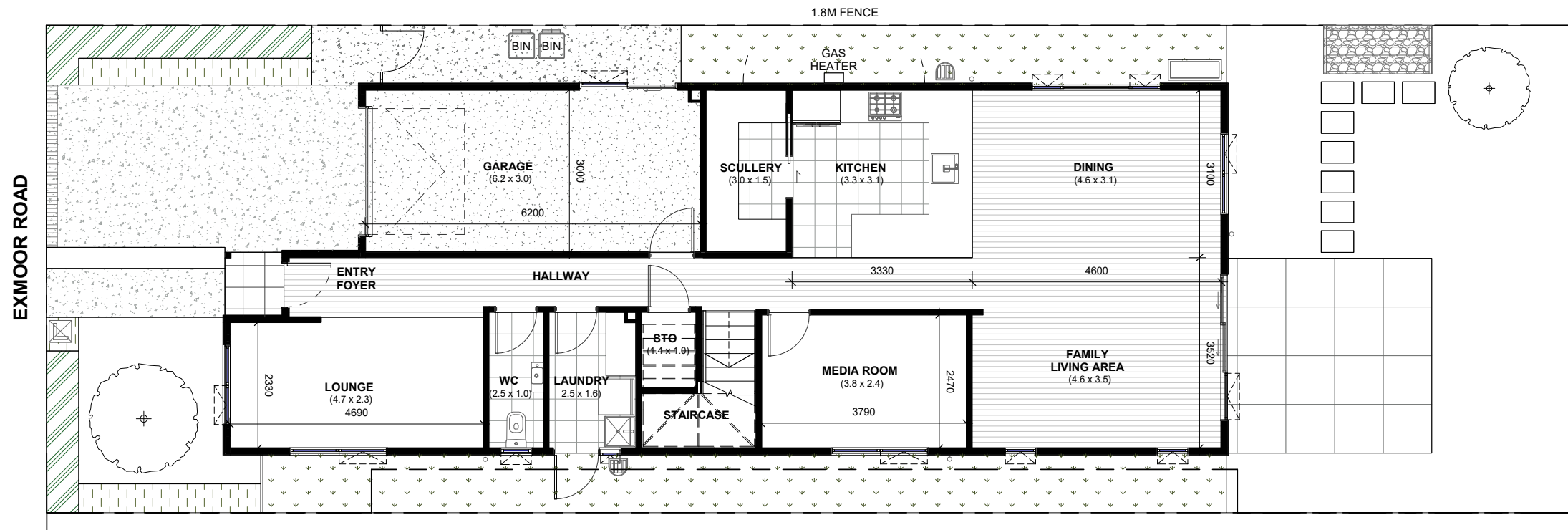
LOT 28 - GROUND FLOOR DIMENSION PLAN
