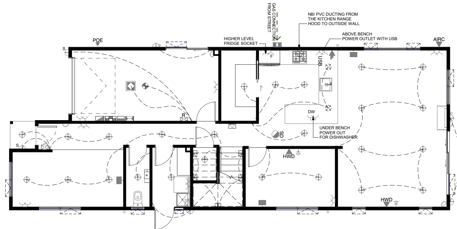
LOT 28 - GROUND FLOOR ELECTRICAL PLAN
