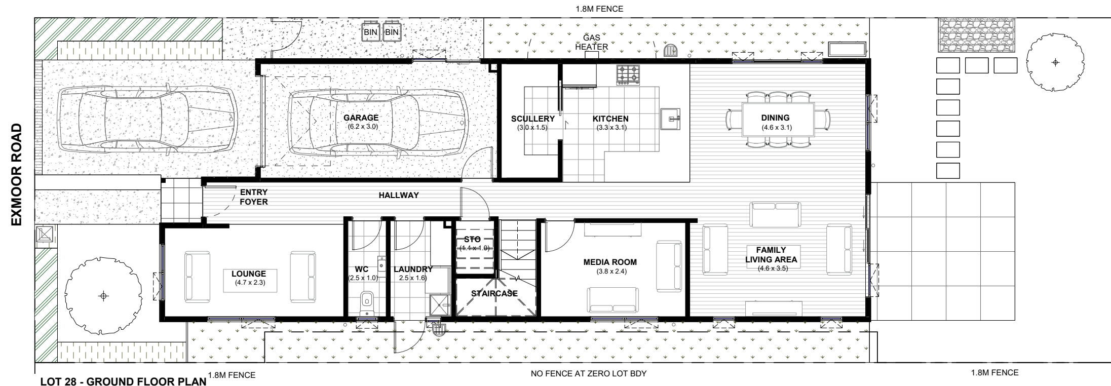
LOT 28 - GROUND FLOOR PLAN
