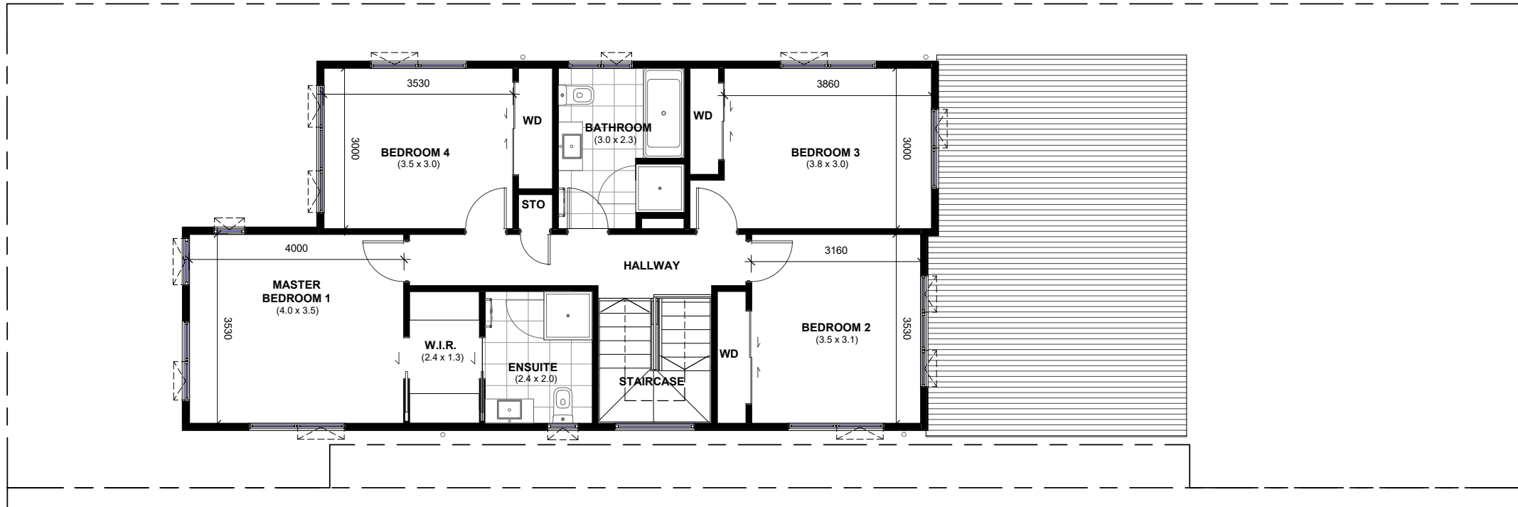
LOT 28 - FIRST FLOOR DIMENSION PLAN
