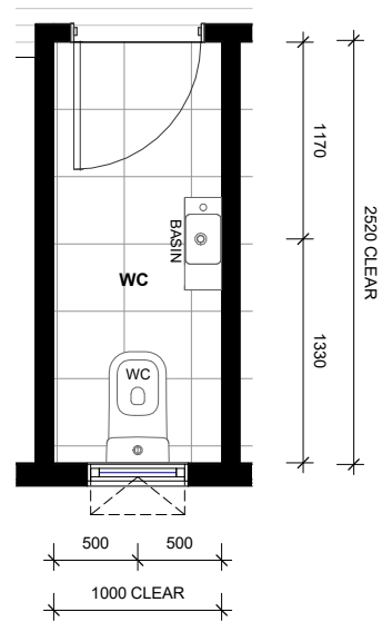
LOT 28 - GROUND FLOOR WC LAYOUT
