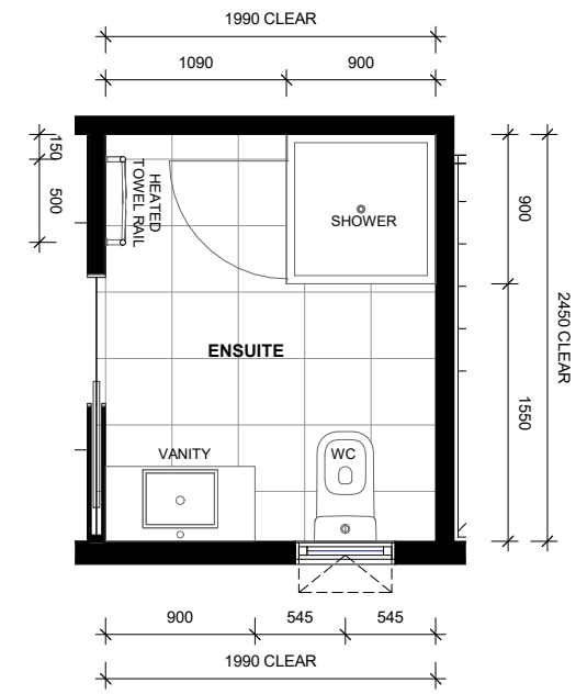
LOT 28 - FIRST FLOOR ENSUITE LAYOUT
