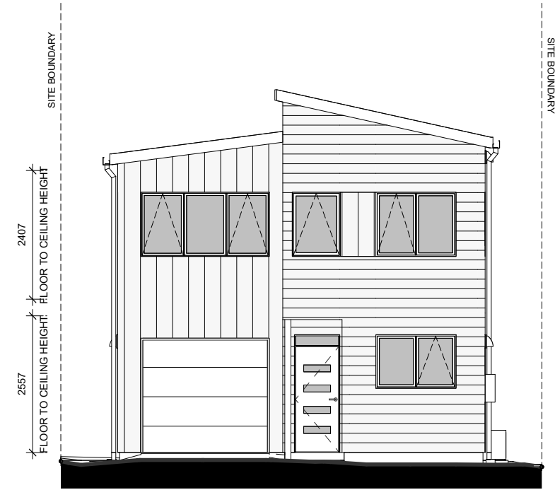
LOT 19 - SOUTH ELEVATION
