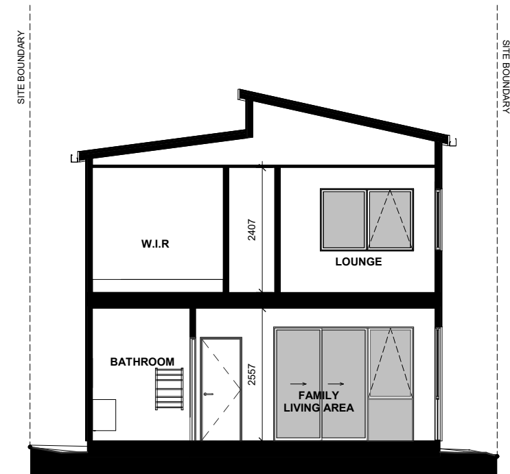
LOT 19 - SECTION D-D
