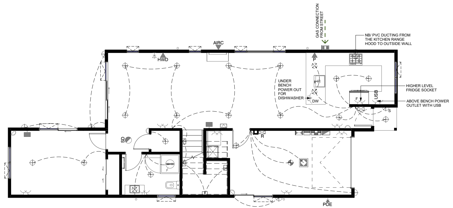
LOT 19 - GROUND FLOOR ELECTRICAL PLAN
