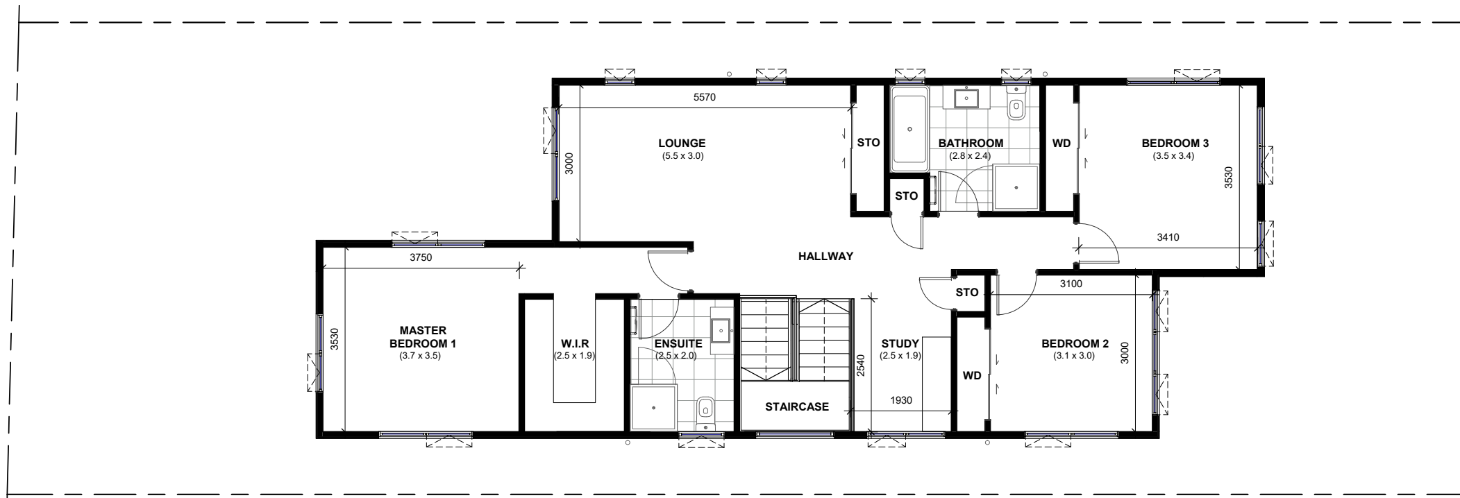
LOT 19 - FIRST FLOOR DIMENSION PLAN
