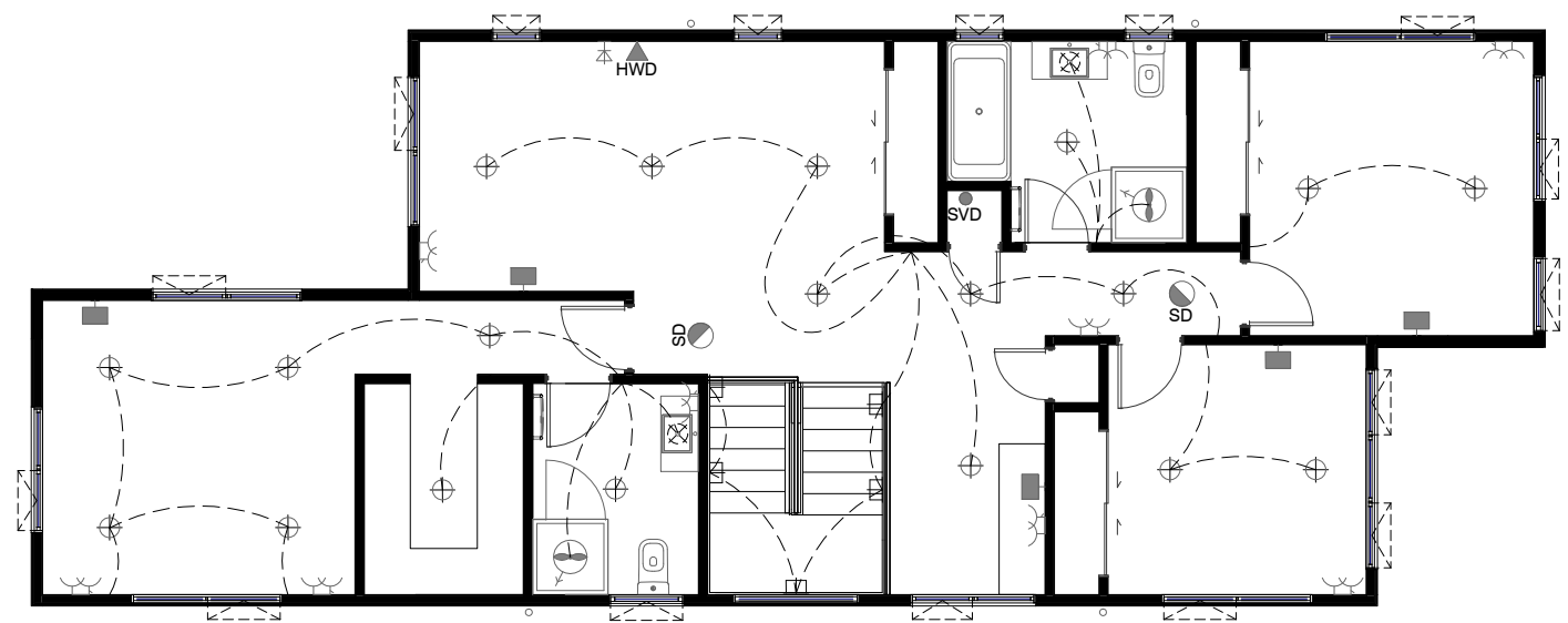
LOT 19 - FIRST FLOOR ELECTRICAL PLAN
