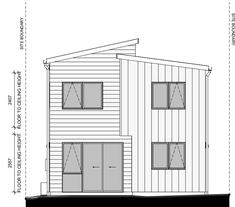
LOT 19 - NORTH ELEVATION
