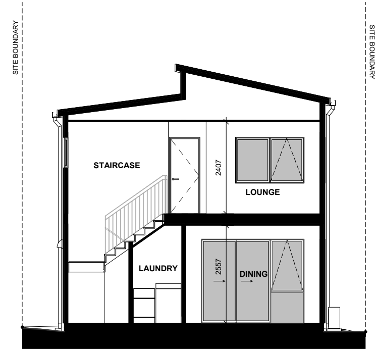
LOT 19 - SECTION C-C
