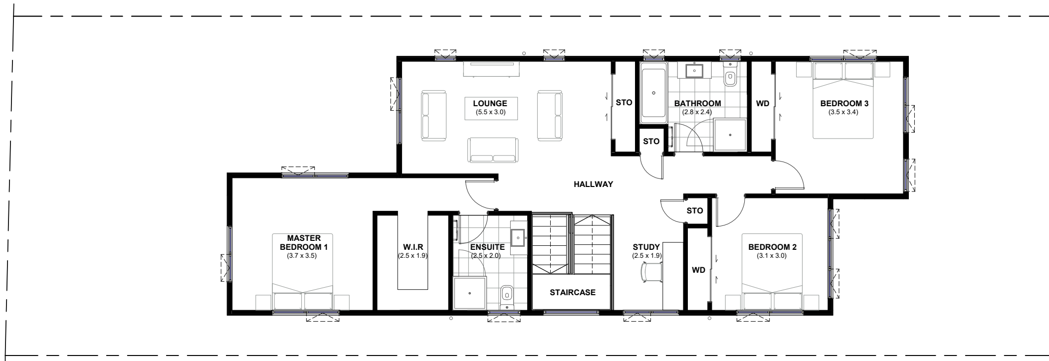
LOT 19 - FIRST FLOOR PLAN
