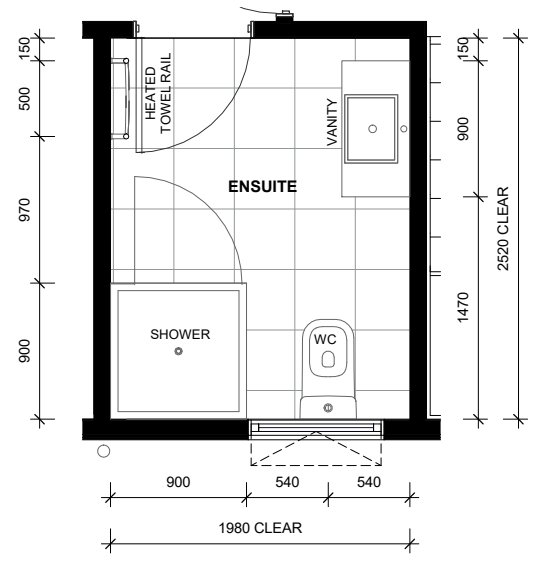
LOT 19 - FIRST FLOOR ENSUITE LAYOUT
