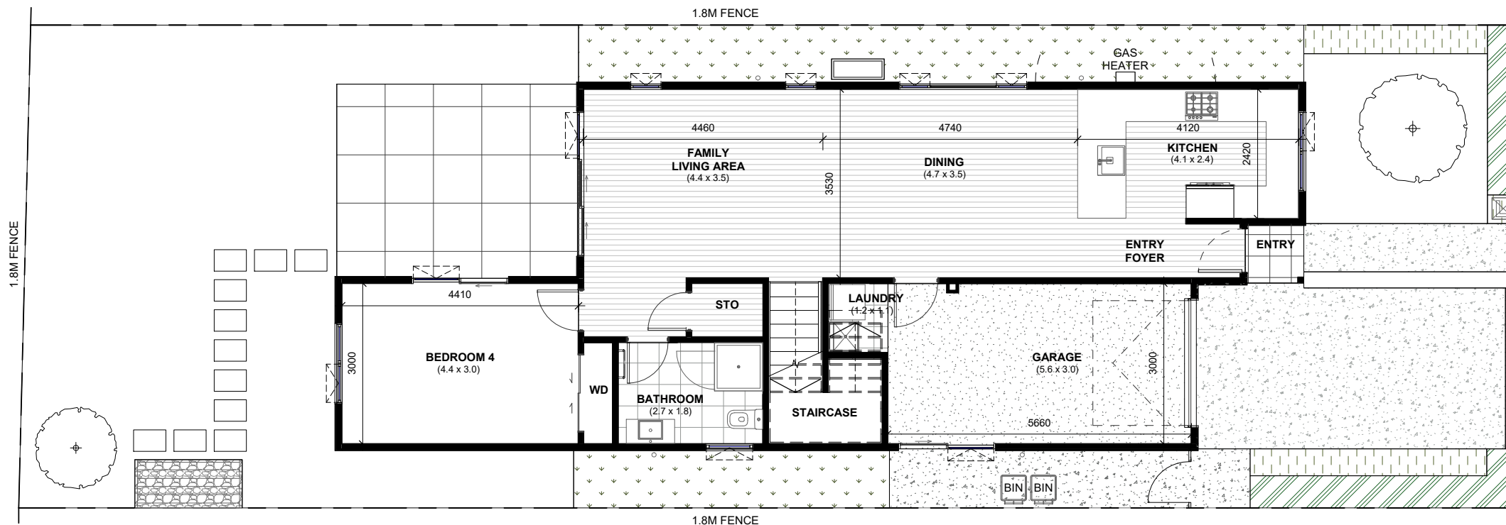
LOT 19 - GROUND FLOOR DIMENSION PLAN
