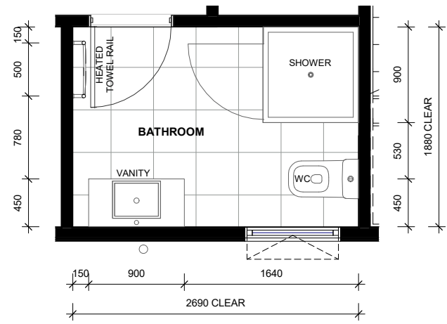
LOT 19 - GROUND FLOOR BATHROOM LAYOUT
