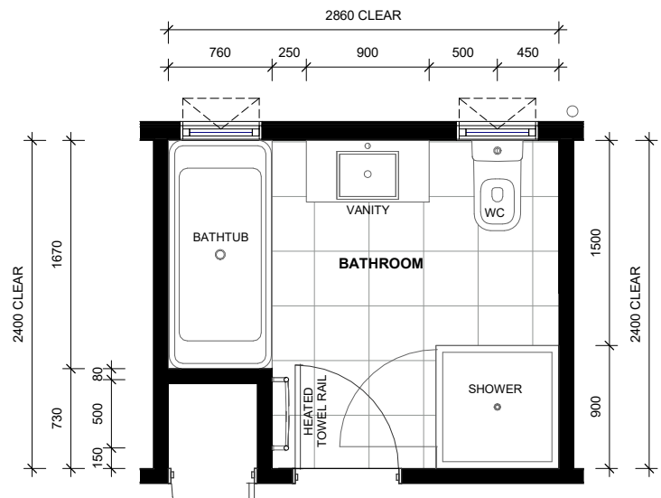
LOT 19 - FIRST FLOOR BATHROOM LAYOUT
