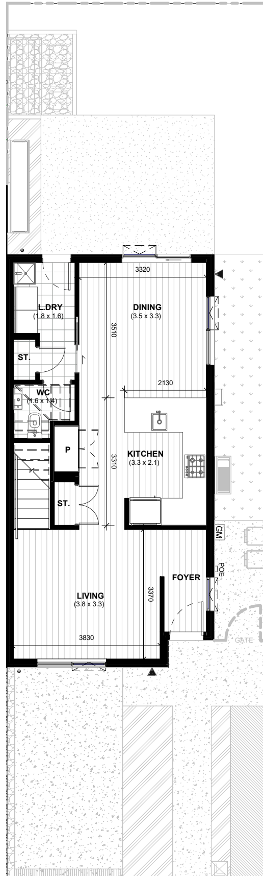
LOT 112- GROUND FLOOR DIMENSION PLAN
