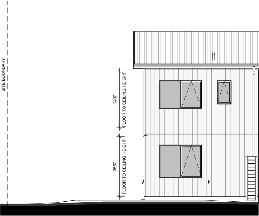
LOT 109 - SOUTH ELEVATION
