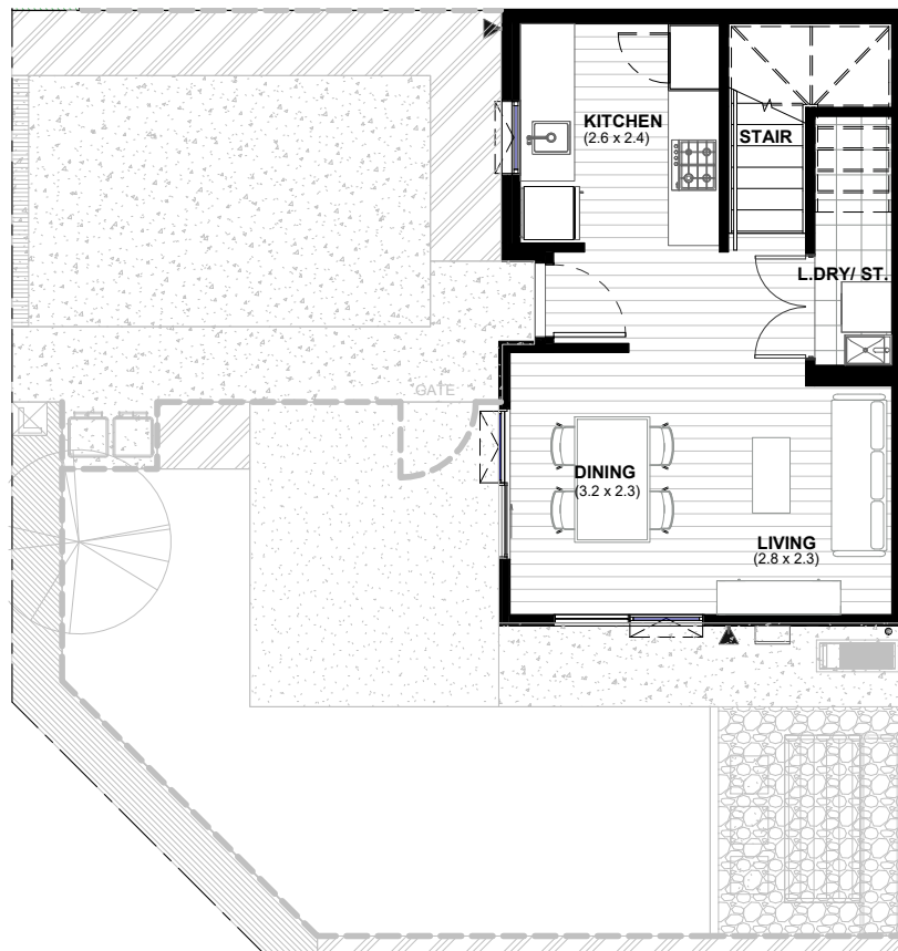
LOT 109 - GROUND FLOOR PLAN
