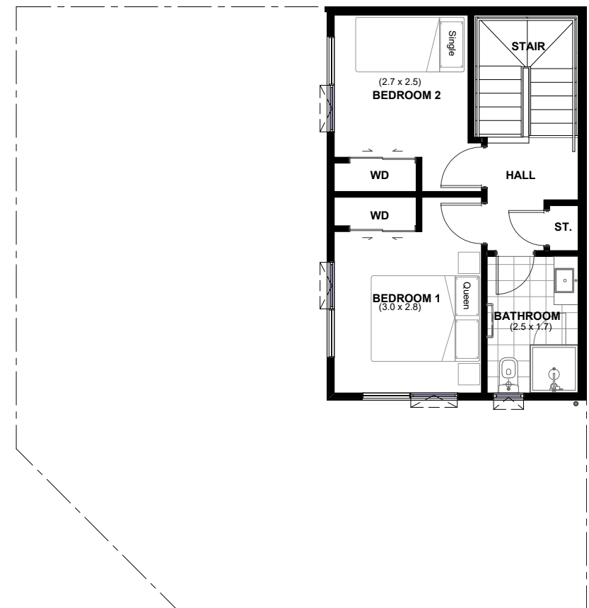
LOT 109 - FIRST FLOOR PLAN
