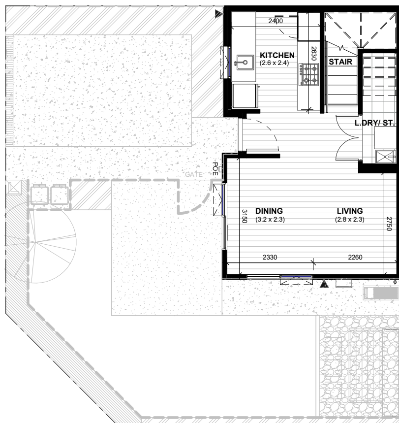
LOT 109 - GROUND FLOOR DIMENSION PLAN
