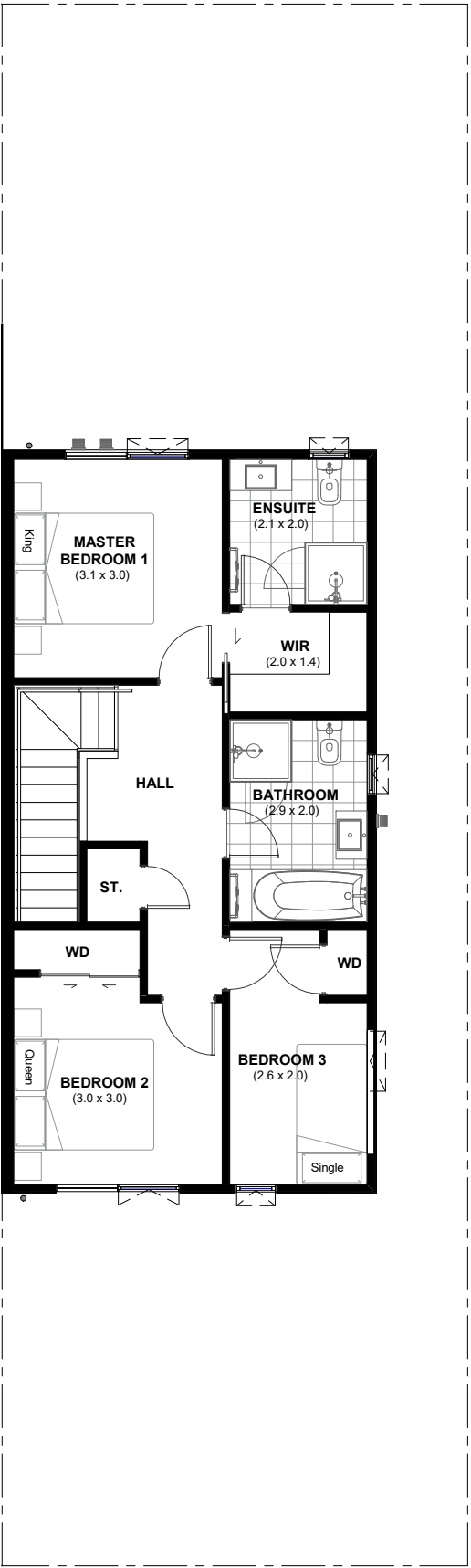
LOT 112 - FIRST FLOOR PLAN
