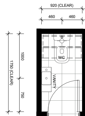
LOT 111 - GROUND FLOOR WC LAYOUT
