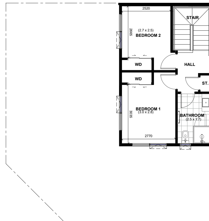
LOT 109 - FIRST FLOOR DIMENSION PLAN
