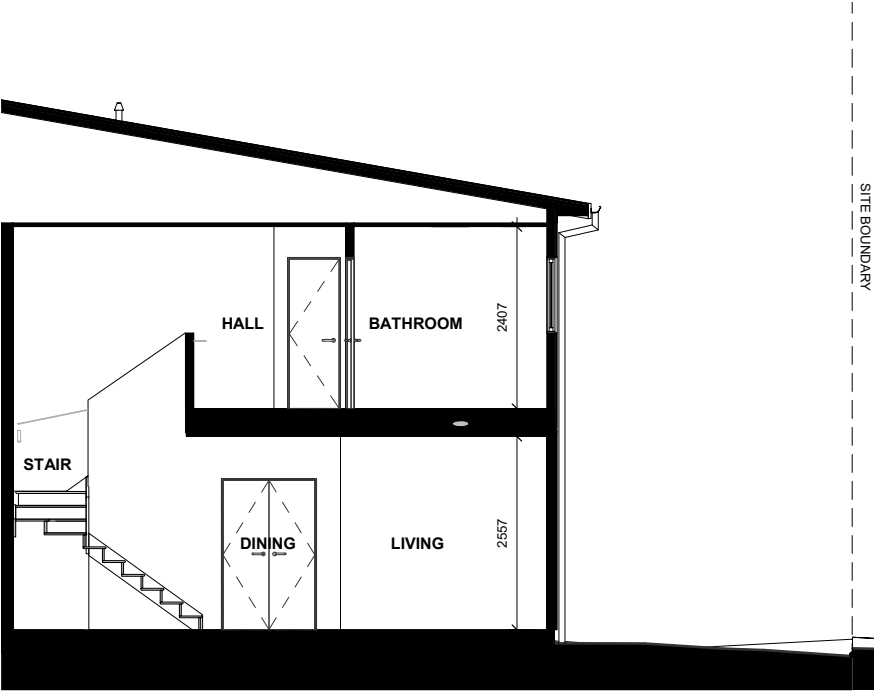
LOT 109 - SECTION B - B
