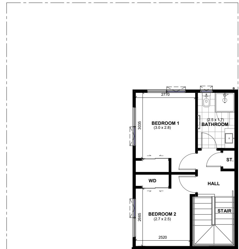
LOT 110 - FIRST FLOOR DIMENSION PLAN
