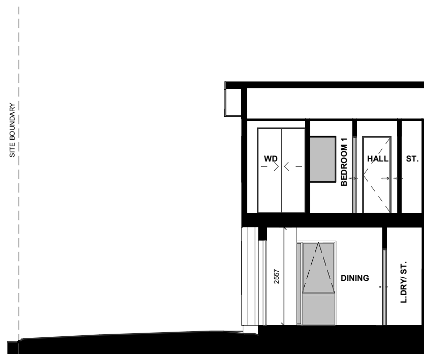
LOT 110 - SECTION A - A
