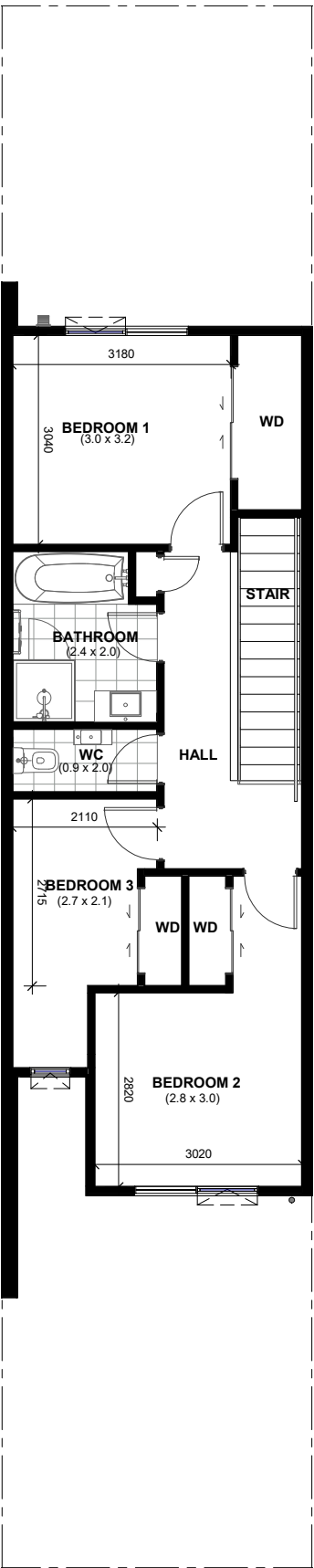
LOT 111 - FIRST FLOOR DIMENSION PLAN
