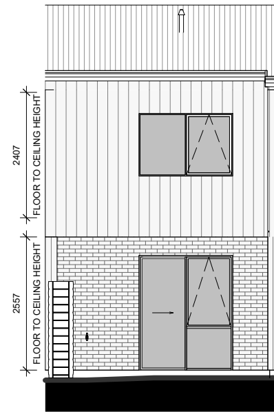
LOT 111 - NORTH ELEVATION
