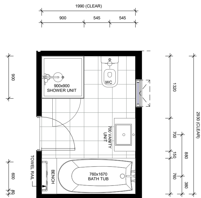
LOT 112 - FIRST FLOOR BATHROOM LAYOUT
