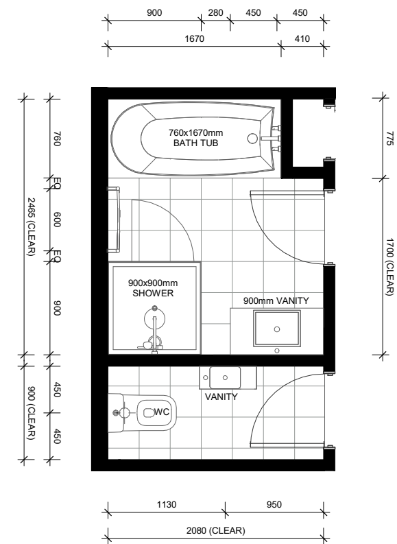
LOT 111 - FIRST FLOOR BATHROOM & WC LAYOUT
