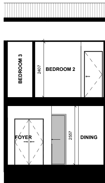
LOT 111 - SECTION A - A
