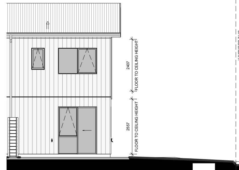
LOT 110 - NORTH ELEVATION
