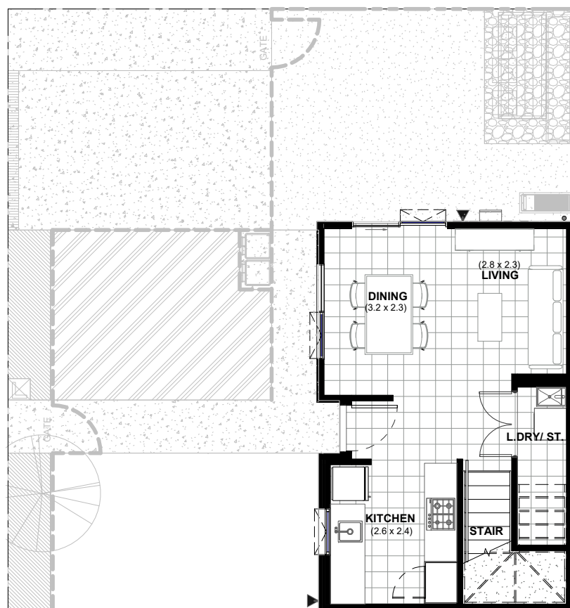
LOT 110 - GROUND FLOOR PLAN
