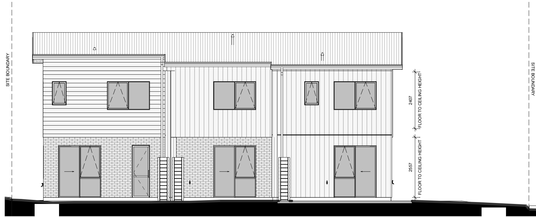
OVERALL - NORTH ELEVATION
