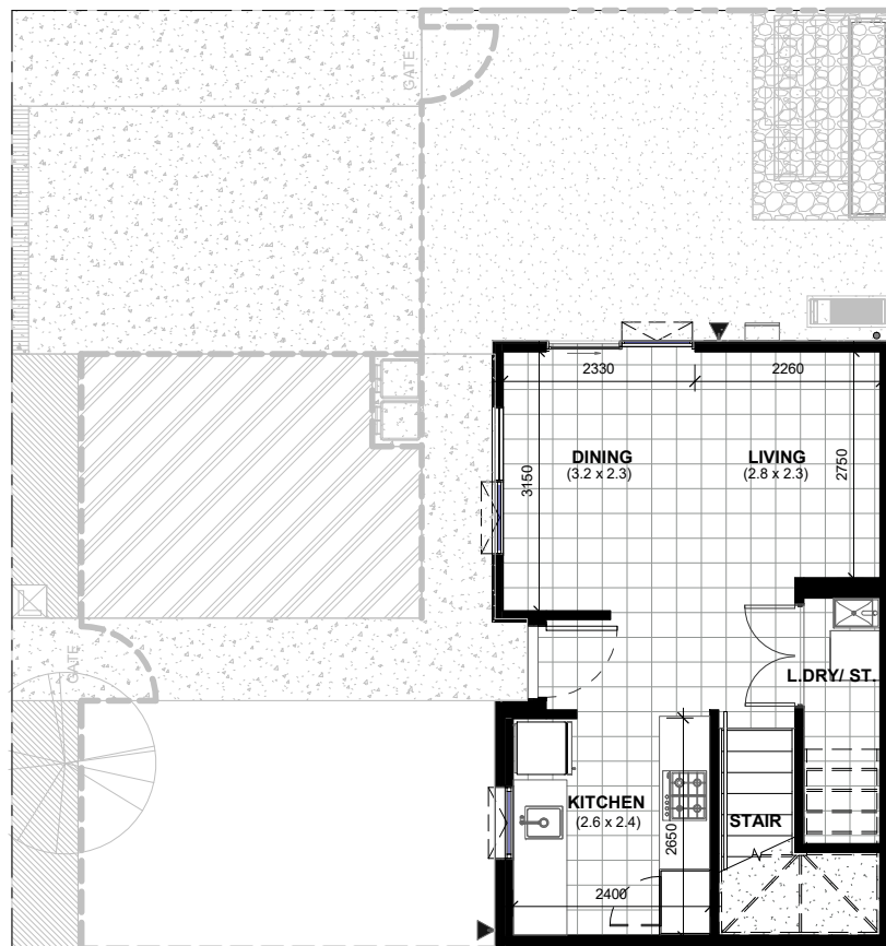
LOT 110- GROUND FLOOR DIMENSION PLAN
