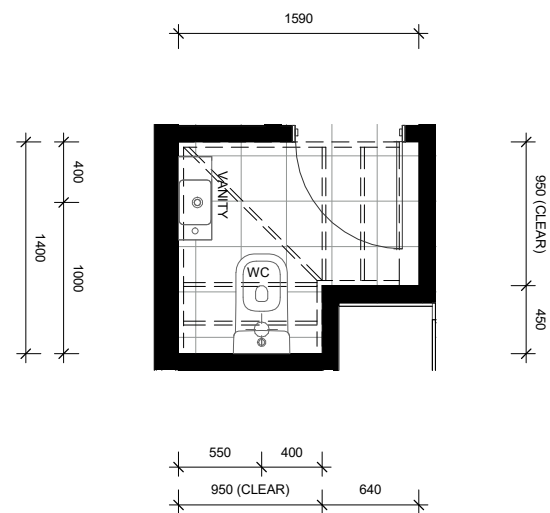
LOT 112 - GROUND FLOOR WC LAYOUT
