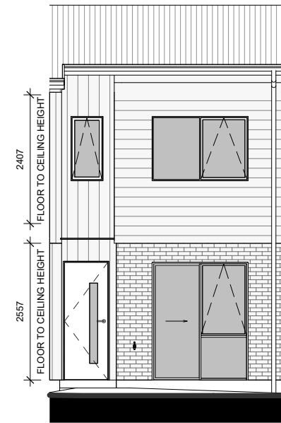
LOT 111 - SOUTH ELEVATION
