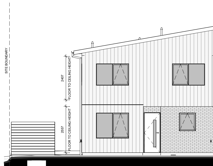
LOT 110 - WEST ELEVATION
