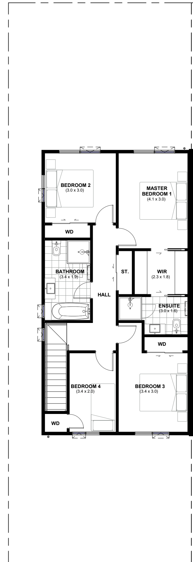
LOT 145 - FIRST FLOOR PLAN
