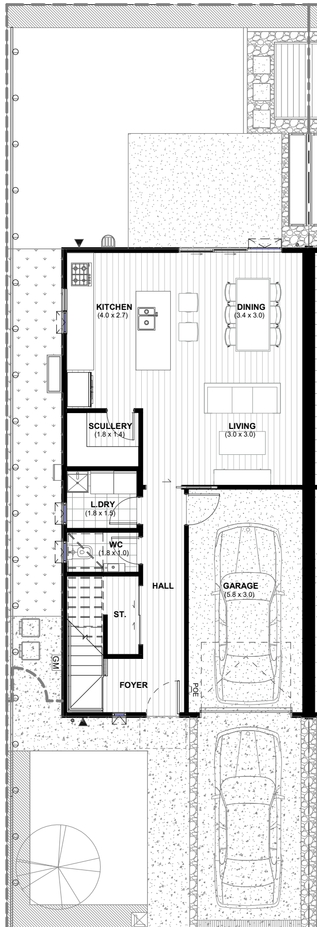
LOT 145 - GROUND FLOOR PLAN
