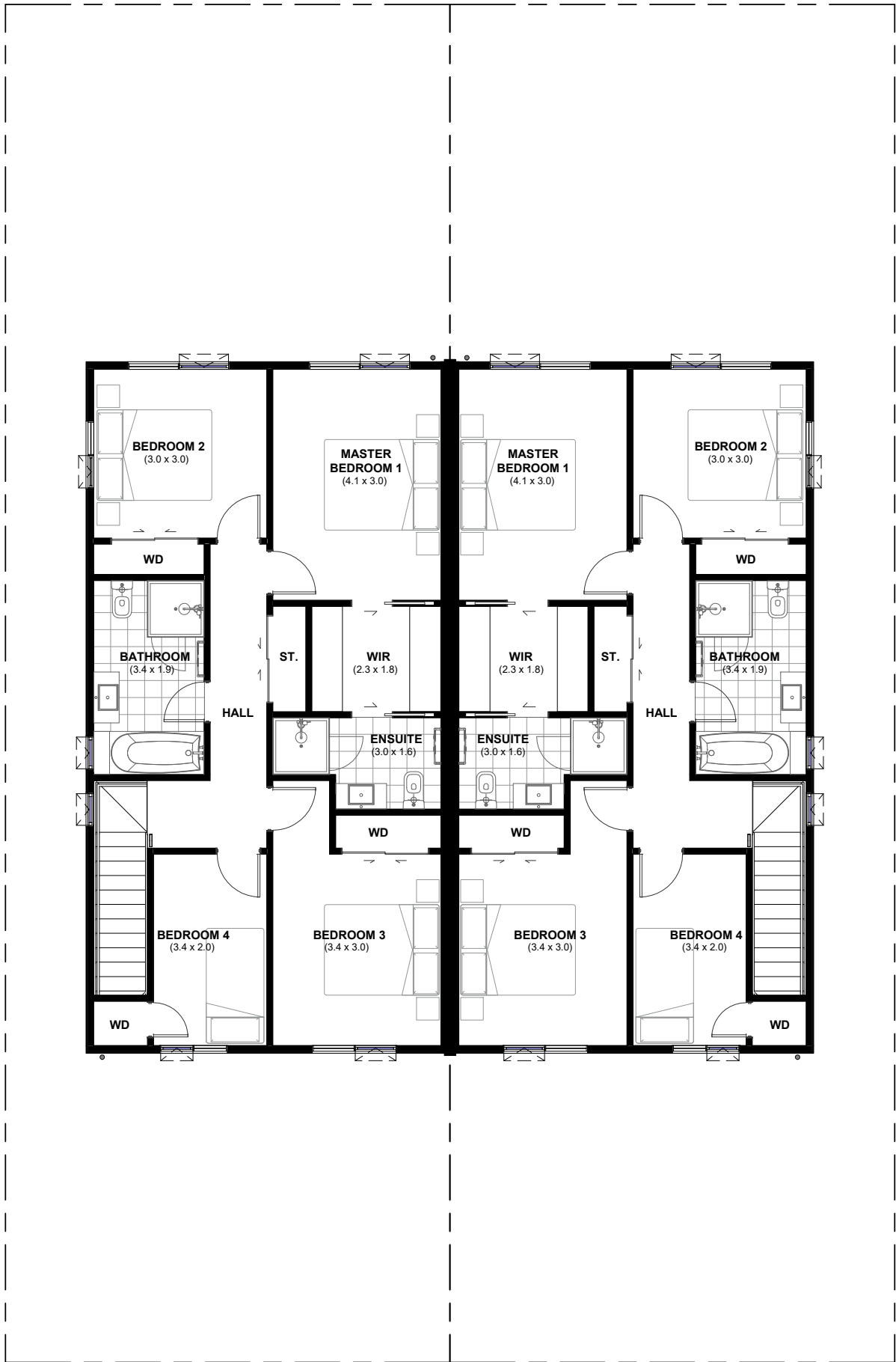
LOT 145 FIRST FLOOR PLAN
