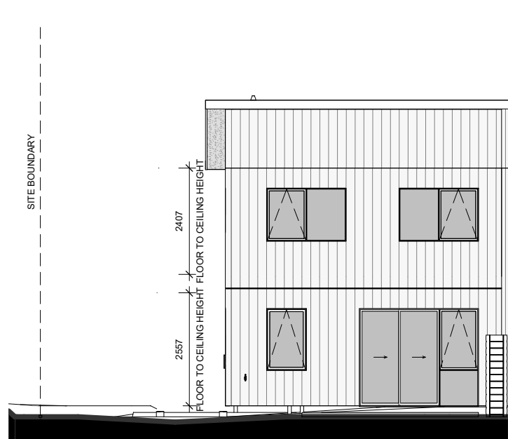
LOT 81 - NORTH ELEVATION
