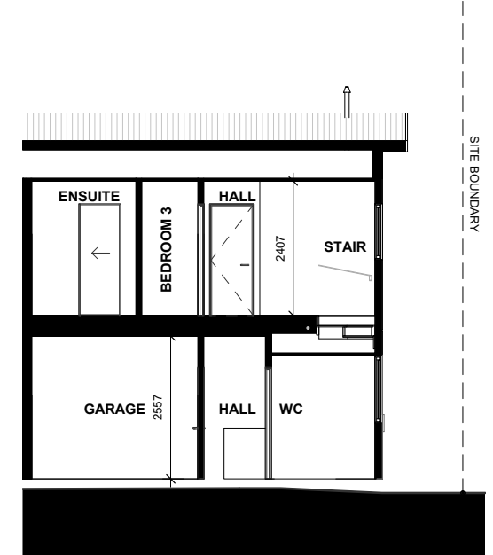
LOT 81- SECTION A-A
