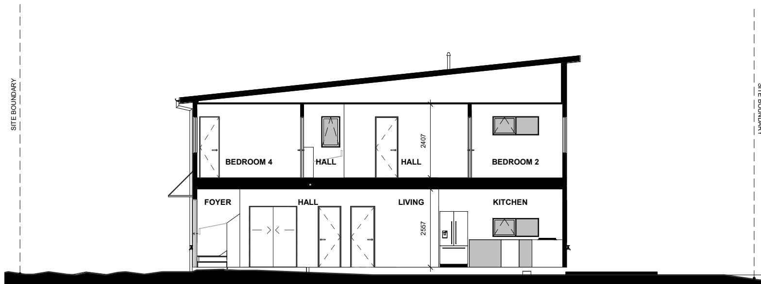
LOT 82 - SECTION C-C
