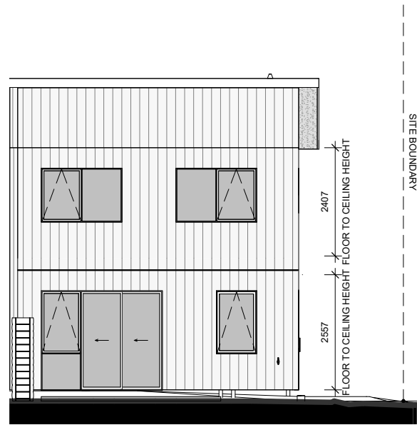
LOT 82 - NORTH ELEVATION
