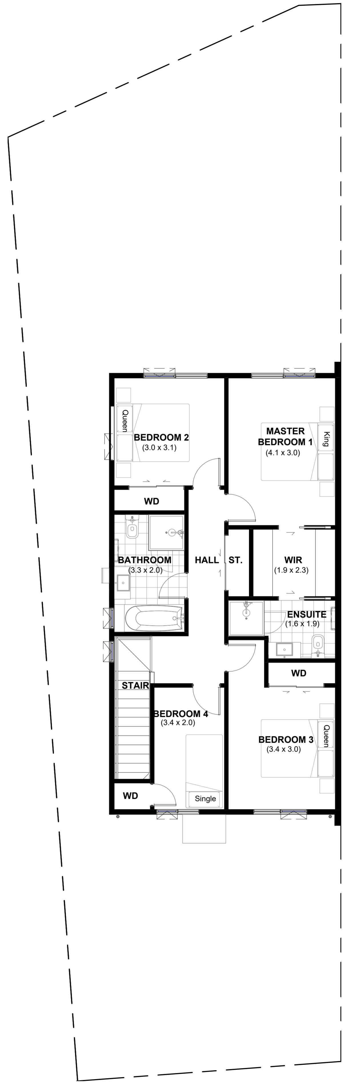
LOT 82 - FIRST FLOOR PLAN
