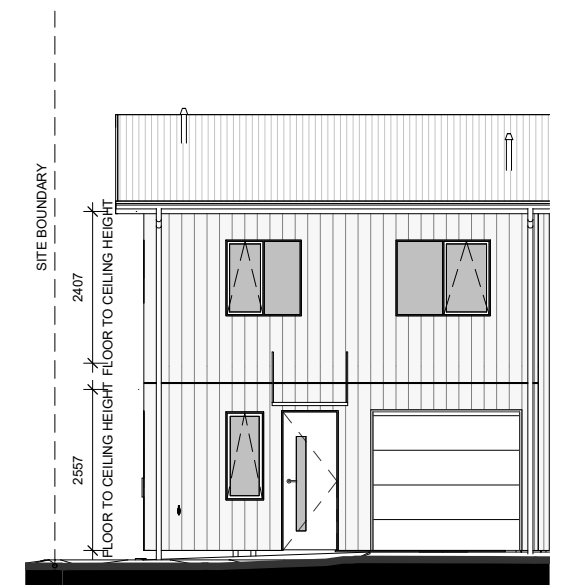
LOT 82 - SOUTH ELEVATION
