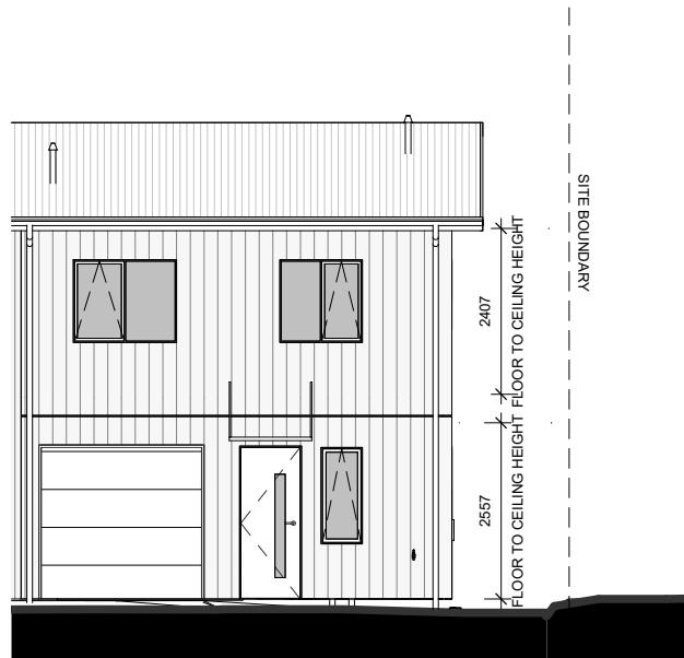
LOT 81 - SOUTH ELEVATION
