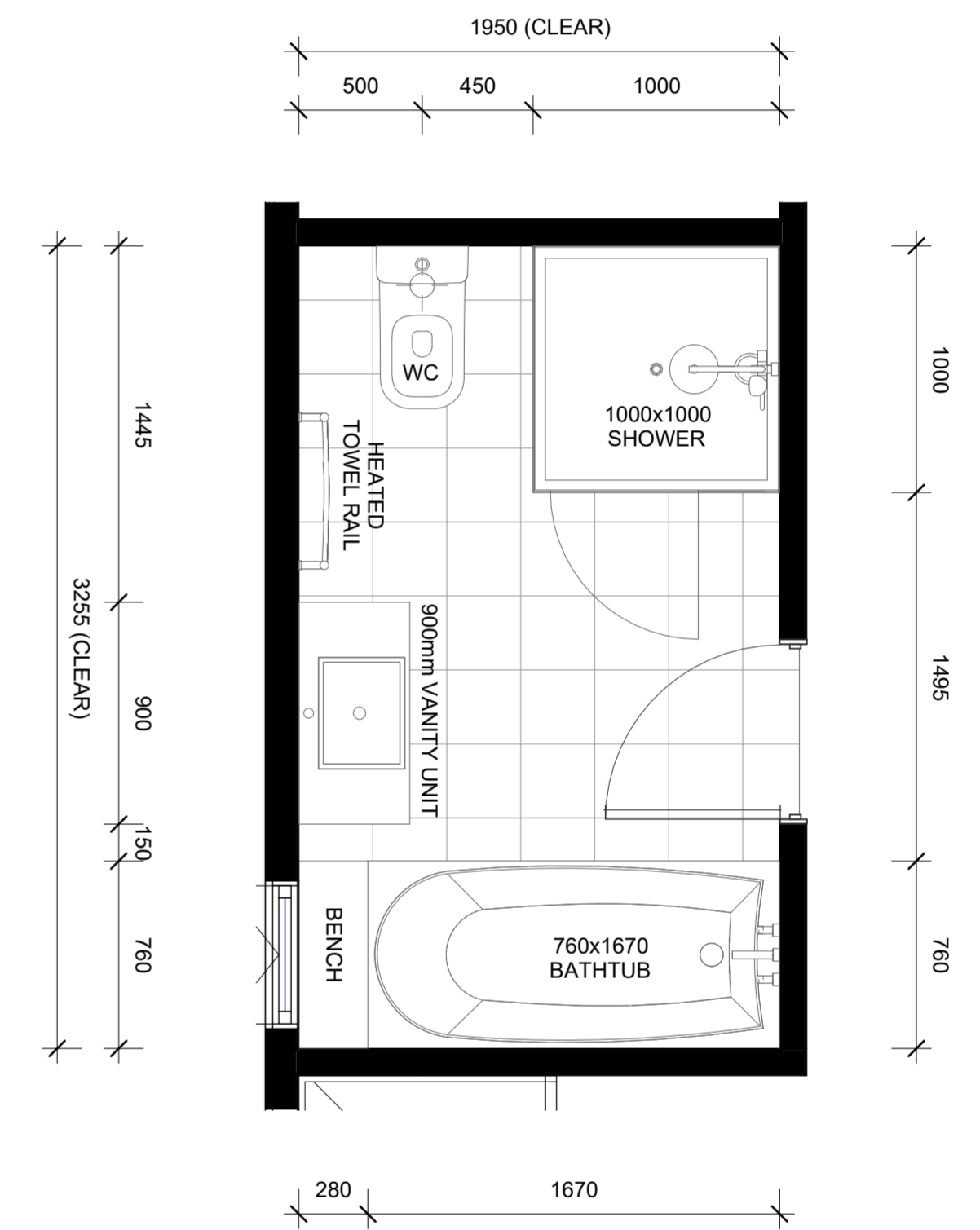
LOT 82 - FIRST FLOOR BATHROOM LAYOUT
