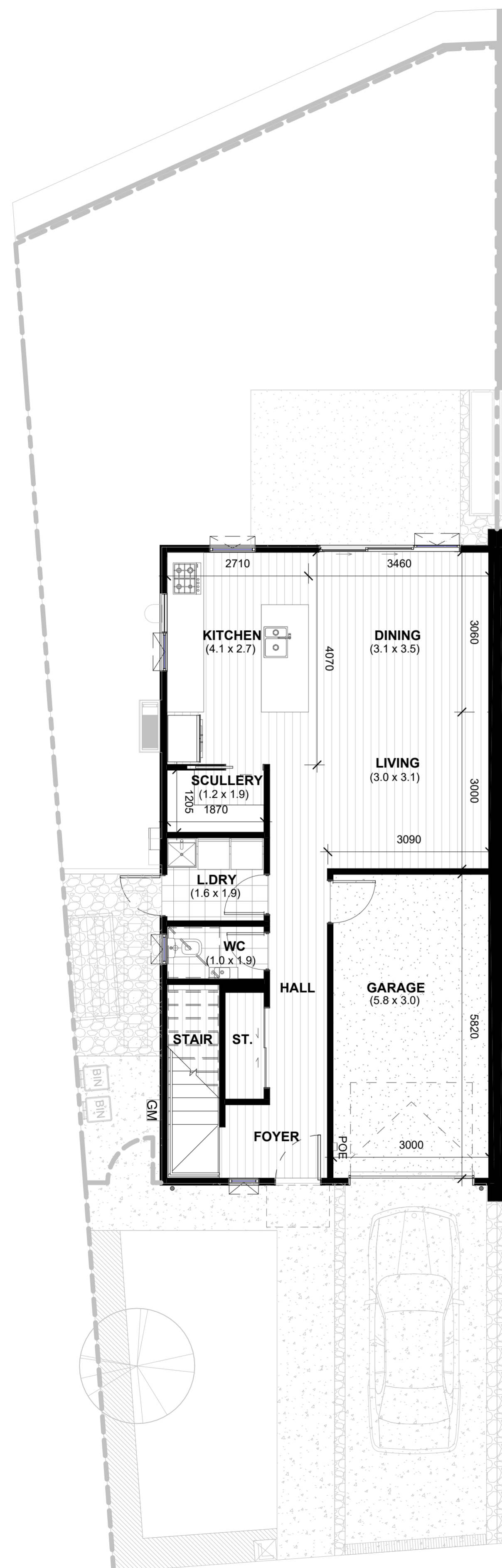
LOT 82 - GROUND FLOOR DIMENSION PLAN
