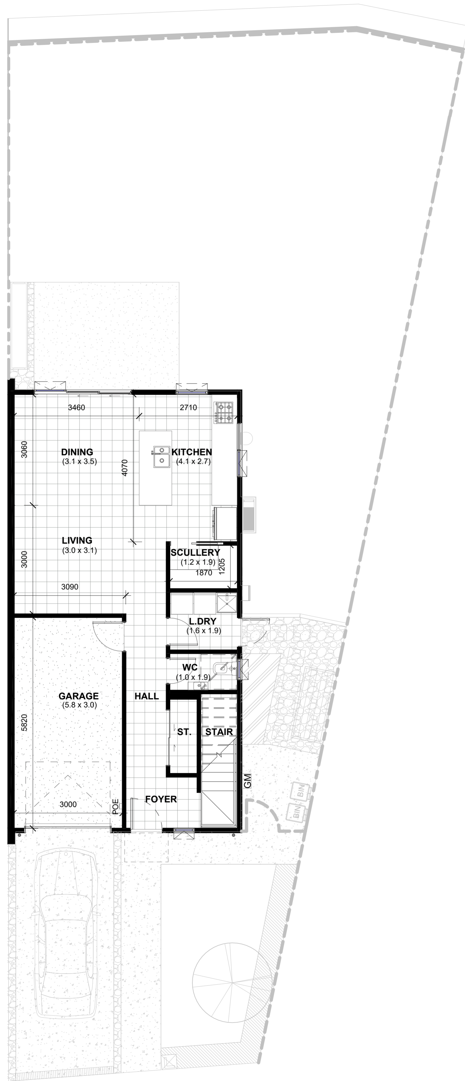
LOT 81 - GROUND FLOOR DIMENSION PLAN
