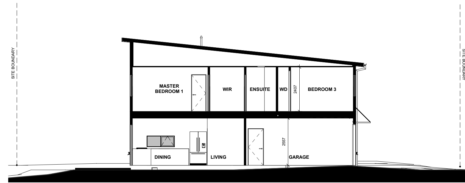
LOT 81 - SECTION D-D
