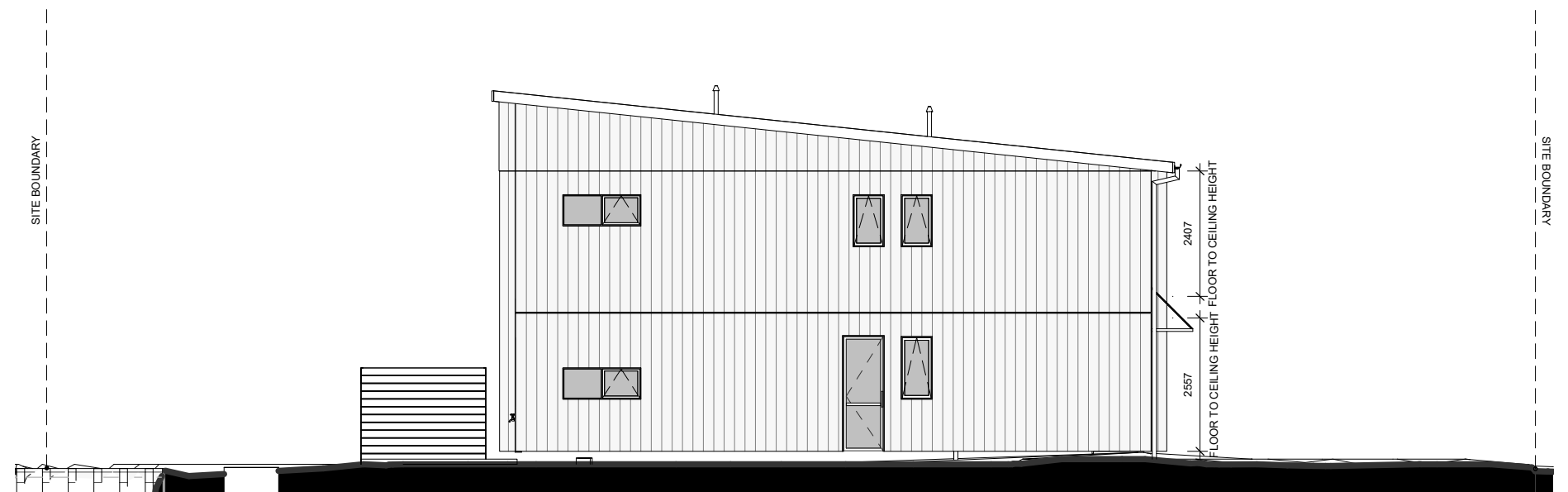
LOT 82 - WEST ELEVATION
