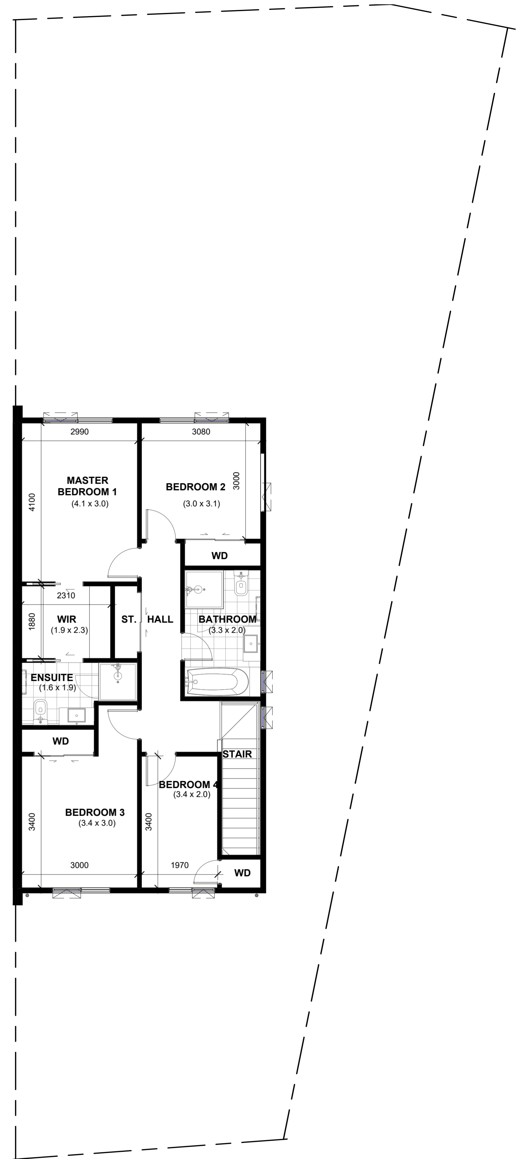
LOT 81 - FIRST FLOOR DIMENSION PLAN
