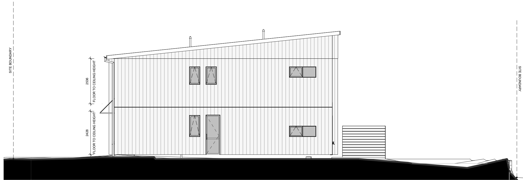
OVERALL EAST ELEVATION
