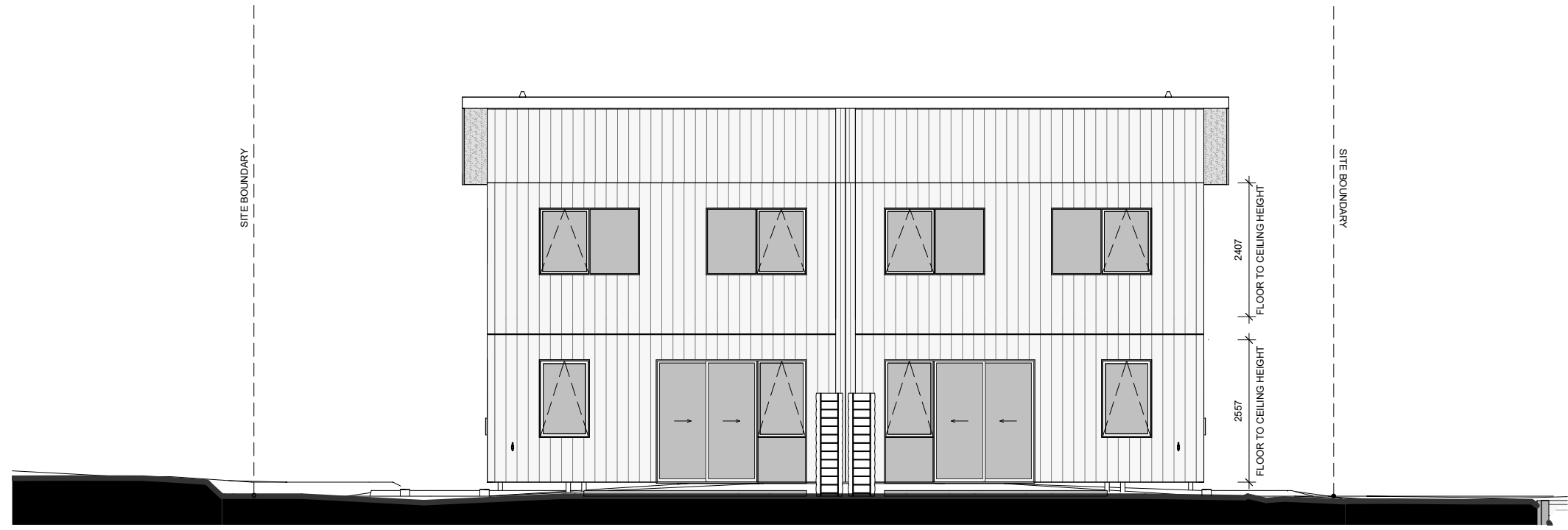
OVERALL NORTH ELEVATION
