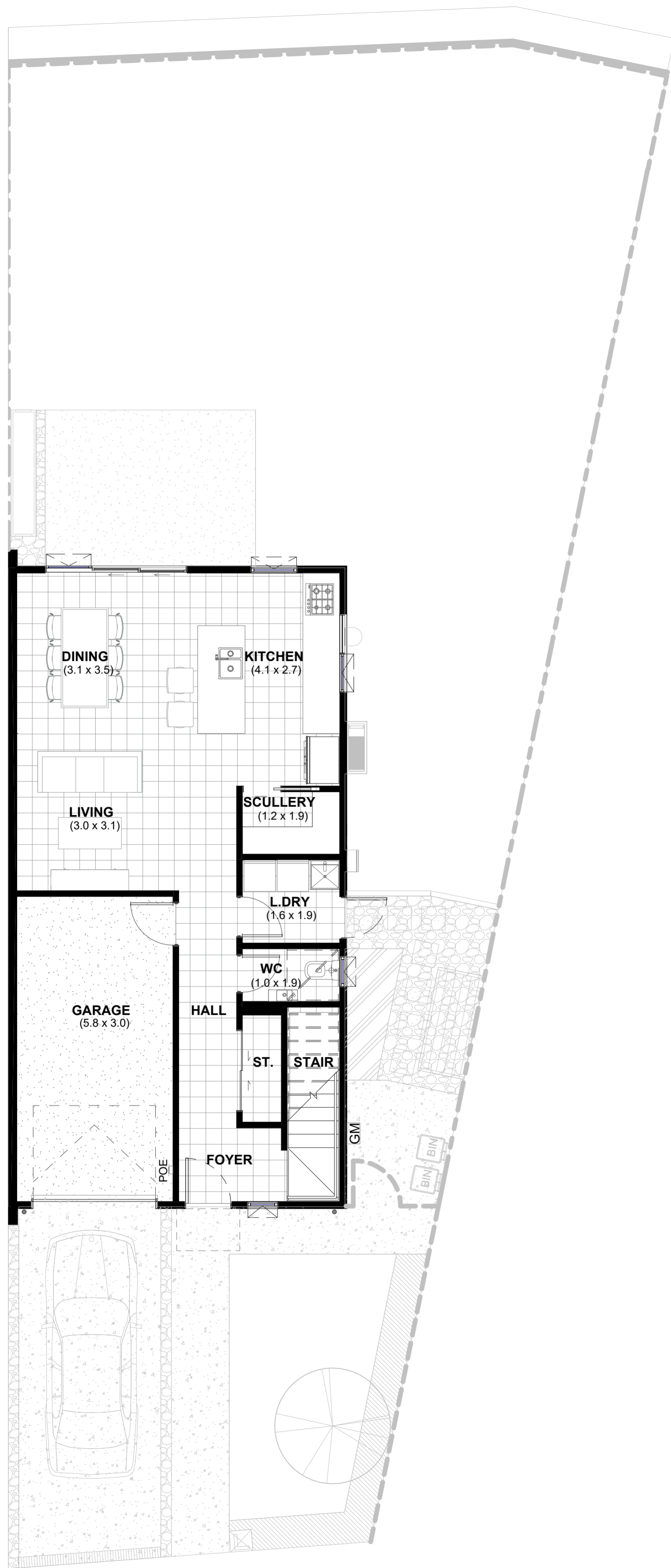
LOT 81 - GROUND FLOOR PLAN
