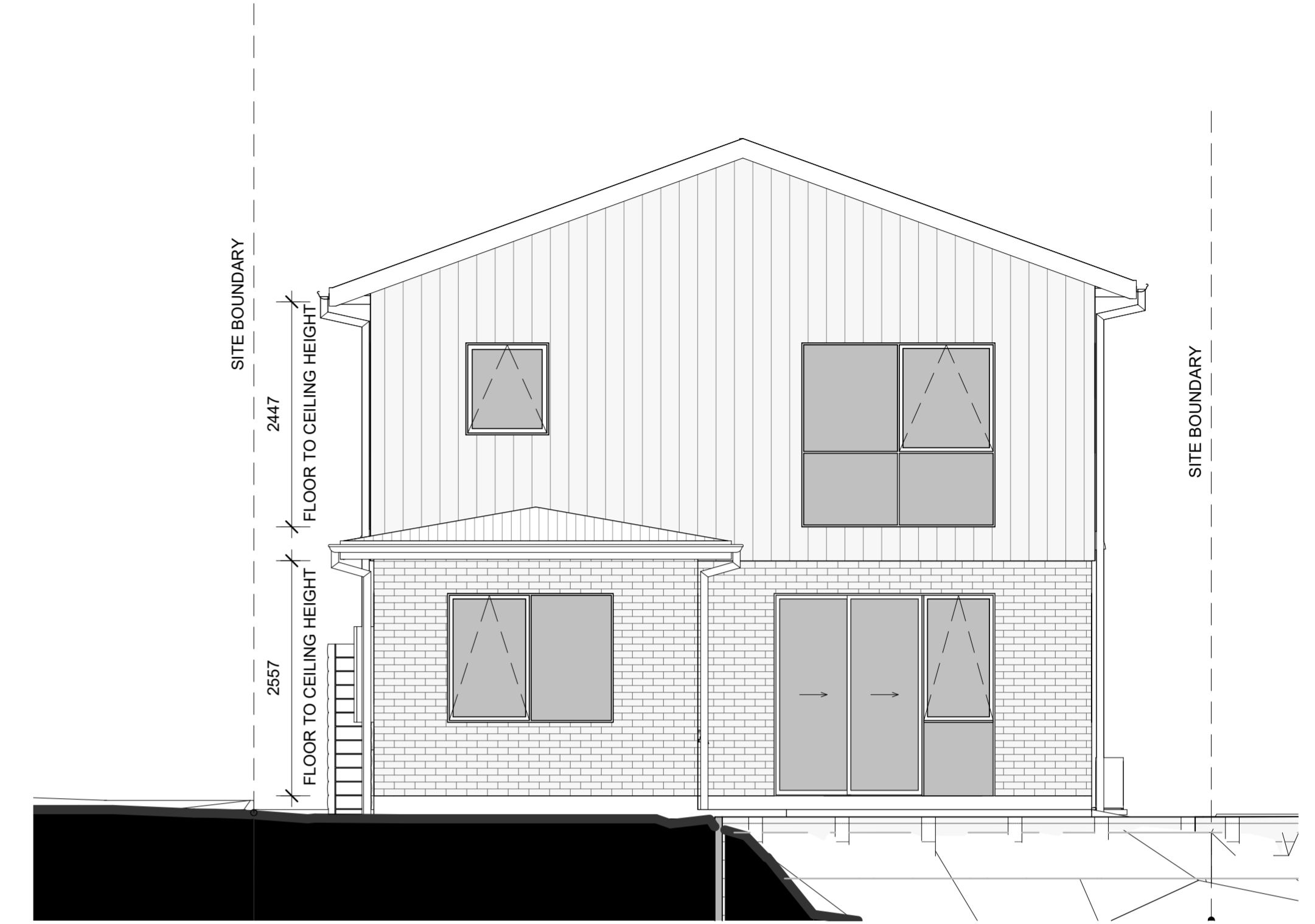
LOT 83 - NORTH ELEVATION
