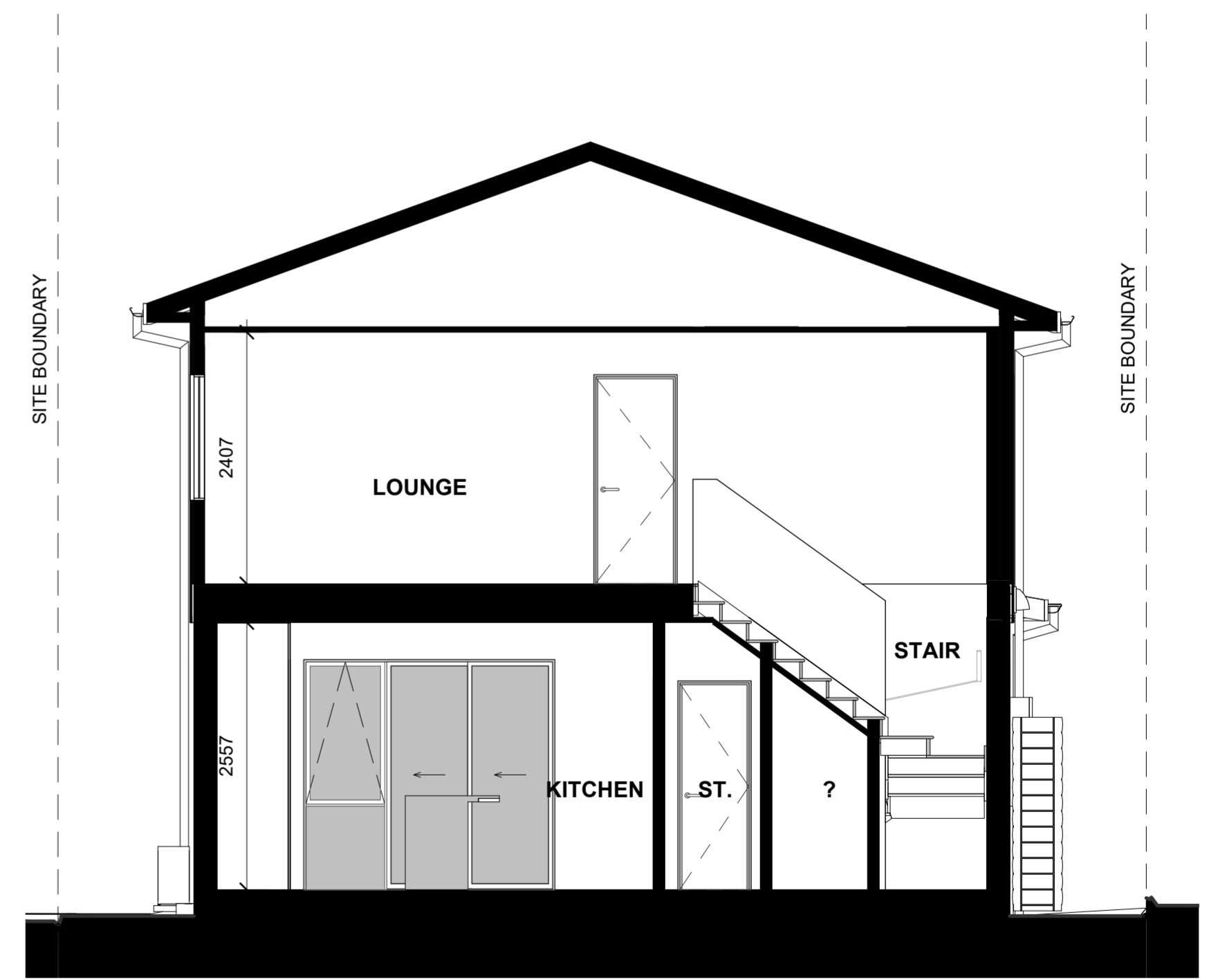
LOT 83 - SECTION D-D
