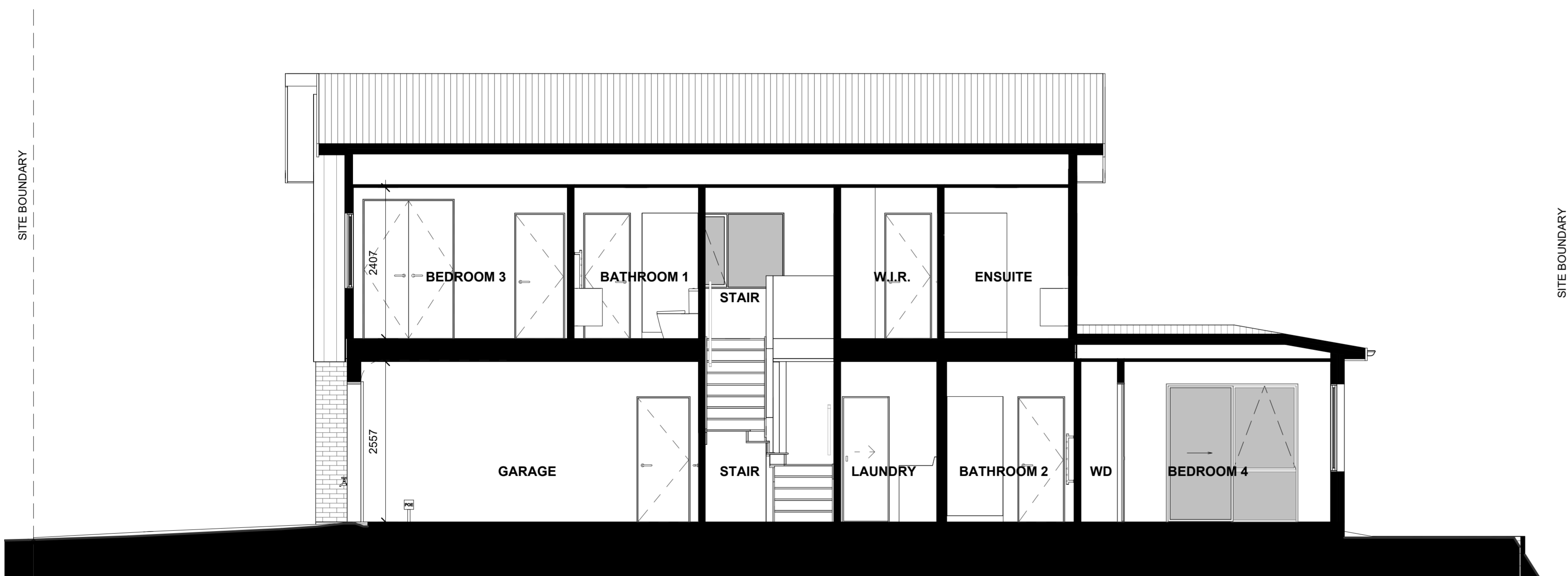
LOT 83 - SECTION B-B
