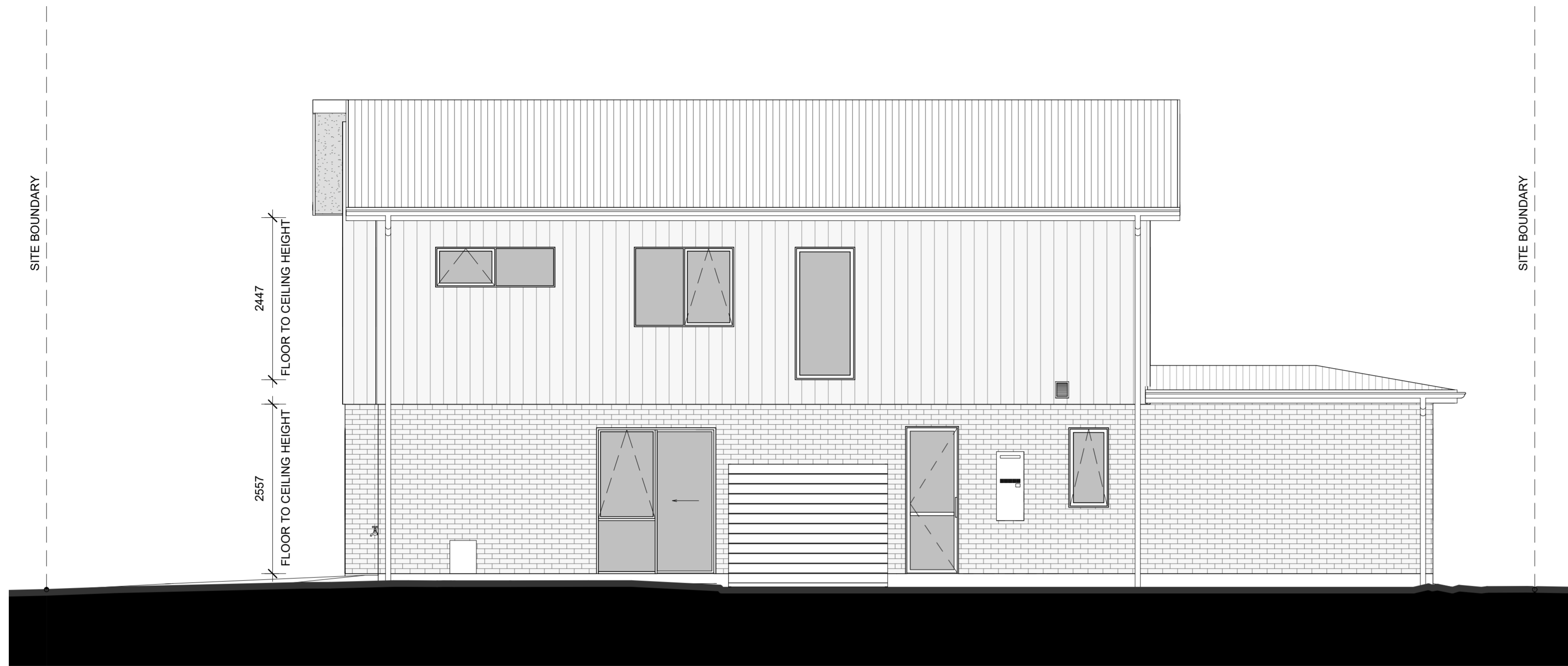
LOT 83 - EAST ELEVATION
