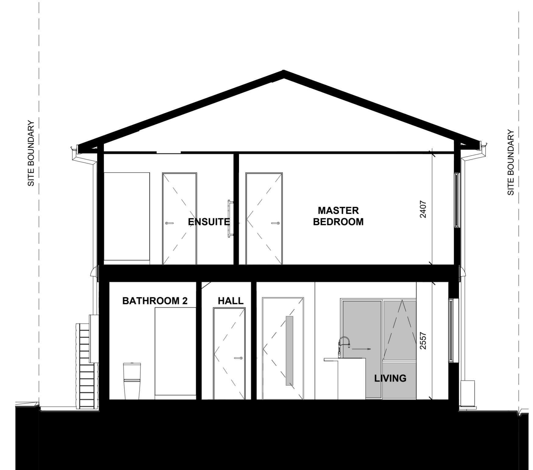
LOT 83 - SECTION C-C
