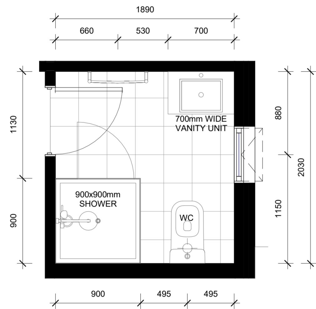
LOT 83 - GROUND FLOOR BATHROOM LAYOUT PLAN
