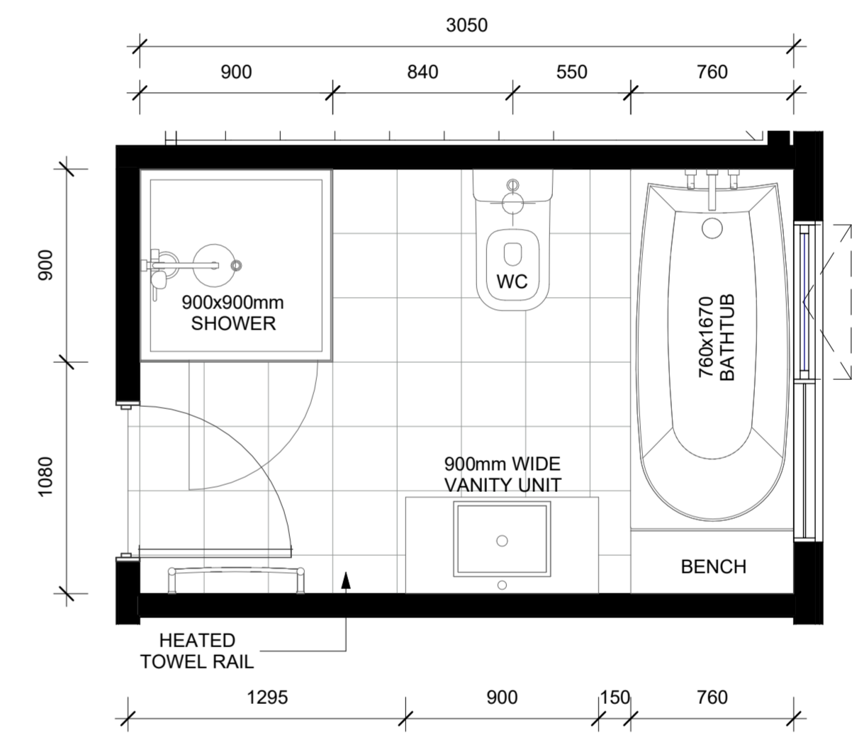
LOT 83 - FIRST FLOOR BATHROOM LAYOUT PLAN
