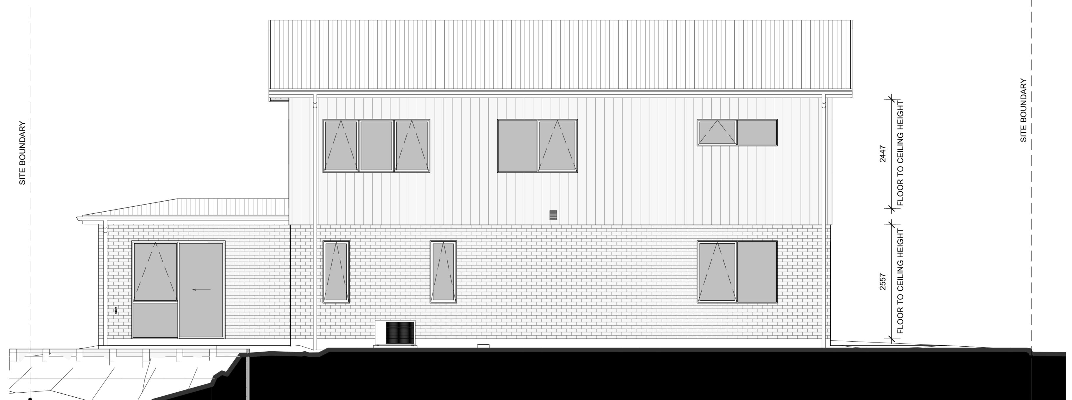
LOT 83 - WEST ELEVATION
