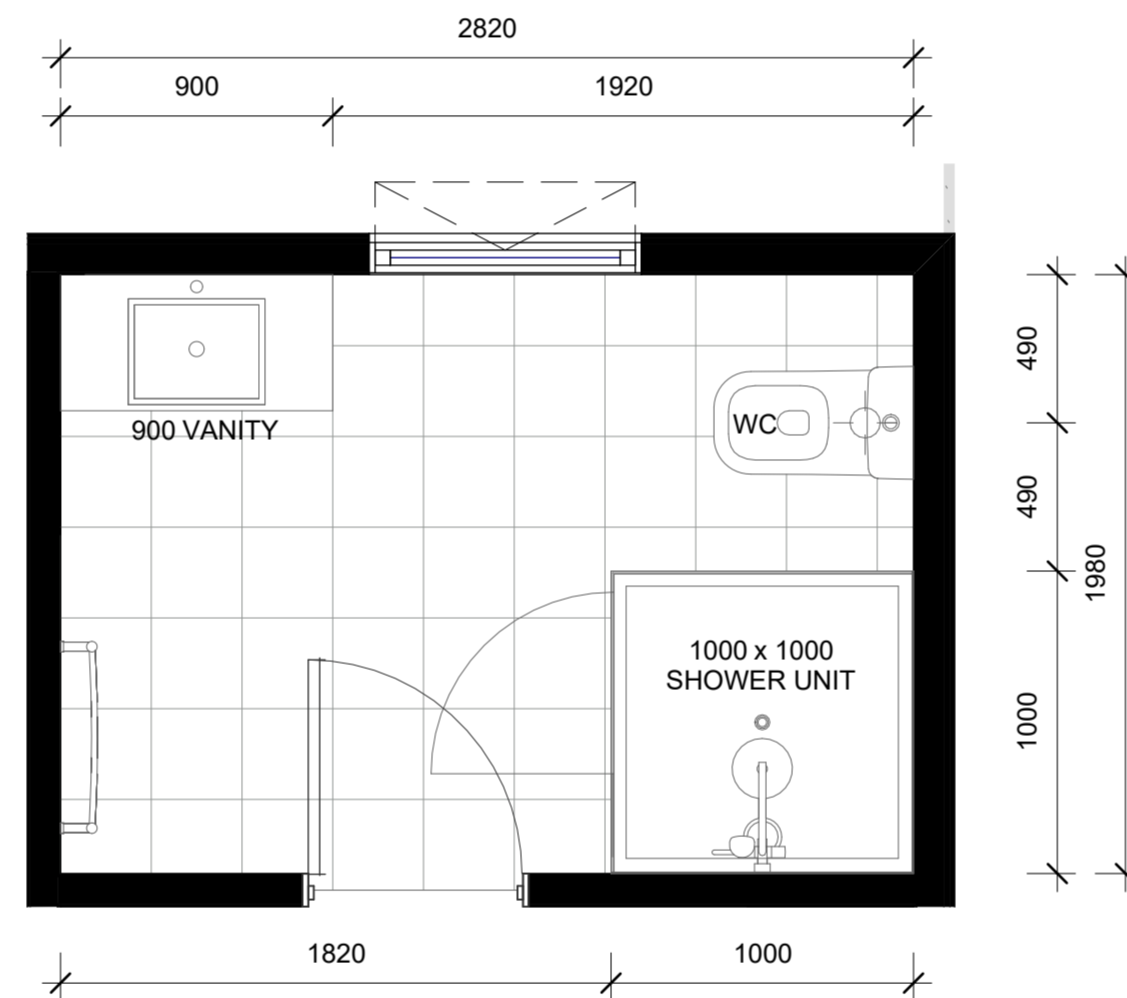
LOT 83 - FIRST FLOOR ENSUITE LAYOUT
