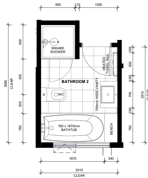
LOT 2 - FIRST FLOOR BATHROOM LAYOUT
