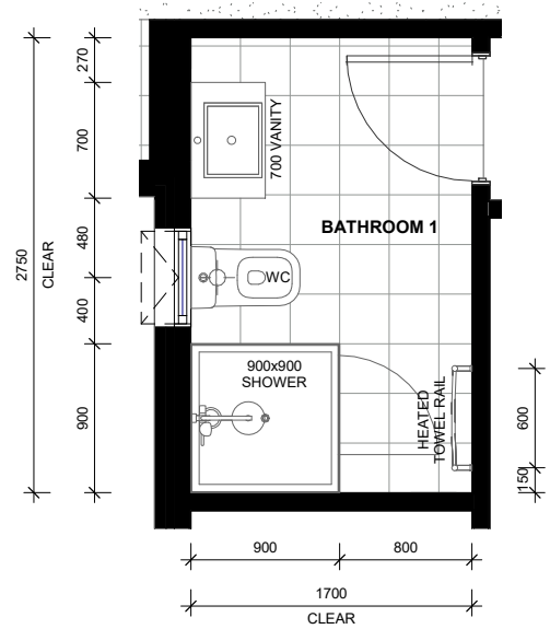
LOT 2 - GROUND FLOOR BATHROOM LAYOUT
