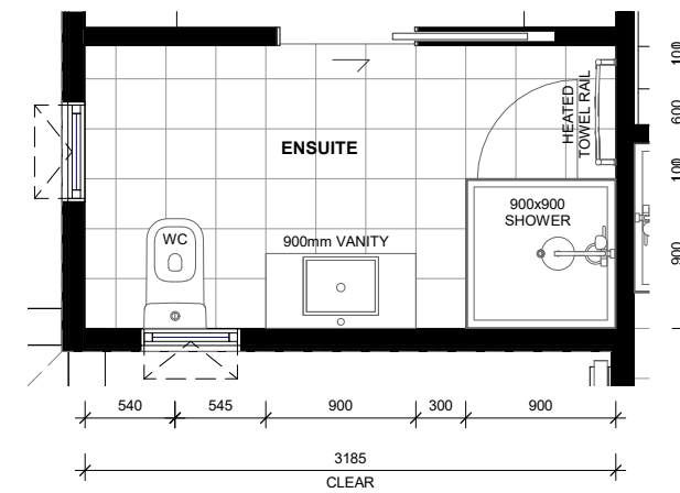
LOT 2 - FIRST FLOOR ENSUITE LAYOUT
