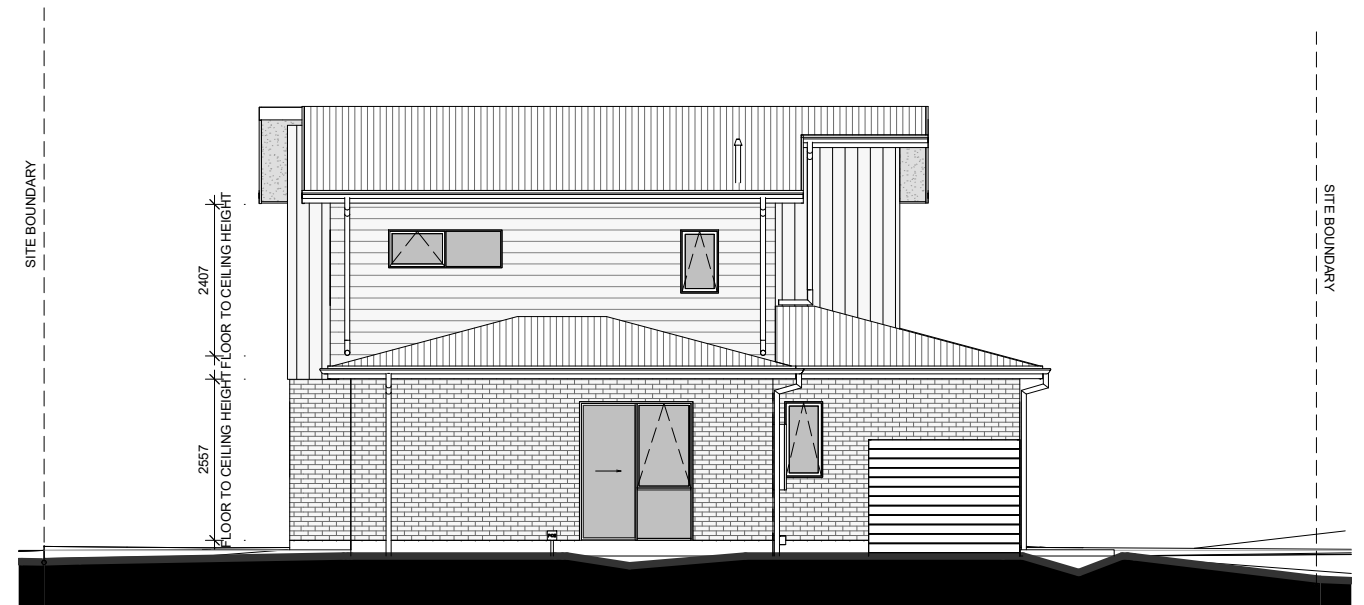
LOT 2 - SOUTH ELEVATION
