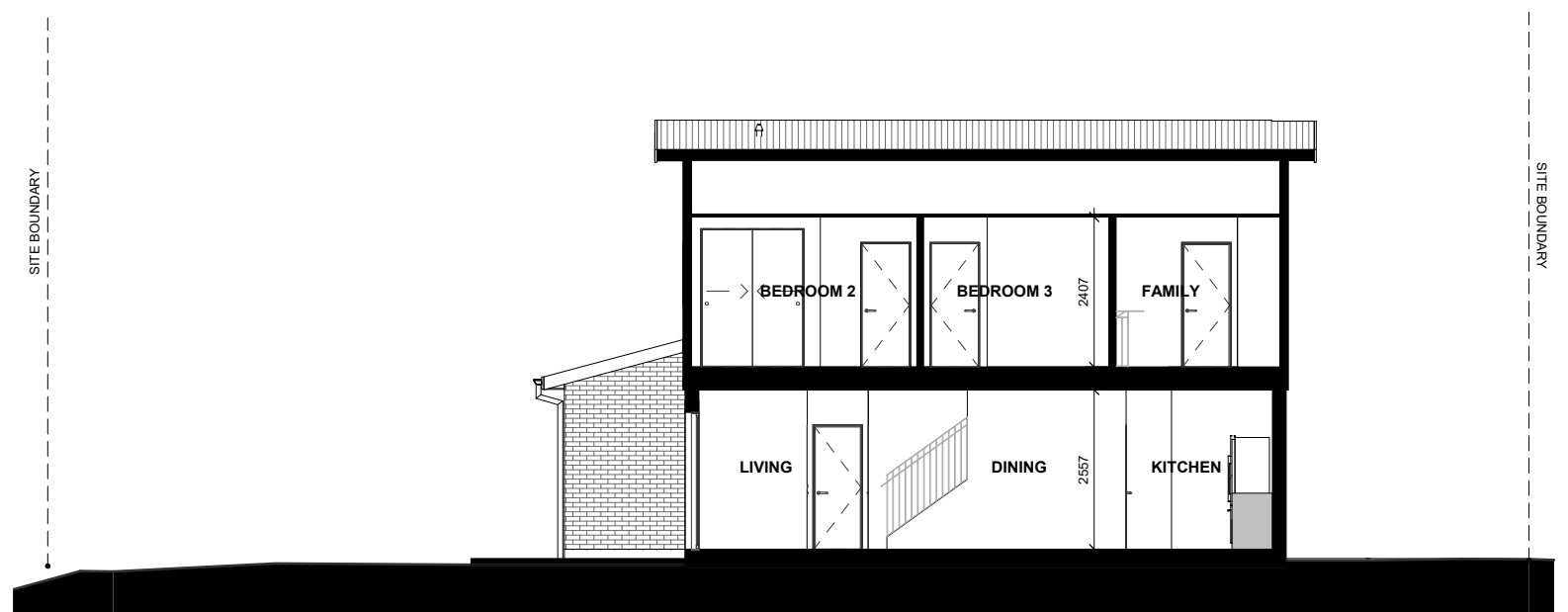
LOT 2 - SECTION C-C
