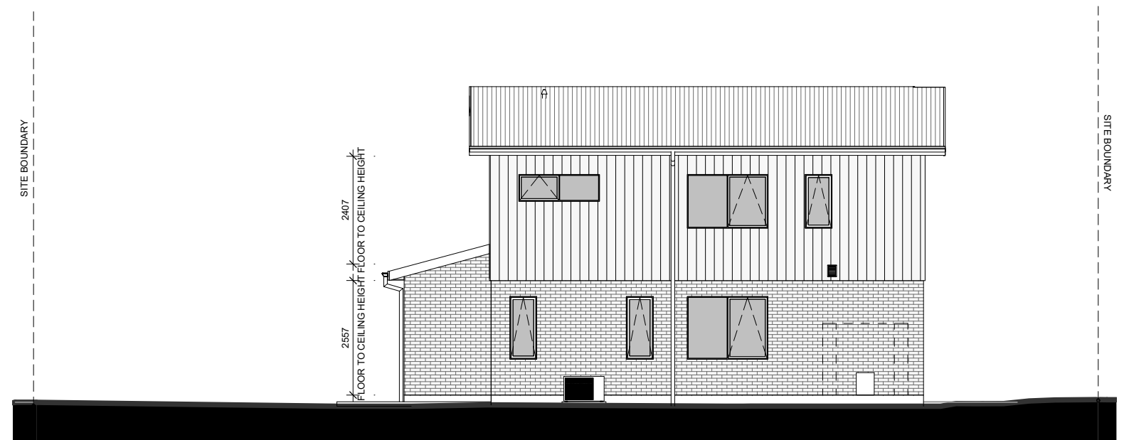
LOT 2 - NORTH ELEVATION
