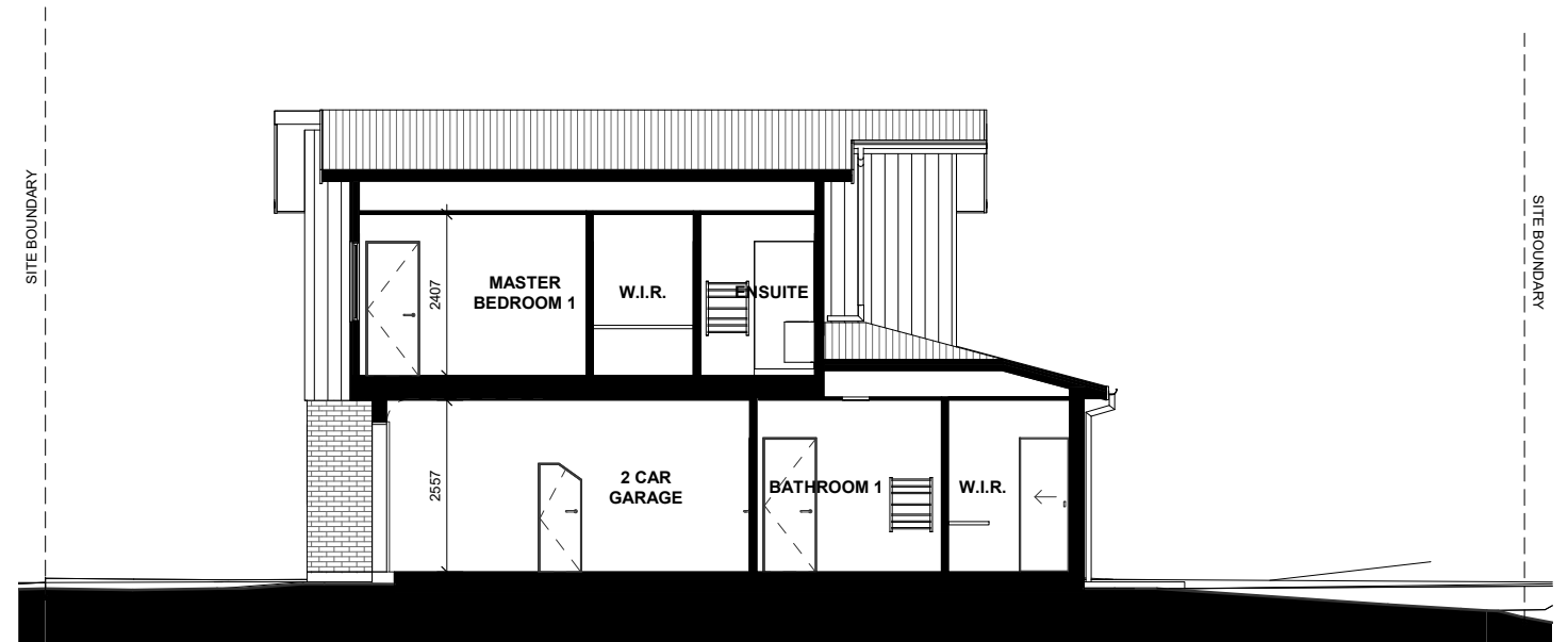
LOT 2 - SECTION D-D
