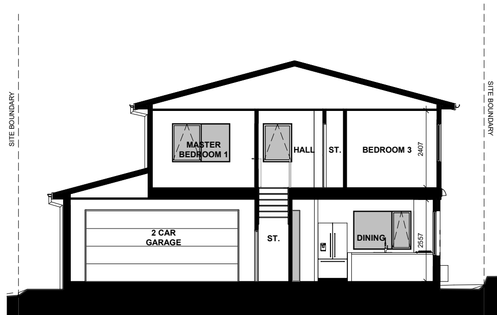
LOT 2 - SECTION A-A
