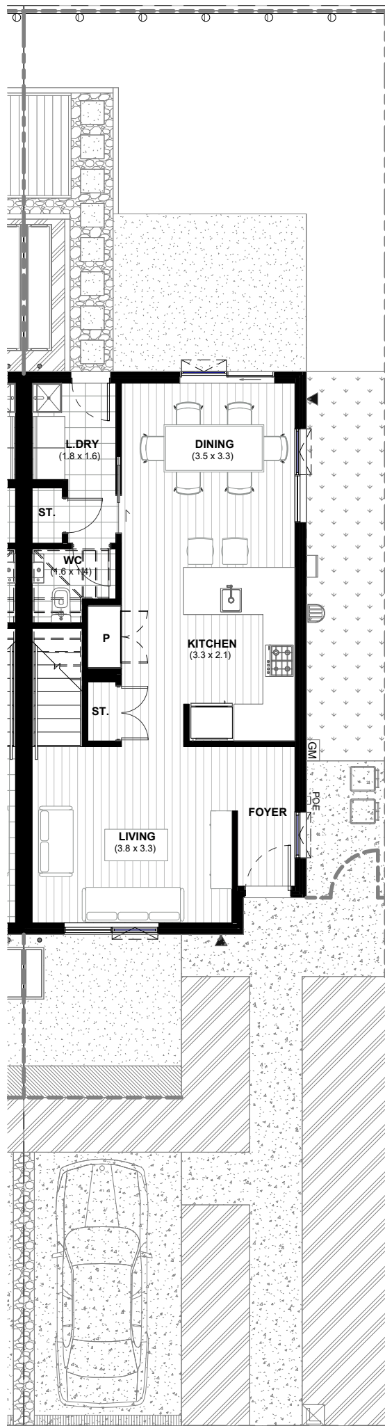
LOT 103 - GROUND FLOOR PLAN
