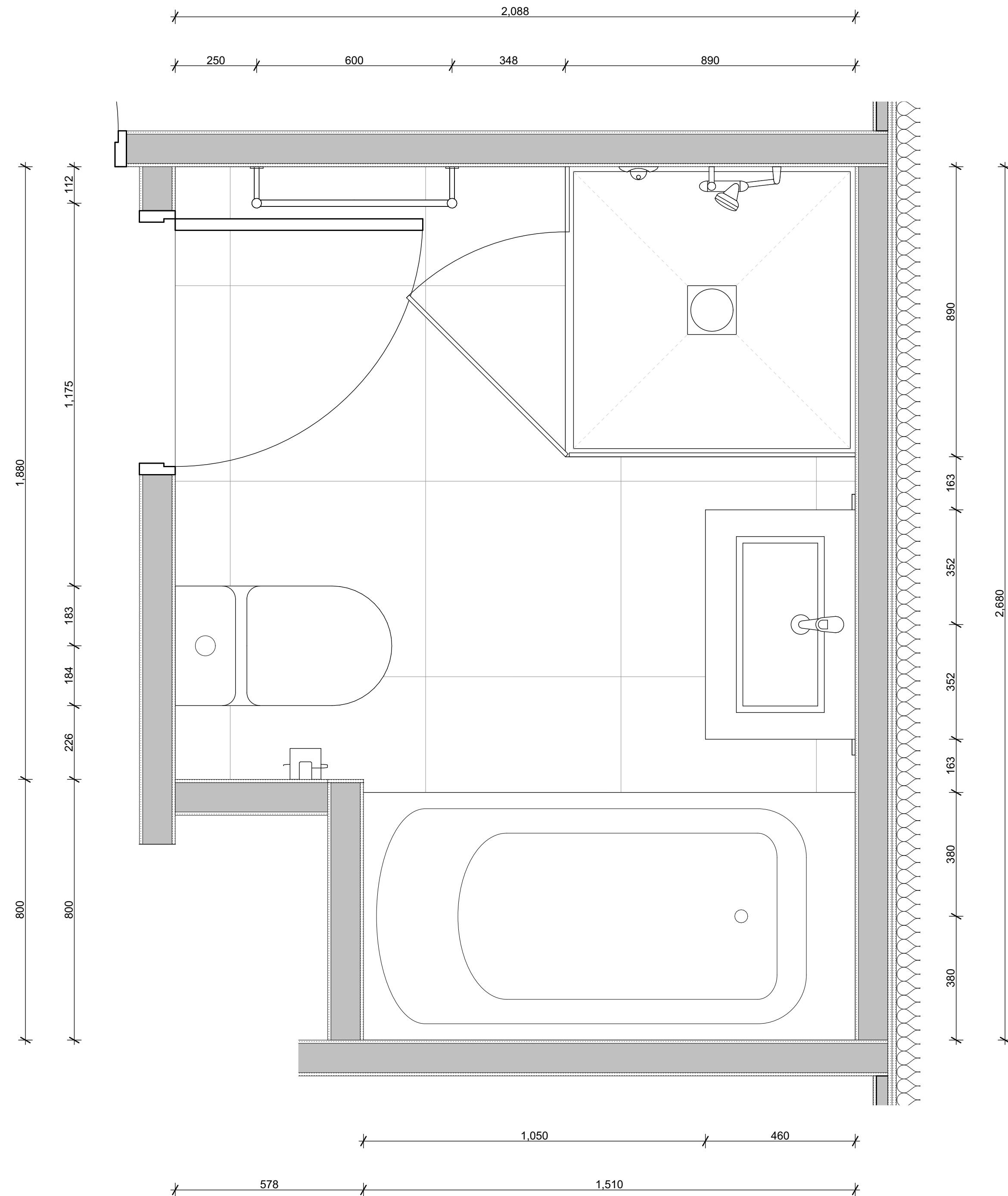
1 | FIRST FLOOR BATHROOM - | 1:10
