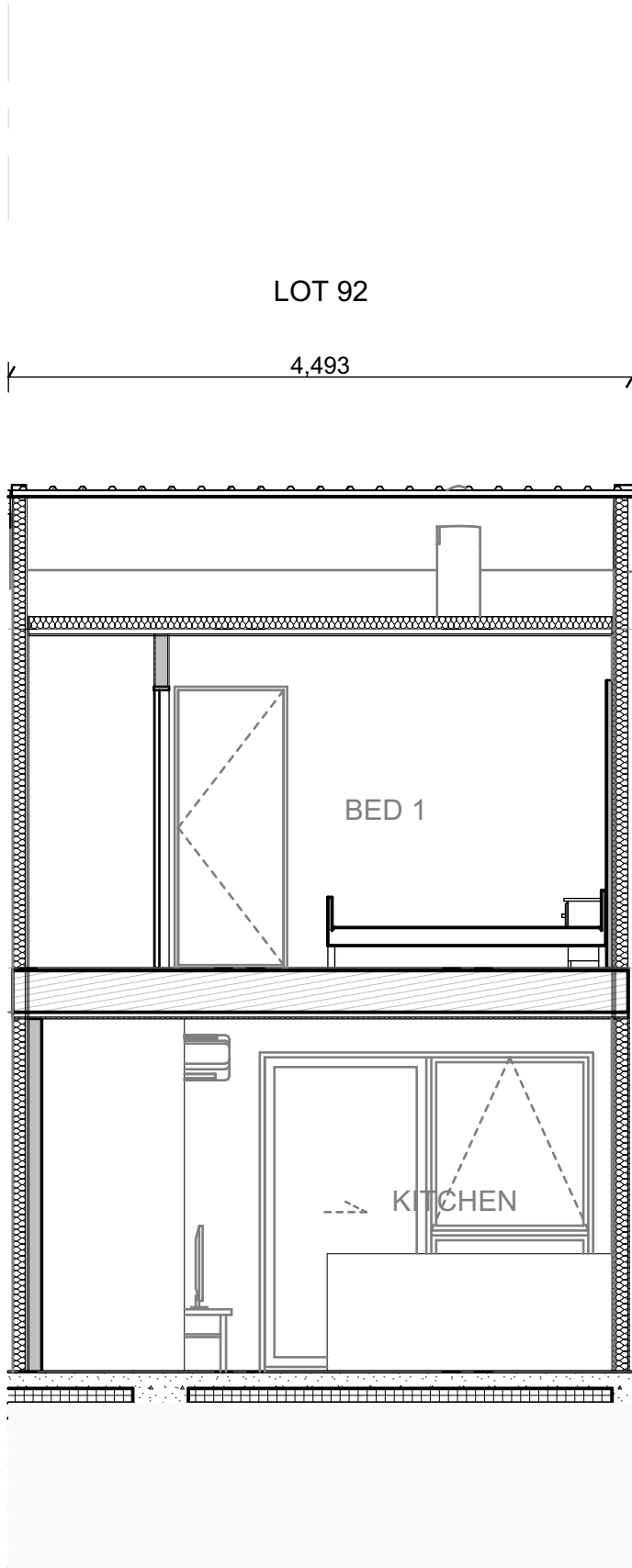
1 | LOT 92 SECTION - | 1:50
