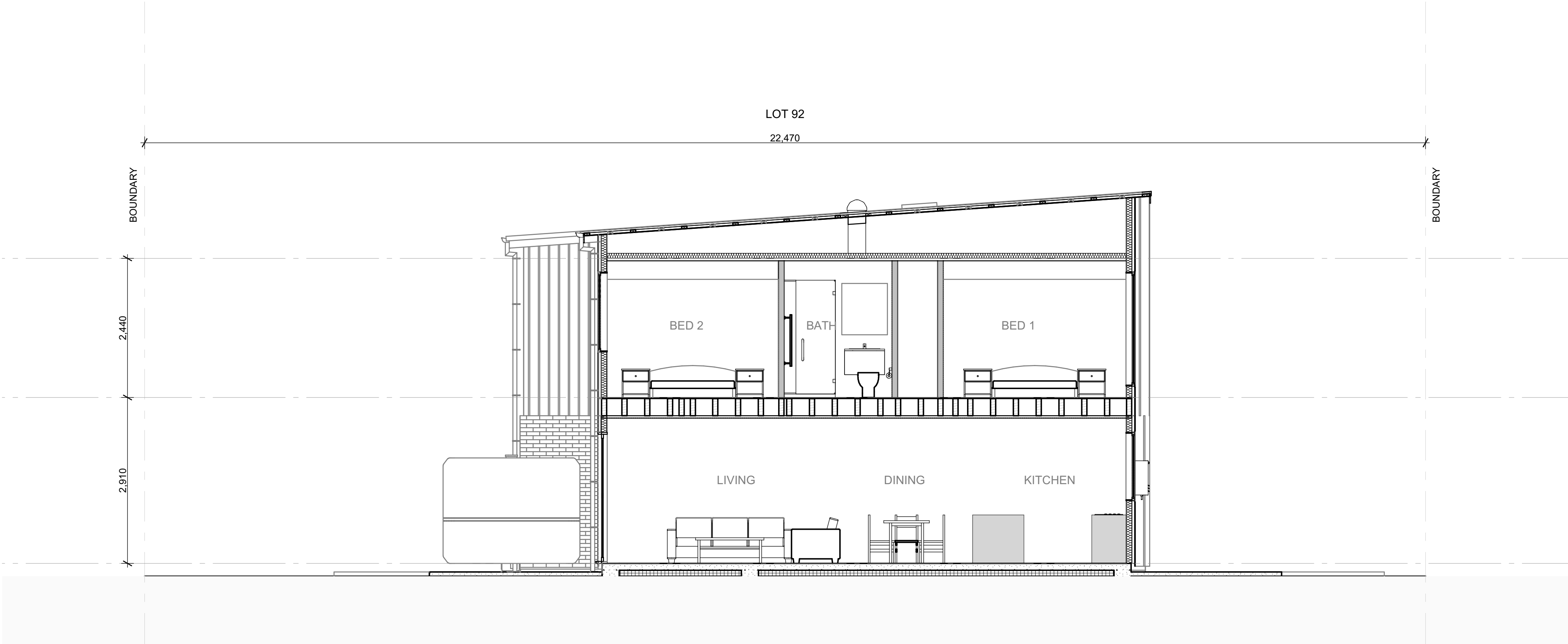
2 | LOT 92 CROSS SECTION - | 1:50
