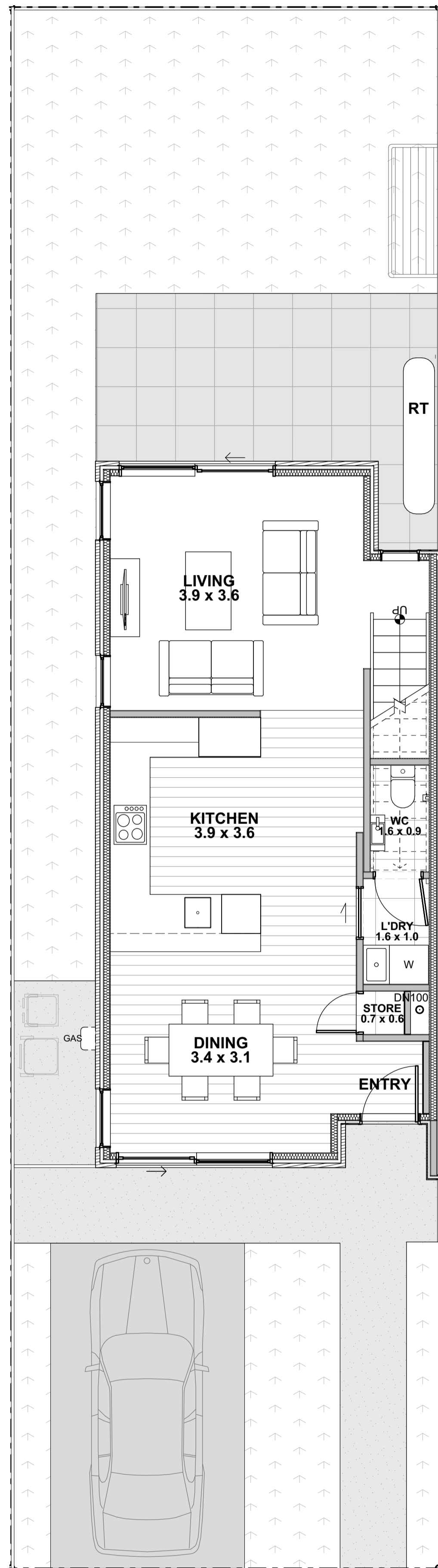
1 | GROUND FLOOR PLAN - | 1:50
