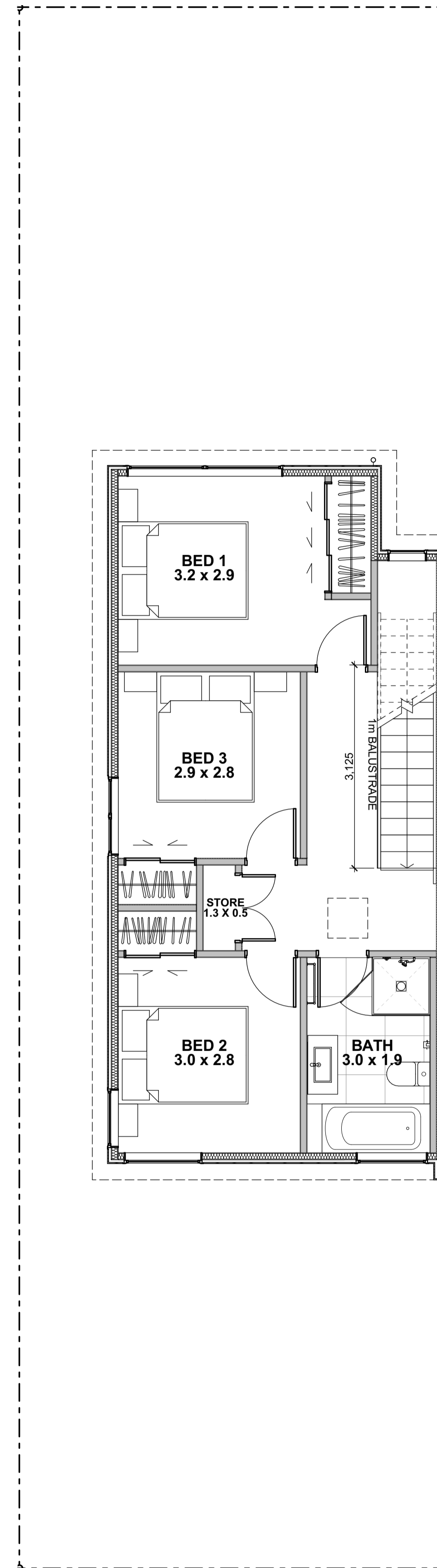
2 | FIRST FLOOR PLAN - | 1:50
