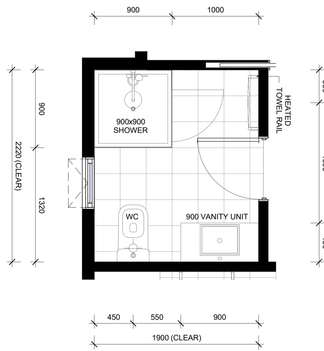
LOT 75 - FIRST FLOOR PLAN ENSUITE LAYOUT
