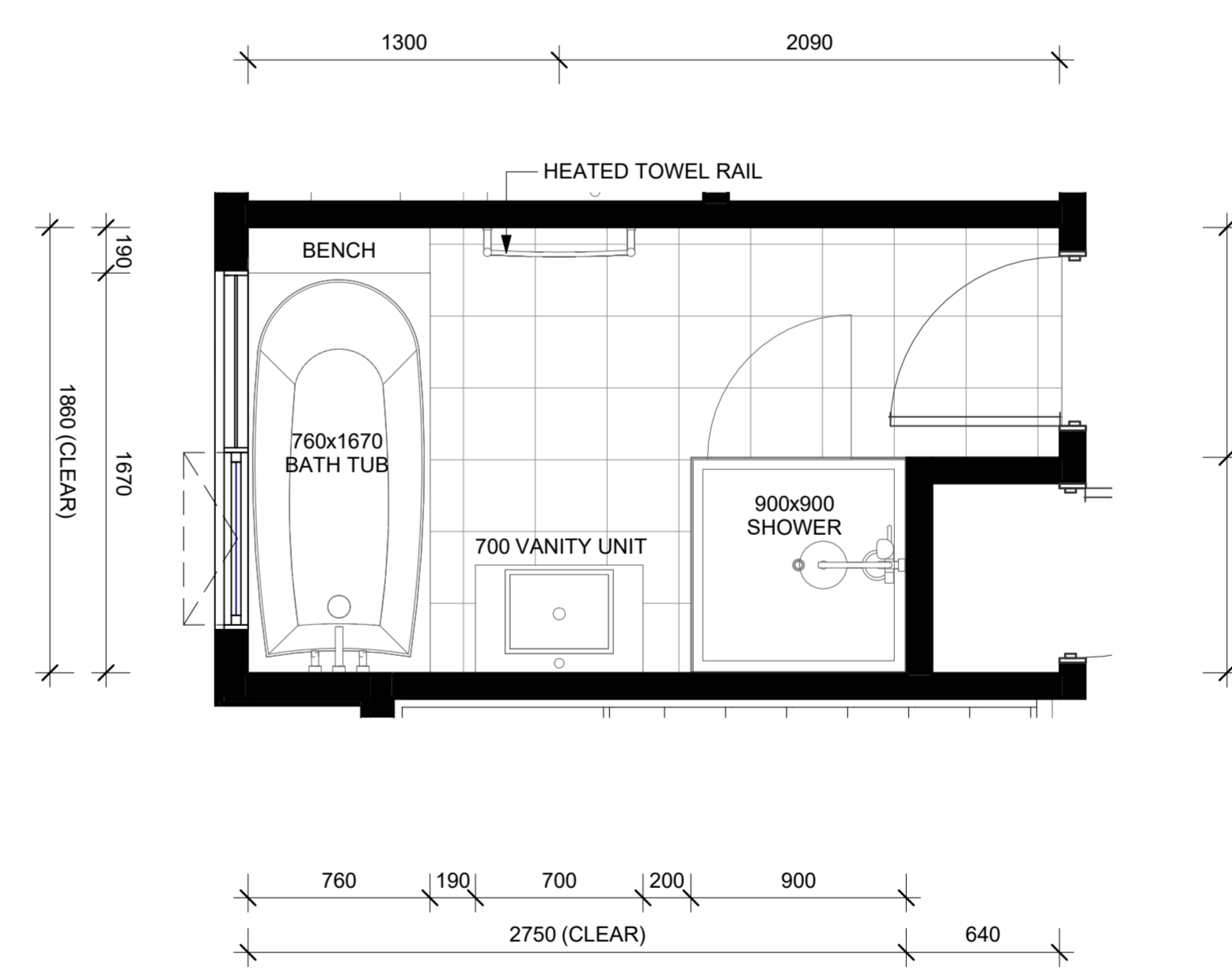
LOT 75 - FIRST FLOOR BATHROOM LAYOUT
