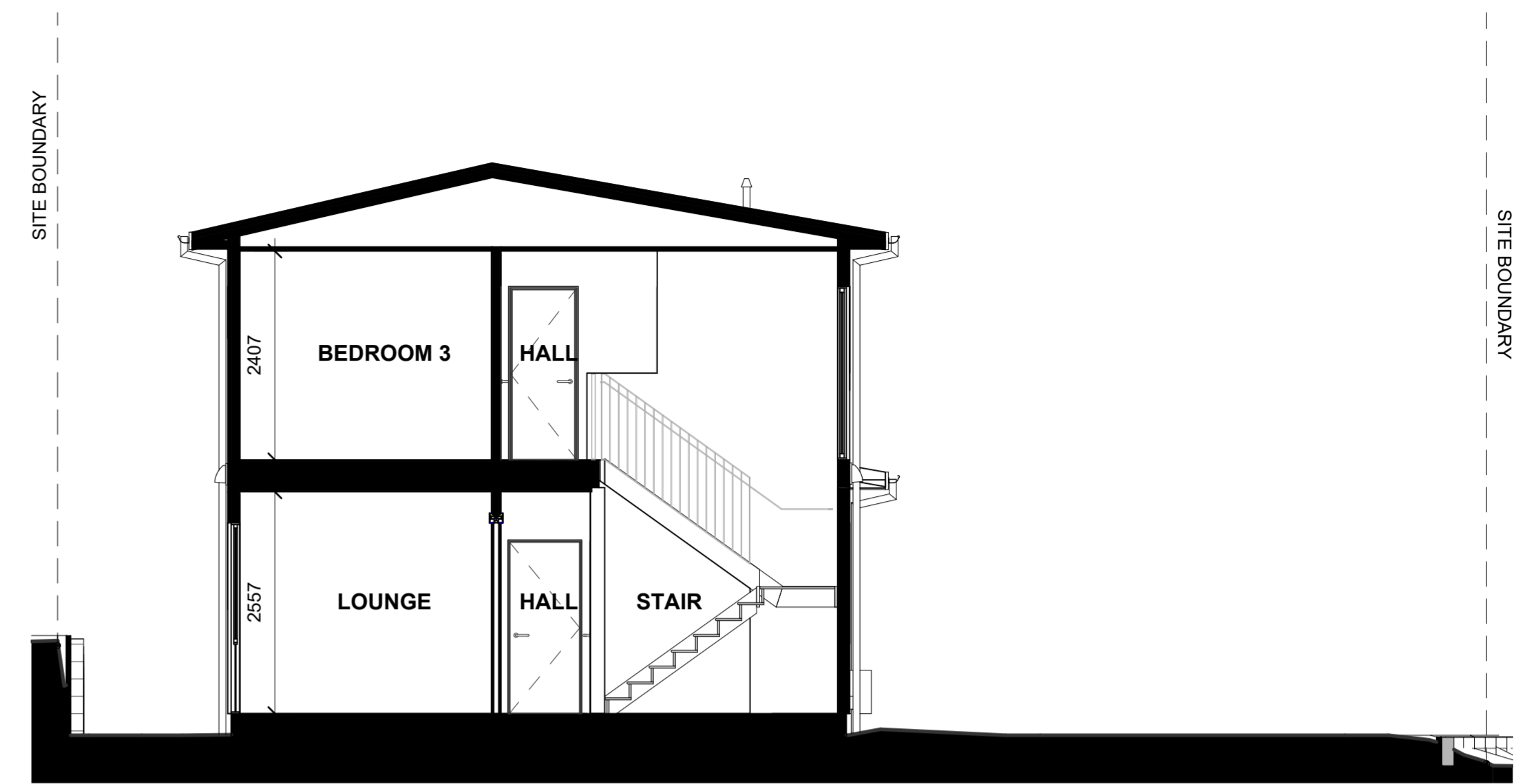
LOT 75 - SECTION B-B
