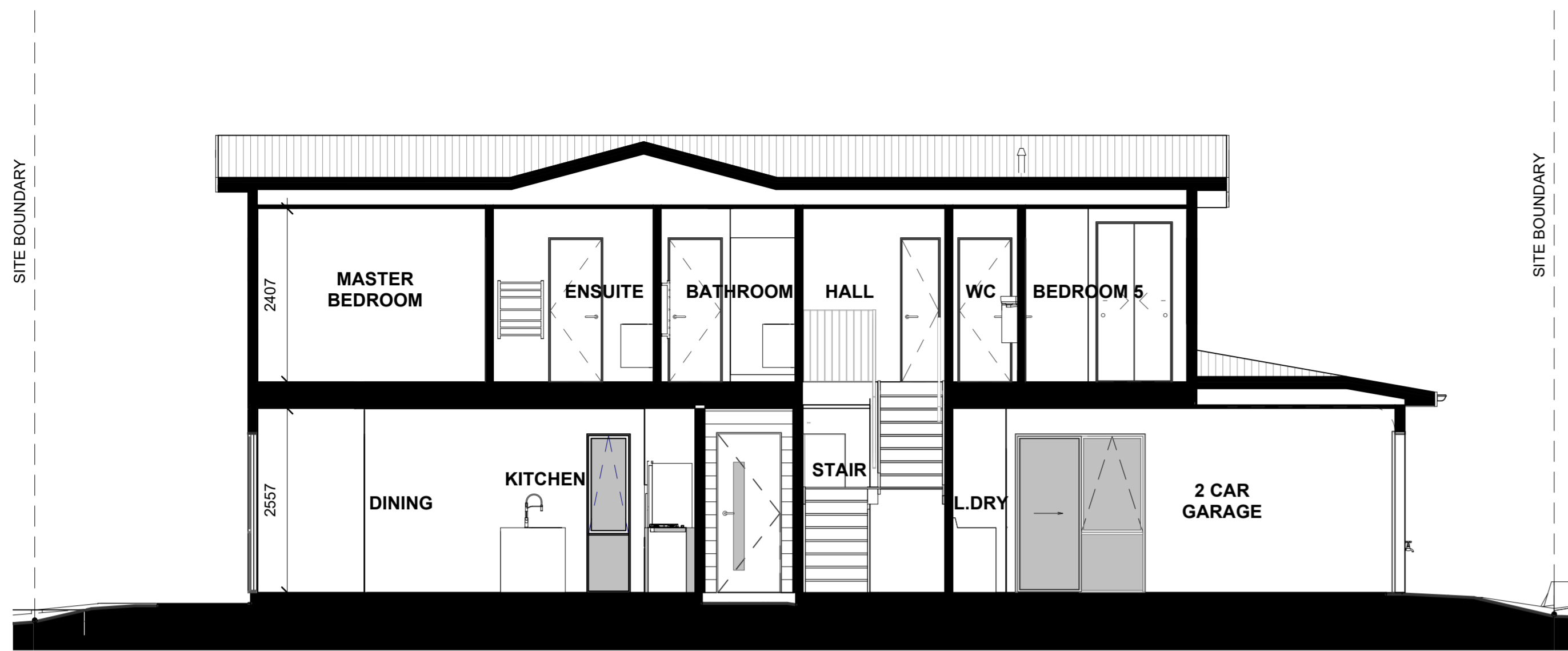
LOT 75 - SECTION A-A
