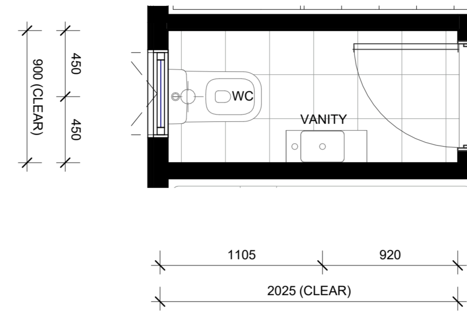
LOT 75 - FIRST FLOOR PLAN WC LAYOUT
