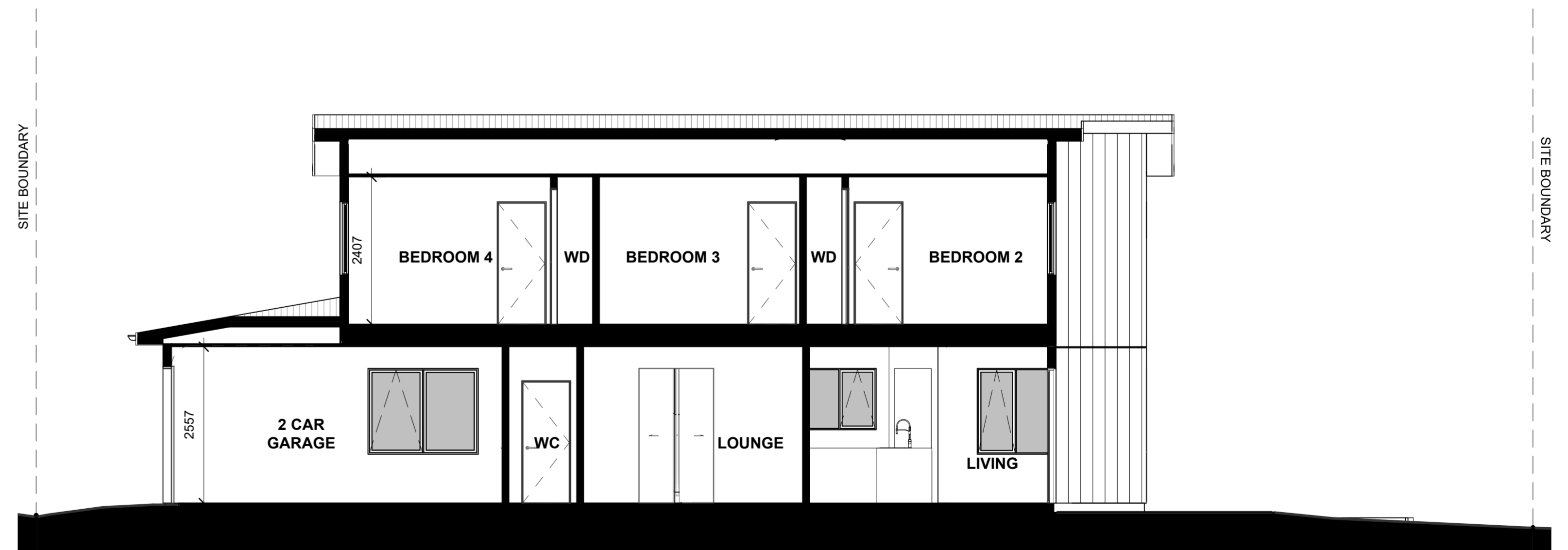
LOT 75 - SECTION D-D
