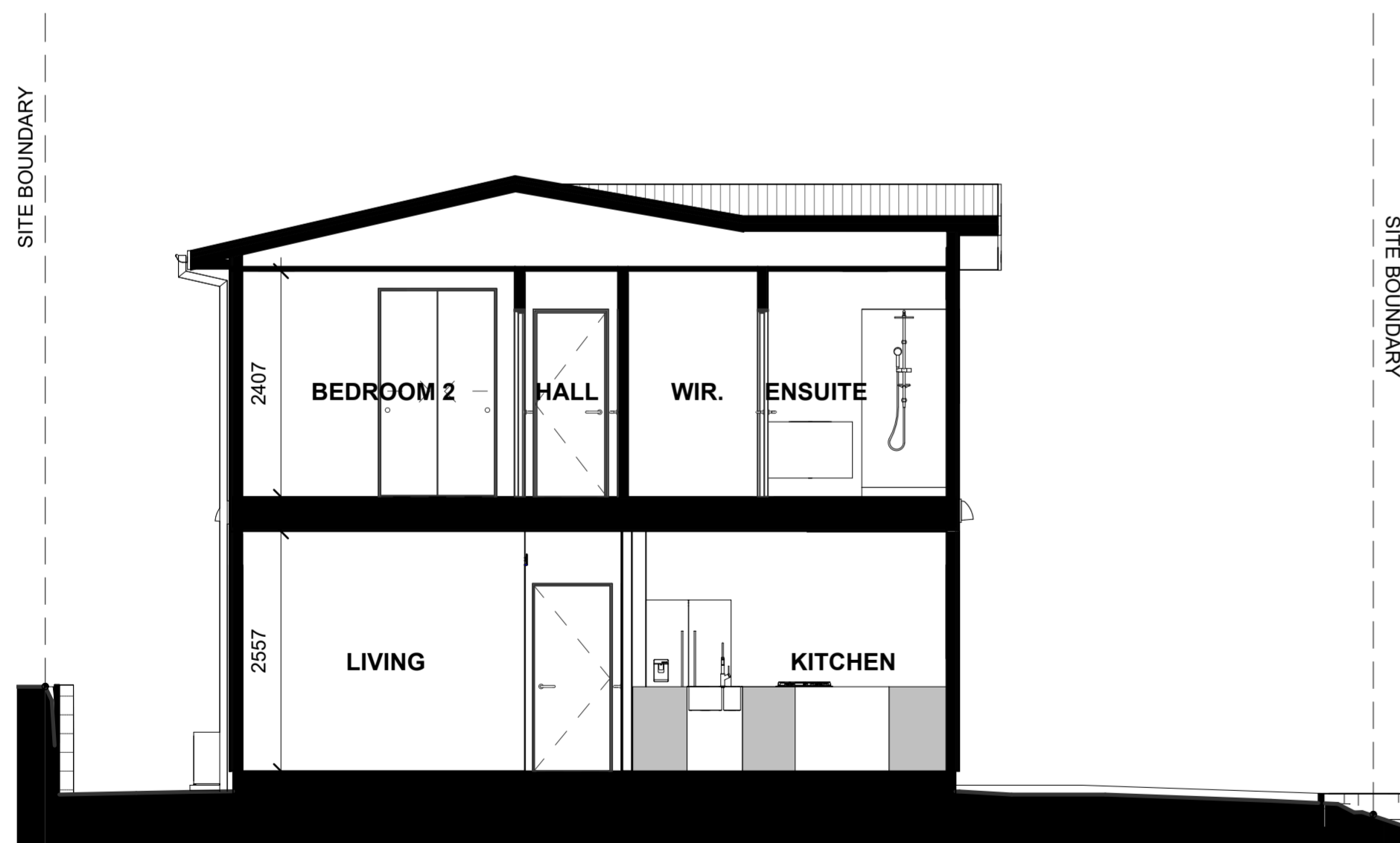
LOT 75 - SECTION C-C
