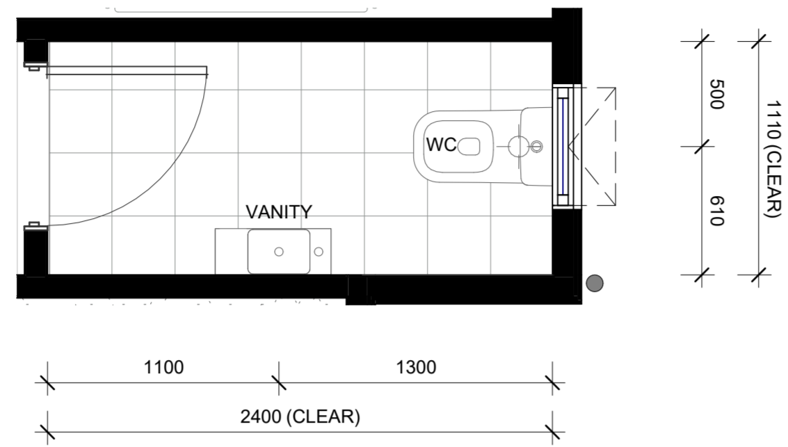
LOT 75 - GROUND FLOOR WC LAYOUT
