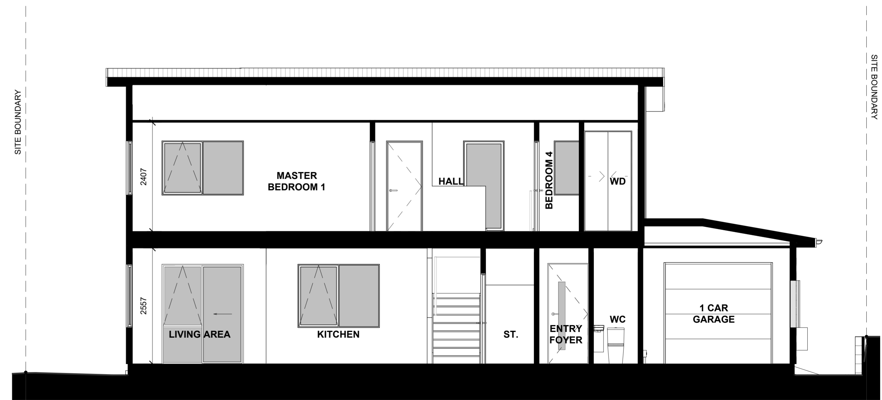
LOT 86 - SECTION D-D
