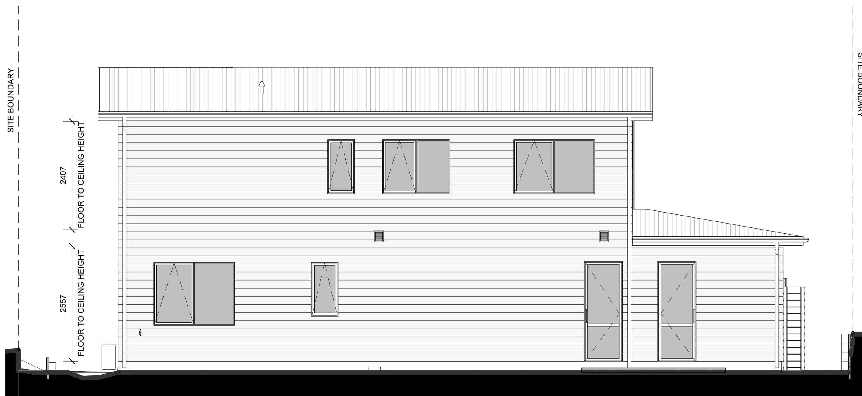
LOT 86 - SOUTH ELEVATION
