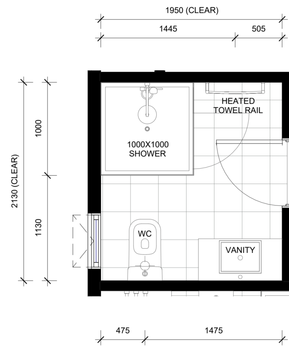
LOT 86 - FIRST FLOOR ENSUITE LAYOUT
