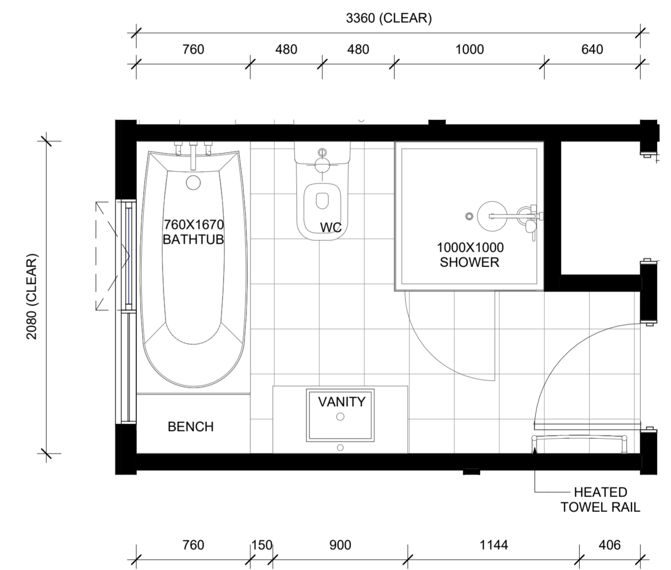
LOT 86 - FIRST FLOOR BATHROOM LAYOUT
