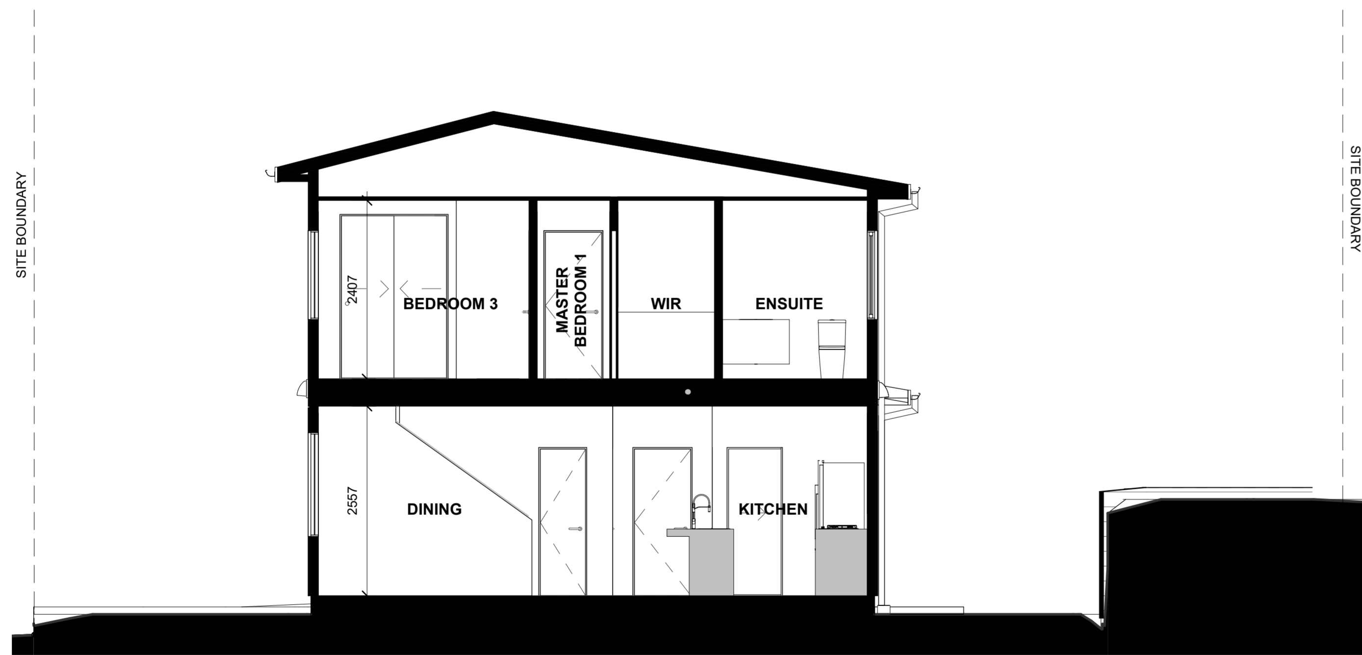
LOT 86 - SECTION C-C
