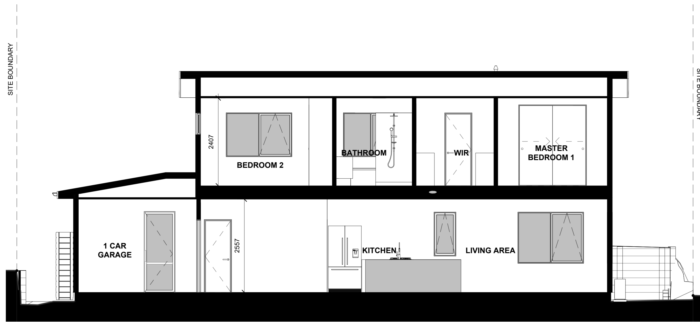
LOT 86 - SECTION A-A
